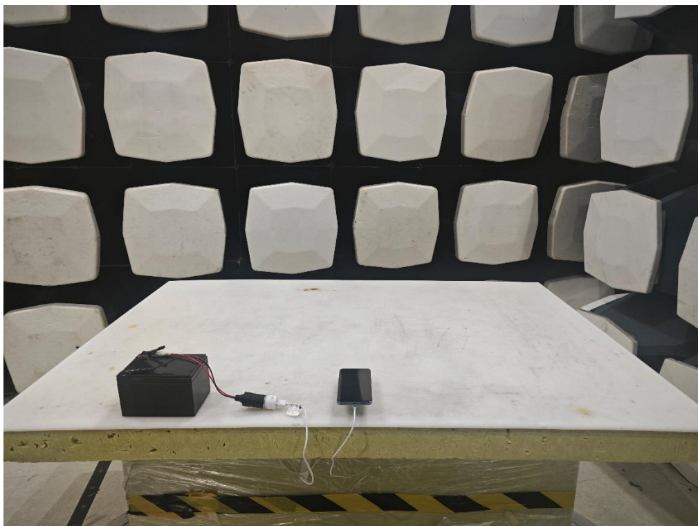
EUT is placed in the center of the turn table
