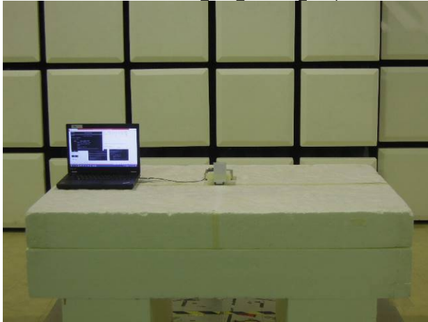
P15.225+RSS210 NFC Radiated Setup
