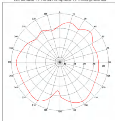
Far-field Power Distribution(H+V) on X-Z Plane Plot Peak Gain(H+V)= 1.68 dB; Plot AvgGain(H+V)= -3.83dB @2.4000 GHz
