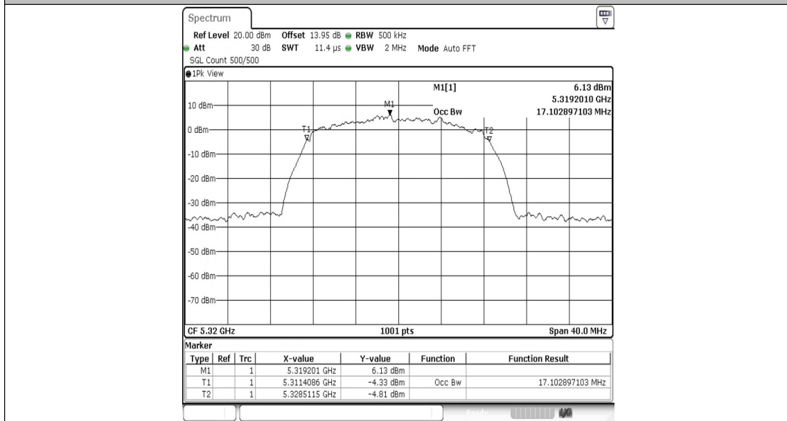
11A-Ant1-5320
