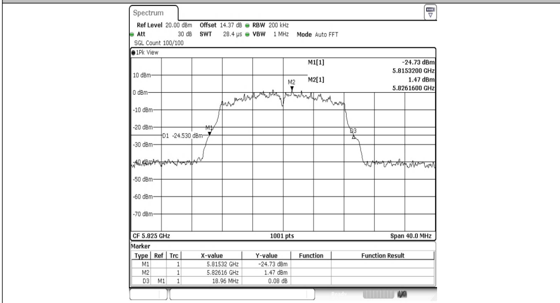
11A-Ant1-5825
