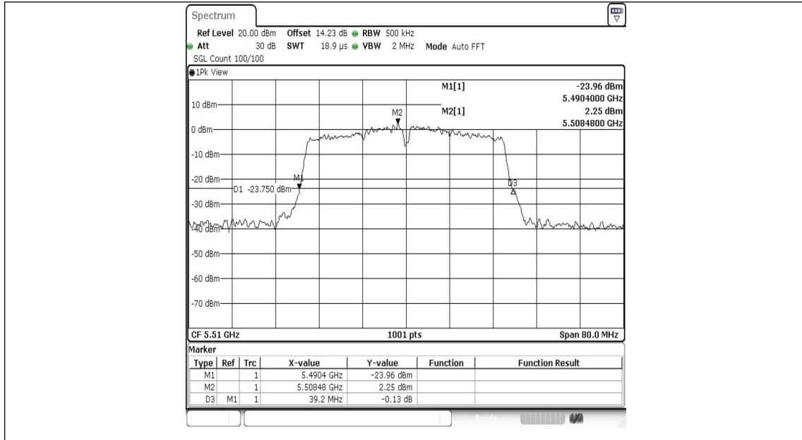
11N40SISO-Ant1-5510
