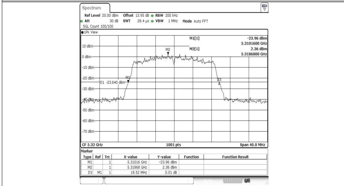
11N20SISO-Ant1-5320
