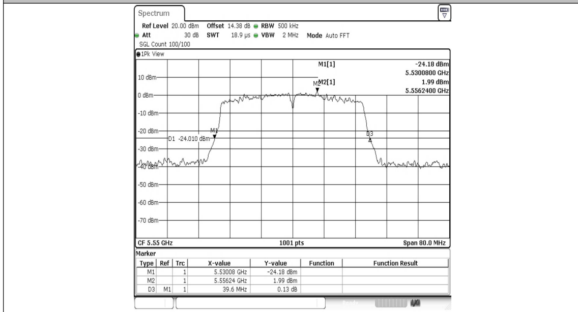
11N40SISO-Ant1-5550
