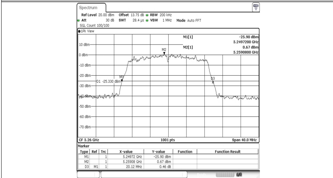
11N20SISO-Ant1-5260
