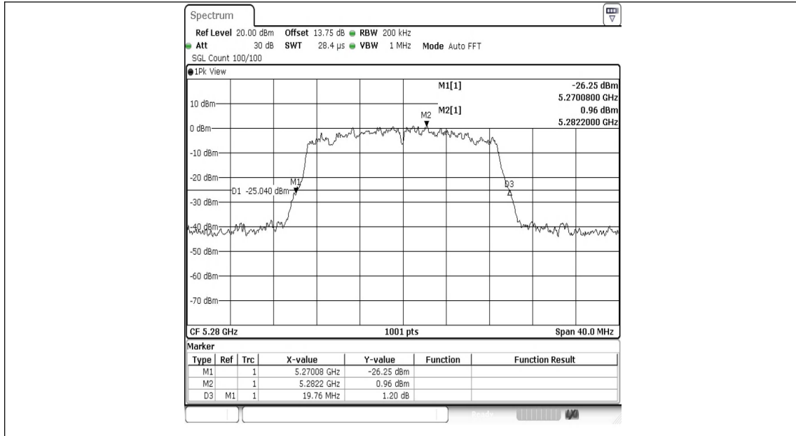
11N20SISO-Ant1-5280
