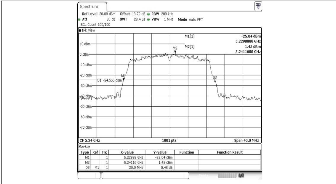
11N20SISO-Ant1-5240
