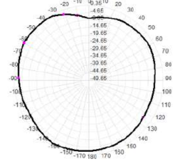
5750.0MHz Total(H), Max=0.35dBi
