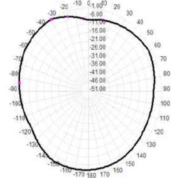
5850.0MHz Total(H), Max=-1.10dBi
