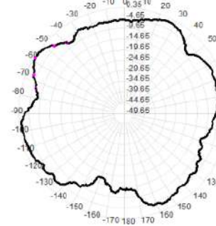
5750.0MHz Total(E2), Max=-0.23dBi
