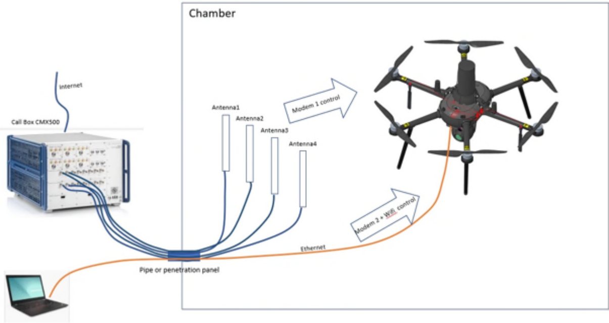
Figure 2. Setup Diagram of Radiated Test with Call Box
