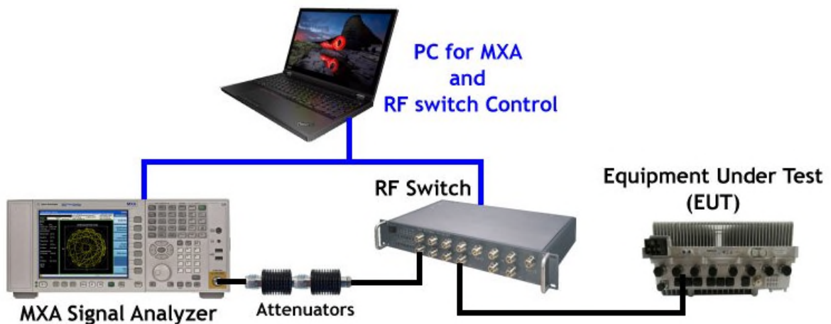
Figure 1. Setup Diagrams of Conducted Test
