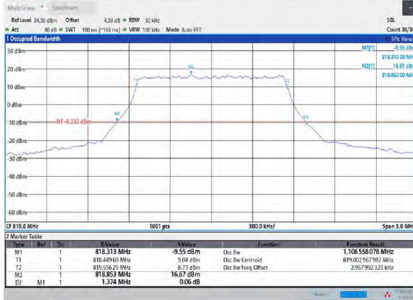
Band26-1.4MHz-QPSK-26740-6RB#0
