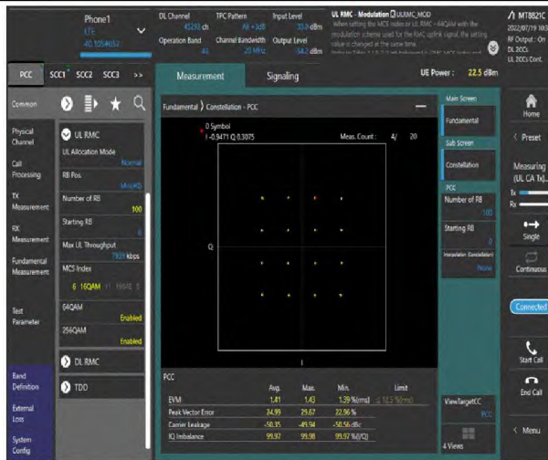
42-42-20MHz-20MHz-16QAM-6QAM-42491-42689-100RB#0-100RB#0
