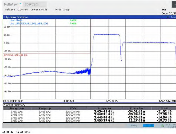
42-42-10MHz-20MHz-QPSK-QPSK-42145-42289-50RB#0-100RB#0
