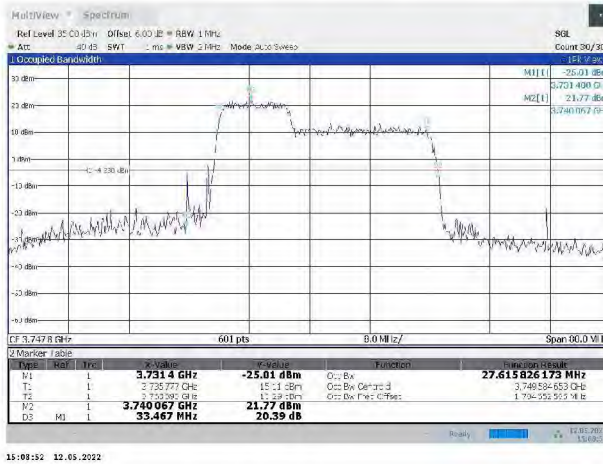
43-43-10MHz-20MHz-QPSK-QPSK-44996-45140-50RB#0-100RB#0
