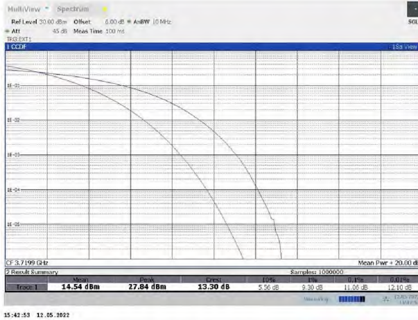
43-43-20MHz-20MHz-QPSK-QPSK-44690-44888-100RB#0-100RB#0
