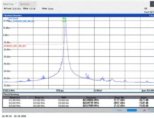
5-5-10MHz-10MHz-QPSK-QPSK-20450-20549-50RB#0-50RB#0
