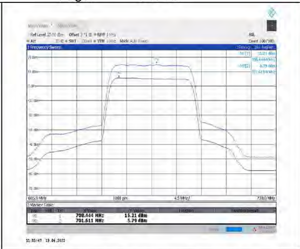
1-N12--15-15-M-2-CP-256QAM-Outer_Full-79@0-Ant1-9.42-100%-0.00-9.42-PASS<=13
