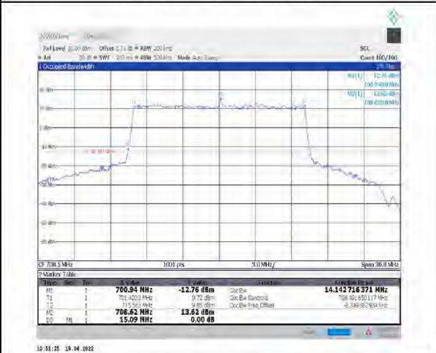
1-N12--15-15-H-8-CP-64QAM-Outer_Full-79@0-Ant1-14.143-15.090-<math>\leq 15</math>-PASS
