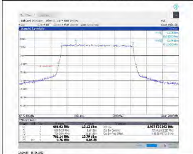
1-N12--15-10-L-4-DFT-64QAM-Outer_Full-50@0-Ant1-8.938-9.760-<math>\leq 10</math>-PASS
