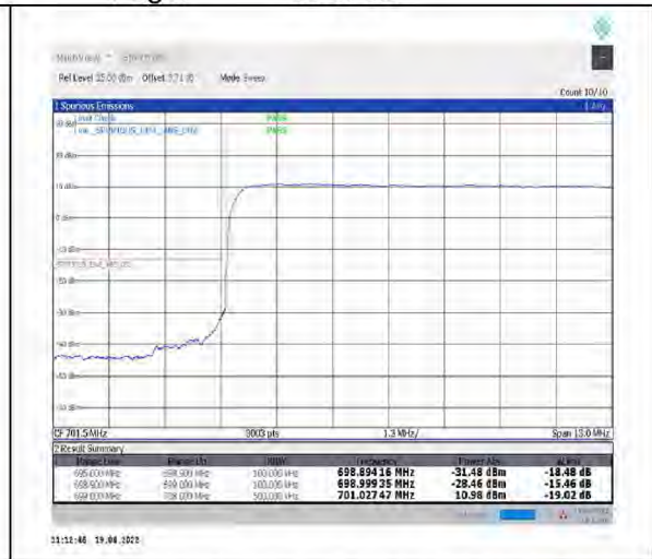
1-N12--15-10-L-3-DFT-PI2BPSK-Outer_Full-50@0-Ant1-PASS-see graph
