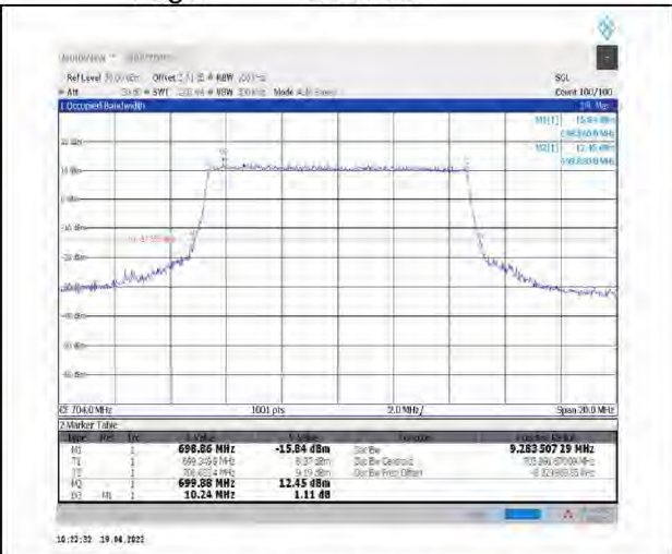
1-N12--15-10-L-7-CP-16QAM-Outer_Full-52@0-Ant1-9,284-10.240-<=10-PASS
