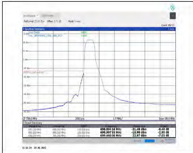
1-N12--15-10-L-1-DFT-PI2BPSK-Edge_1RB_Left-1@0-Ant1-PASS-see graph
