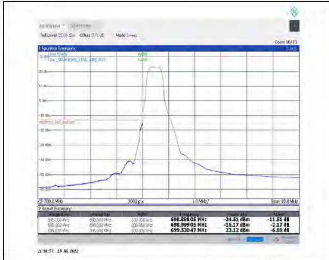
1-N12--15-15-L-1-DFT-PI2BPSK-Edge_1RB_Left-1@0-Ant1-PASS-see graph
