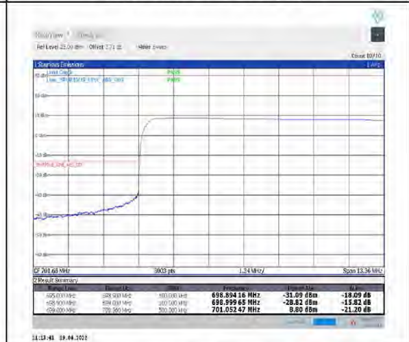
1-N12--15-10-L-6-CP-QPSK-Outer_Full-52@0-Ant1-PASS-see graph
