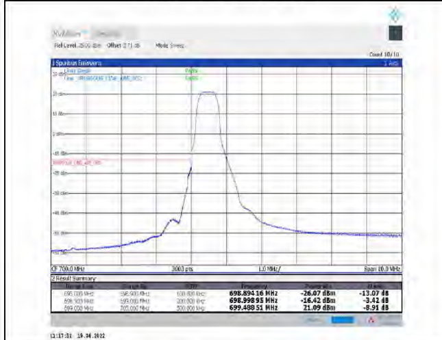
1-N12--15-15-L-4-CP-QPSK-Edge_1RB_Left-1@0-Ant1-PASS-see graph
