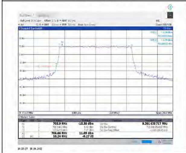
1-N12--15-10-H-6-CP-QPSK-Outer_Full-52@0-Ant1-9.302-10.240-<=10-PASS
