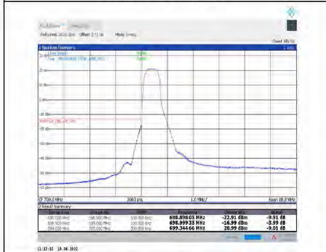
1-N12--15-10-L-4-CP-QPSK-Edge_1RB_Left-1@0-Ant1-PASS-see graph
