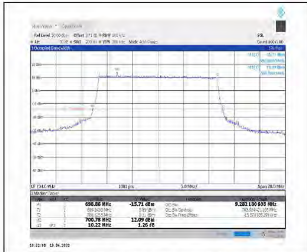
1-N12--15-10-L-6-CP-QPSK-Outer_Full-52@0-Ant1-9,282-10.220-<=10-PASS
