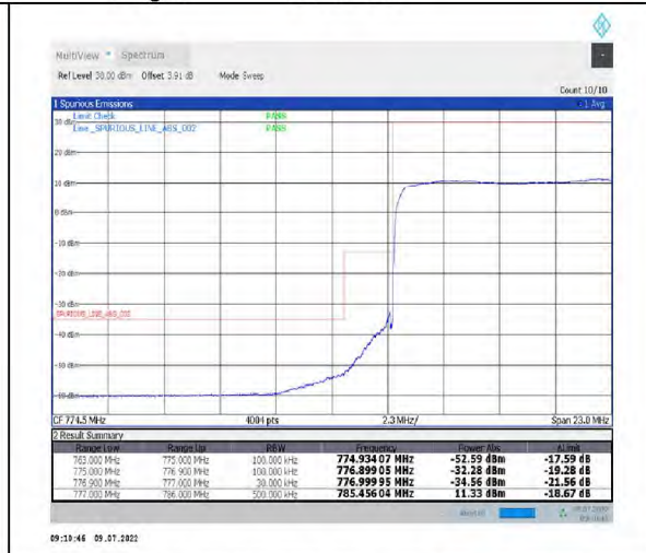
1-N13-PC3-15-10-L-3-DFT-PI2BPSK-Outer_Full-50@0-Ant1-PASS-see graph
