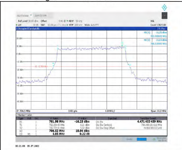
1-N13--15-5-H-8-CP-64QAM-Outer_Full-25@0-Ant1-4.471-5.050-≤5-PASS
