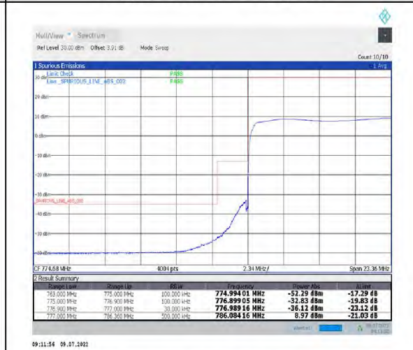
1-N13-PC3-15-10-L-6-CP-QPSK-Outer_Full-52@0-Ant1-PASS-see graph
