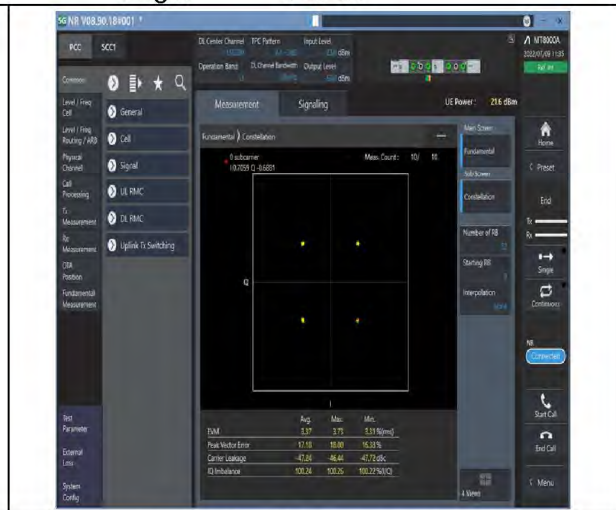
1-N13--15-10-M-6-CP-QPSK-Outer_Full-52@0-Ant1-see graph-PASS
