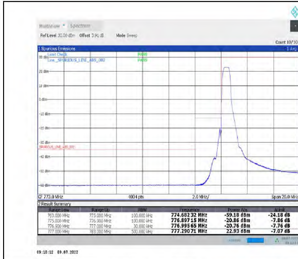
1-N13-PC3-15-10-L-1-DFT-PI2BPSK-Edge_1RB_Left-1@0-Ant1-PASS-see graph
