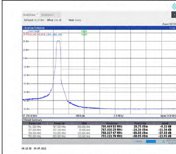
1-N13-PC3-15-10-H-5-CP-QPSK-Edge_1RB_Right-1@51-Ant1-PASS-see graph
