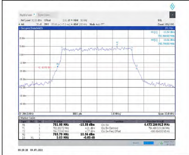
1-N13--15-5-H-5-DFT-256QAM-Outer_Full-25@0-Ant1-4.473-5.050-<math>\leq 5</math>-PASS
