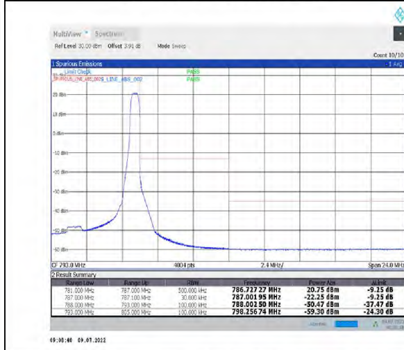
1-N13-PC3-15-5-H-5-CP-QPSK-Edge_1RB_Right-1@24-Ant1-PASS-see graph
