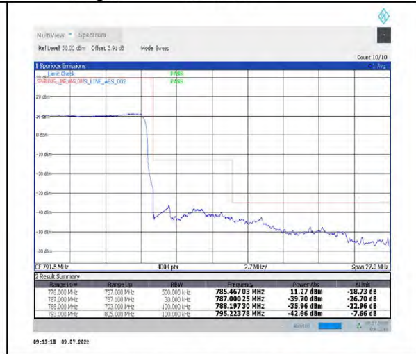
1-N13-PC3-15-10-H-3-DFT-PI2BPSK-Outer_Full-50@0-Ant1-PASS-see graph
