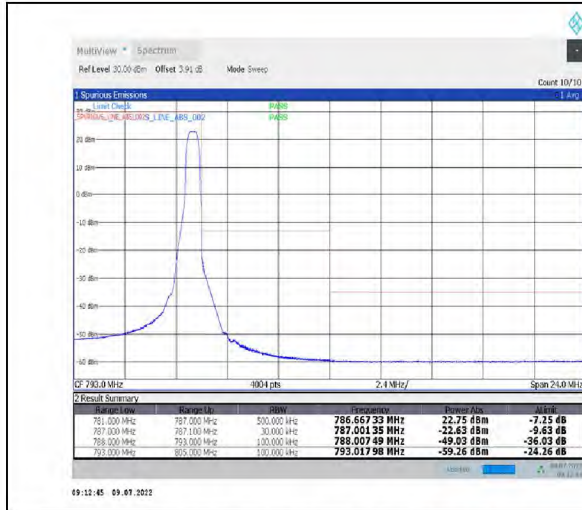
1-N13-PC3-15-10-H-2-DFT-PI2BPSK-Edge_1RB_Right-1@51-Ant1-PASS-see graph
