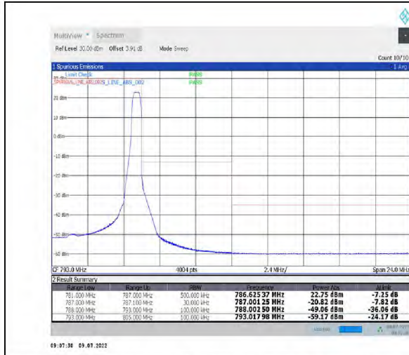
1-N13-PC3-15-5-H-2-DFT-PI2BPSK-Edge_1RB_Right-1@24-Ant1-PASS-see graph
