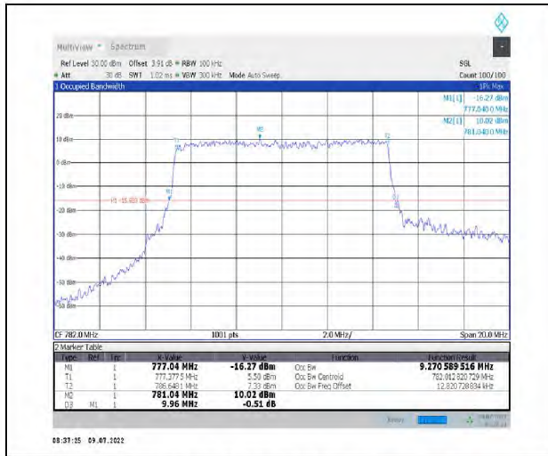
1-N13--15-10-M-6-CP-QPSK-Outer_Full-52@0-Ant1-9.271-9.960-≤10-PASS
