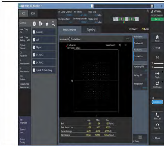
1-N13--15-10-M-5-DFT-256QAM-Outer_Full-50@0-Ant1-see graph-PASS
