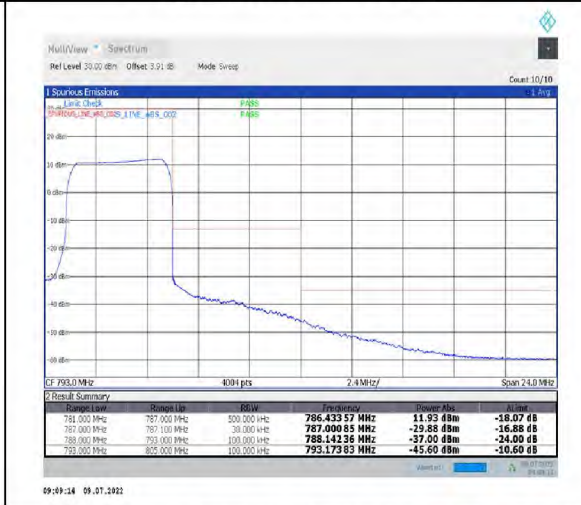
1-N13-PC3-15-5-H-6-CP-QPSK-Outer_Full-25@0-Ant1-PASS-see graph
