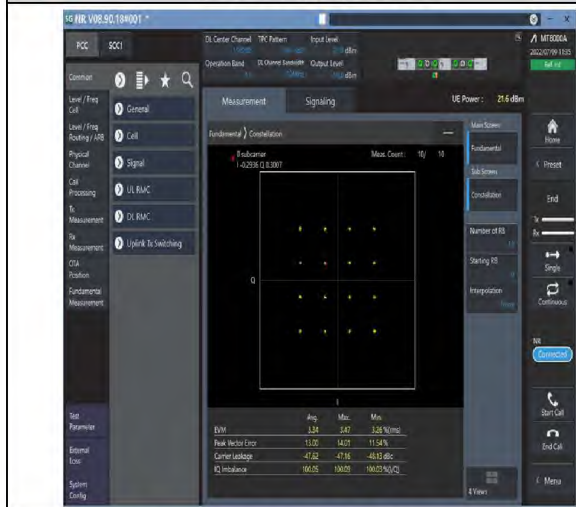
1-N13--15-10-M-7-CP-16QAM-Outer_Full-52@0-Ant1-see graph-PASS
