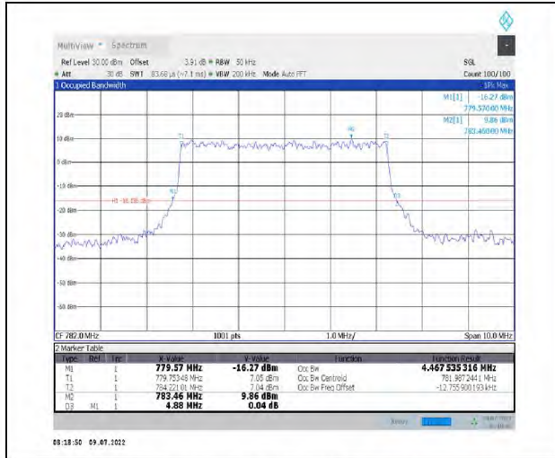
1-N13--15-5-M-8-CP-64QAM-Outer_Full-25@0-Ant1-4.468-4.880-≤5-PASS
