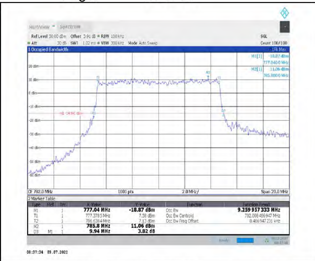
1-N13--15-10-M-7-CP-16QAM-Outer_Full-52@0-Ant1-9.26-9.940-≤10-PASS
