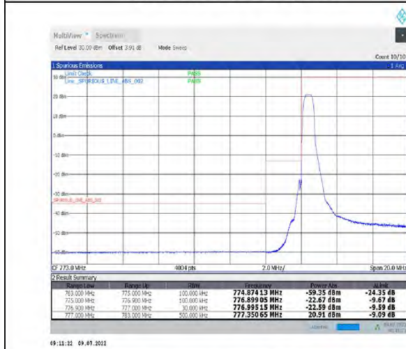
1-N13-PC3-15-10-L-4-CP-QPSK-Edge_1RB_Left-1@0-Ant1-PASS-see graph
