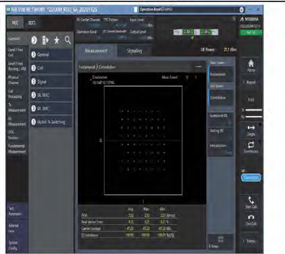
1-N14-PC3-15-10-M-8-CP-64QAM-Outer_Full-52@0-Ant1-see graph-PASS
