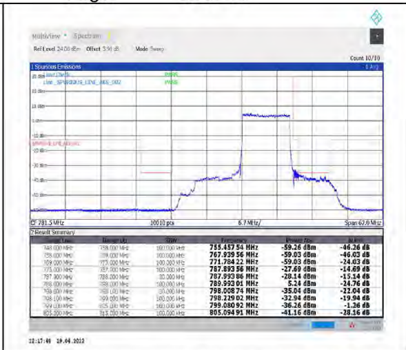
1-N14--15-10-H-3-DFT-PI2BPSK-Outer_Full-50@0-Ant1-PASS-see graph
