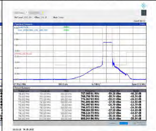
1-N14--15-5-H-6-CP-QPSK-Outer_Full-25@0-Ant1-PASS-see graph
