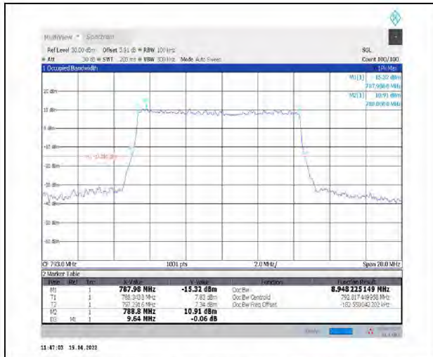
1-N14--15-10-M-5-DFT-256QAM-Outer_Full-50@0-Ant1-8.948-9.640-<=10-PASS
