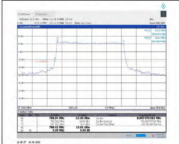
1-N14--15-10-M-3-DFT-16QAM-Outer_Full-50@0-Ant1-8.957-9.580-<=10-PASS
