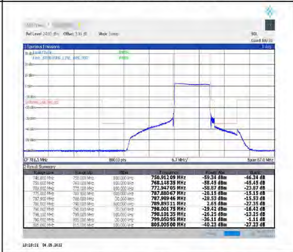
1-N14--15-10-L-6-CP-QPSK-Outer_Full-52@0-Ant1-PASS-see graph
