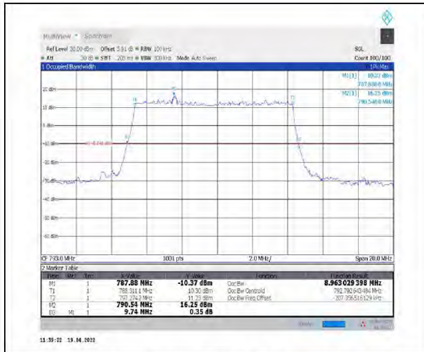
1-N14--15-10-L-2-DFT-PI2BPSK-Outer_Full-50@0-Ant1-8.963-9.740-<=10-PASS
