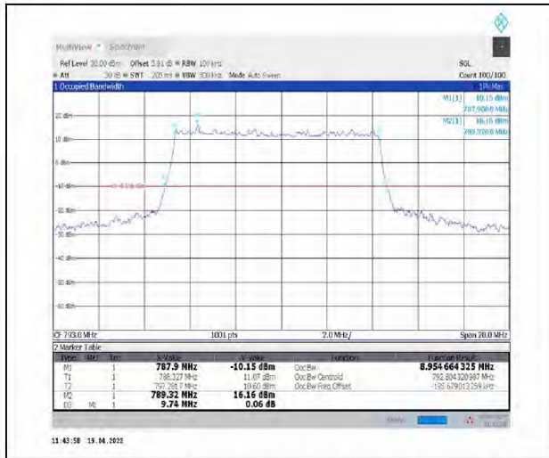
1-N14--15-10-M-1-DFT-QPSK-Outer_Full-50@0-Ant1-8.955-9.740-<=10-PASS
