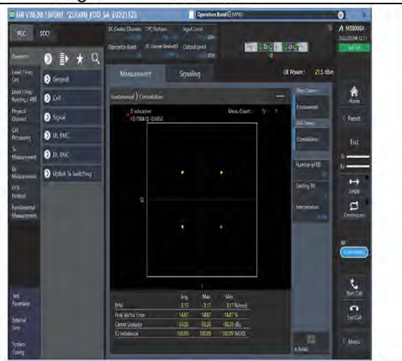
1-N14-PC3-15-10-M-6-CP-QPSK-Outer_Full-52@0-Ant1-see graph-PASS
