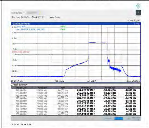
1-N14--15-10-H-6-CP-QPSK-Outer_Full-52@0-Ant1-PASS-see graph
