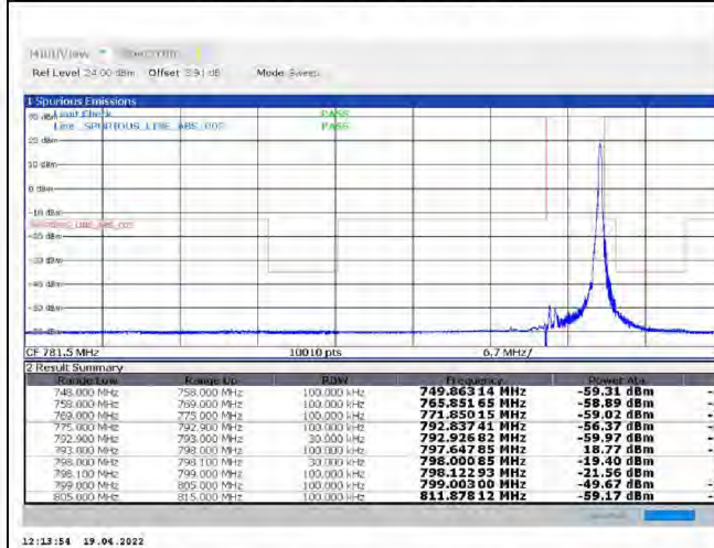
1-N14--15-5-H-5-CP-QPSK-Edge_1RB_Right-1@24-Ant1-PASS-see graph
