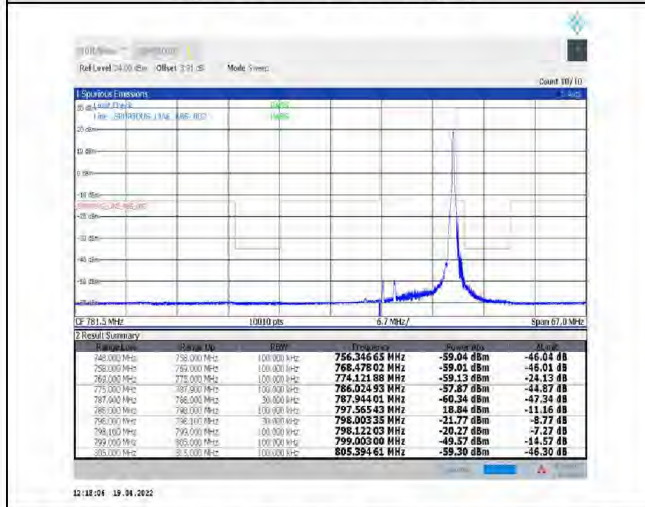
1-N14--15-10-H-5-CP-QPSK-Edge_1RB_Right-1@51-Ant1-PASS-see graph
