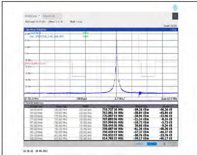
1-N14--15-10-L-1-DFT-PI2BPSK-Edge_1RB_Left-1@0-Ant1-PASS-see graph
