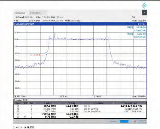
1-N14--15-10-M-4-DFT-64QAM-Outer_Full-50@0-Ant1-8.947-9.780-<=10-PASS
