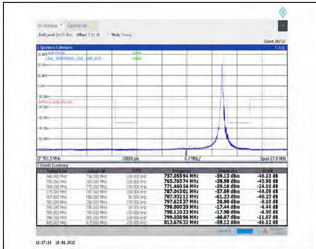
1-N14--15-10-H-2-DFT-PI2BPSK-Edge_1RB_Right-1@51-Ant1-PASS-see graph
