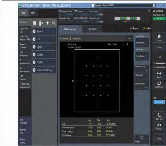
1-N14-PC3-15-10-M-7-CP-16QAM-Outer_Full-52@0-Ant1-see graph-PASS
