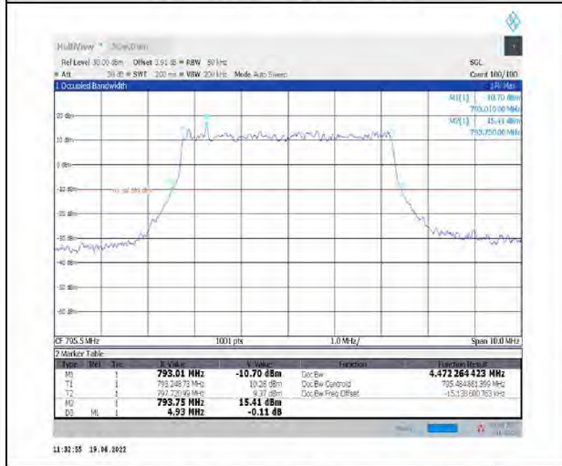
1-N14--15-5-H-1-DFT-QPSK-Outer_Full-25@0-Ant1-4.472-4.930-≤5-PASS
