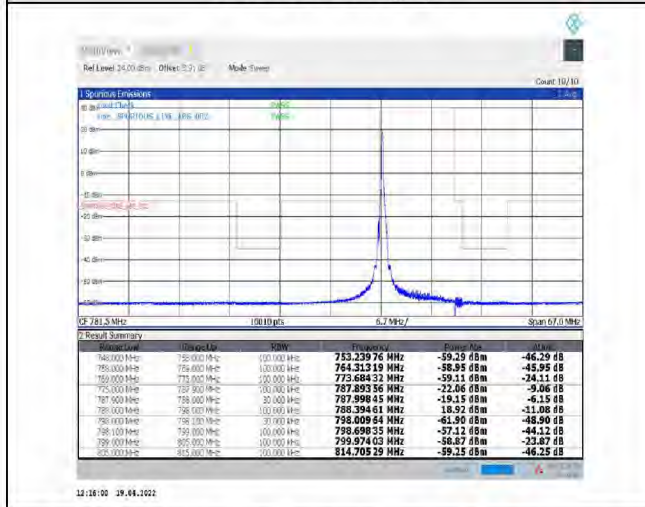
1-N14--15-10-L-4-CP-QPSK-Edge_1RB_Left-1@0-Ant1-PASS-see graph
