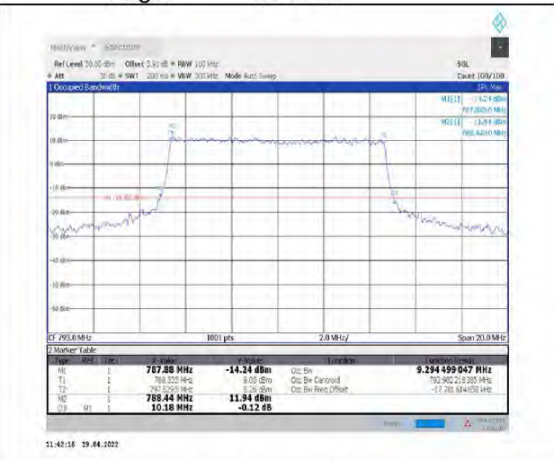
1-N14--15-10-L-7-CP-16QAM-Outer_Full-52@0-Ant1-9.294-10.180-≤10-PASS
