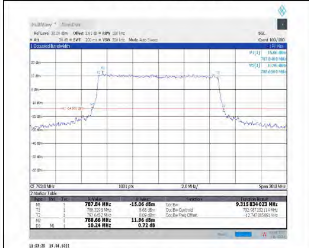
1-N14--15-10-H-6-CP-QPSK-Outer_Full-52@0-Ant1-9.316-10.240-<=10-PASS
