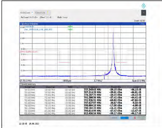
1-N14--15-5-H-2-DFT-PI2BPSK-Edge_1RB_Right-1@24-Ant1-PASS-see graph
