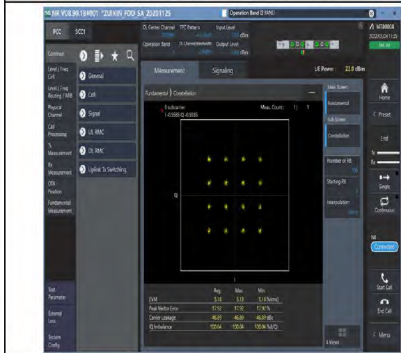
1-N2-PC3-15-20-M-7-CP-16QAM-Outer_Full-106@0-Ant1-see graph-PASS
