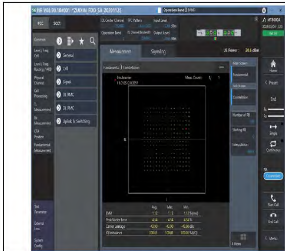
1-N2-PC3-15-20-M-5-DFT-256QAM-Outer_Full-100@0-Ant1-see graph-PASS
