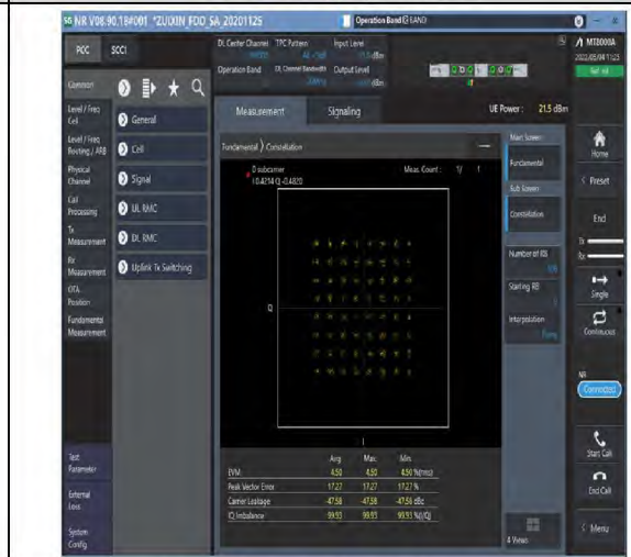
1-N2-PC3-15-20-M-8-CP-64QAM-Outer_Full-106@0-Ant1-see graph-PASS
