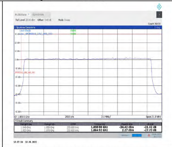
1-N2--15-20-L-3-DFT-PI2BPSK-Outer_Full-100@0-Ant1-seegraph-PASS-see graph
