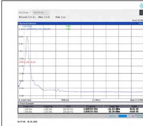
1-N2--15-20-L-1-DFT-PI2BPSK-Edge_1RB_Left-1@0-Ant1-seegraph-PASS-see graph
