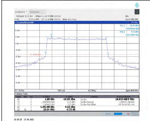
1-N2--15-20-H-8-CP-64QAM-Outer_Full-106@0-Ant1-18.923-20.040-<=20-PASS
