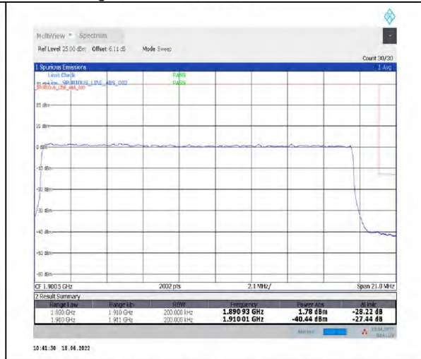
1-N2--15-20-H-3-DFT-PI2BPSK-Outer_Full-100@0-Ant1-seegraph-PASS-see graph
