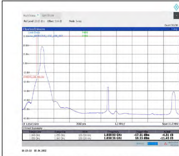
1-N2--15-10-L-1-DFT-PI2BPSK-Edge_1RB_Left-1@0-Ant1-seegraph-PASS-see graph
