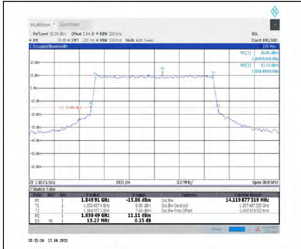
1-N2--15-15-L-7-CP-16QAM-Outer_Full-79@0-Ant1-14.12-15.270-≤15-PASS
