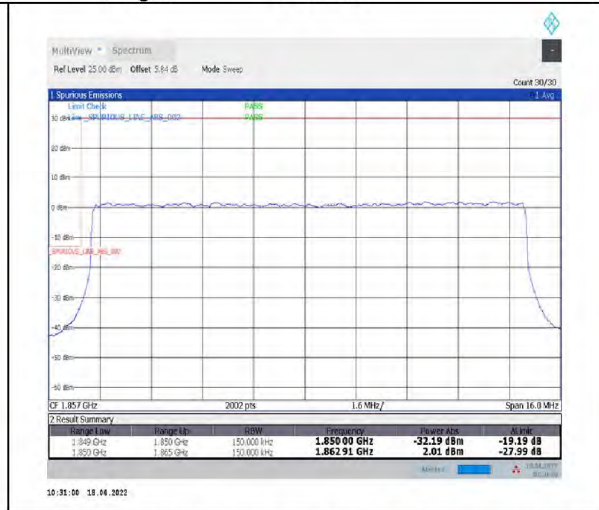
1-N2--15-15-L-3-DFT-PI2BPSK-Outer_Full-75@0-Ant1-seegraph-PASS-see graph
