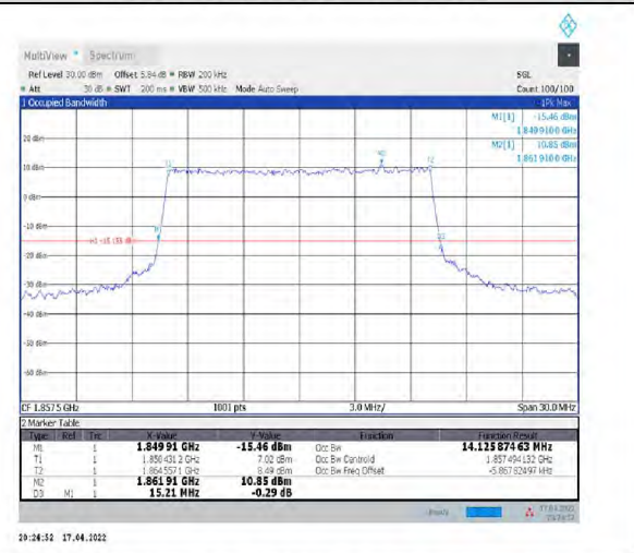
1-N2--15-15-L-6-CP-QPSK-Outer_Full-79@0-Ant1-14.126-15.210-<=15-PASS
