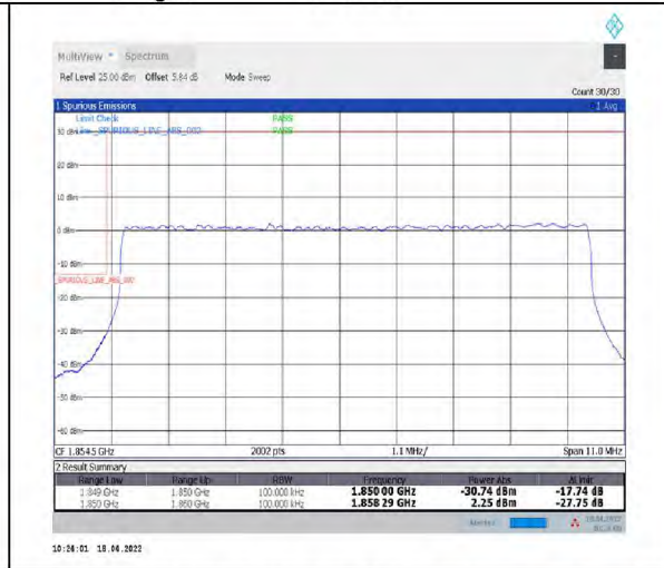
1-N2--15-10-L-3-DFT-PI2BPSK-Outer_Full-50@0-Ant1-seegraph-PASS-see graph
