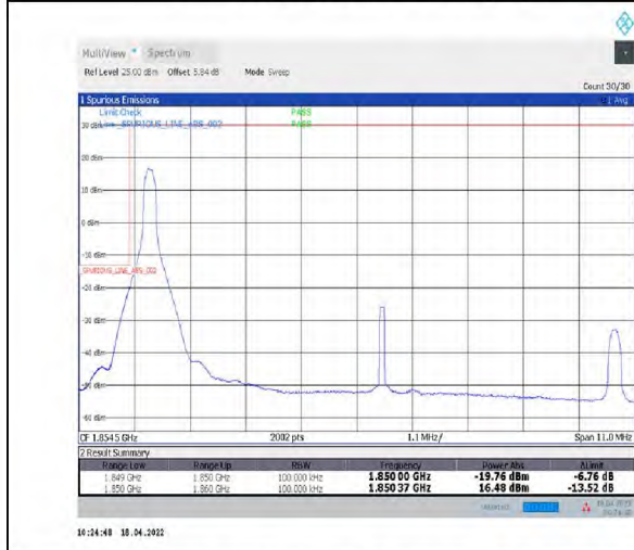
1-N2--15-10-L-4-CP-QPSK-Edge_1RB_Left-1@0-Ant1-seegraph-PASS-see graph
