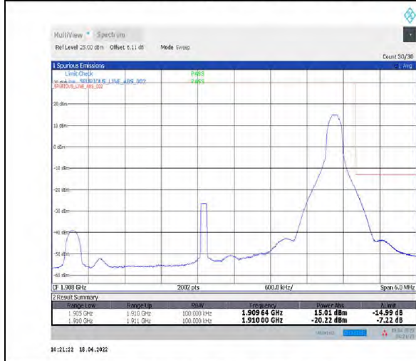
1-N2--15-5-H-5-CP-QPSK-Edge_1RB_Right-1@24-Ant1-seegraph-PASS-see graph
