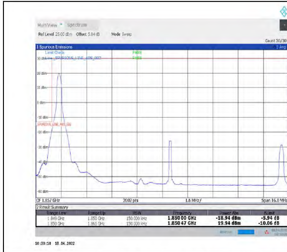
1-N2--15-15-L-1-DFT-PI2BPSK-Edge_1RB_Left-1@0-Ant1-seegraph-PASS-see graph
