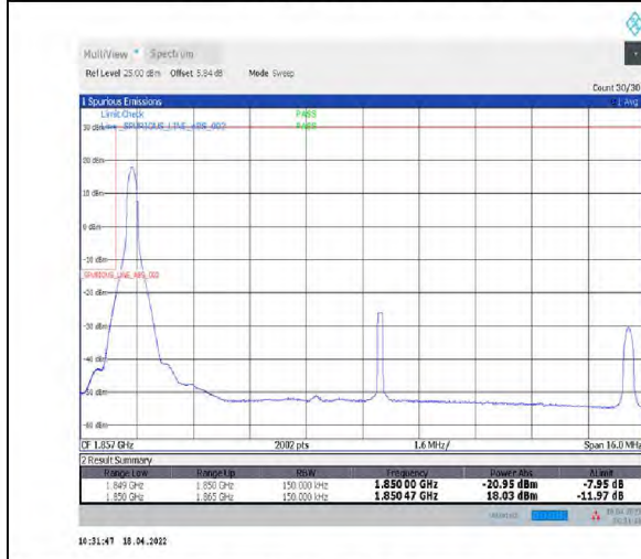
1-N2--15-15-L-4-CP-QPSK-Edge_1RB_Left-1@0-Ant1-seegraph-PASS-see graph
