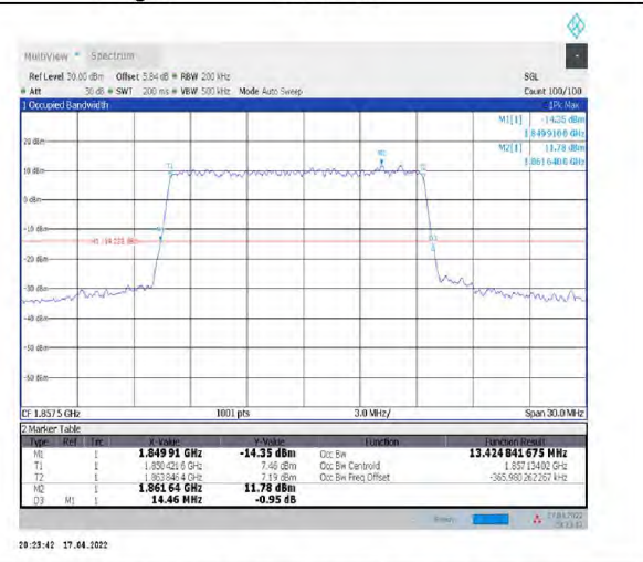
1-N2--15-15-L-4-DFT-64QAM-Outer_Full-75@0-Ant1-13.425-14.460-<=15-PASS
