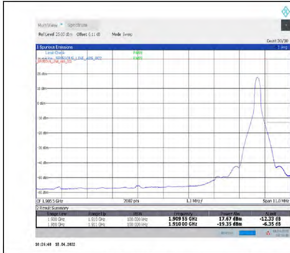
1-N2--15-10-H-2-DFT-PI2BPSK-Edge_1RB_Right-1@51-Ant1-seegraph-PASS-see graph
