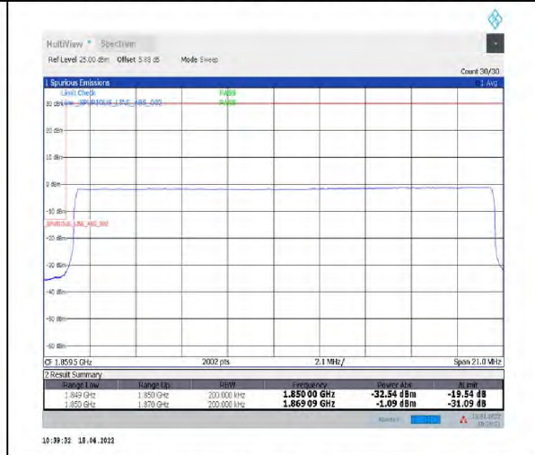
1-N2--15-20-L-6-CP-QPSK-Outer_Full-106@0-Ant1-seegraph-PASS-see graph
