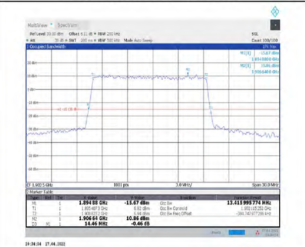
1-N2--15-15-H-4-DFT-64QAM-Outer_Full-75@0-Ant1-13.416-14.460-≤15-PASS
