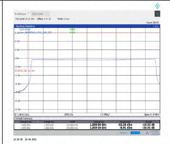
1-N2--15-10-L-6-CP-QPSK-Outer_Full-52@0-Ant1-seegraph-PASS-see graph
