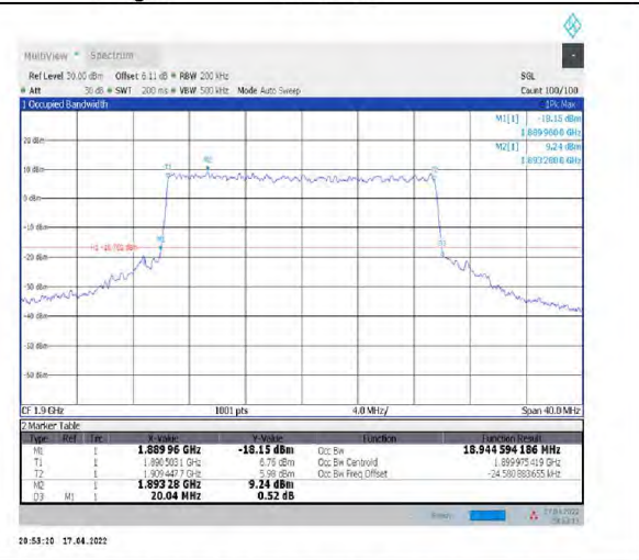
1-N2--15-20-H-7-CP-16QAM-Outer_Full-106@0-Ant1-18.945-20.040-<=20-PASS
