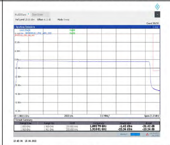
1-N2--15-20-H-6-CP-QPSK-Outer_Full-106@0-Ant1-seegraph-PASS-see graph
