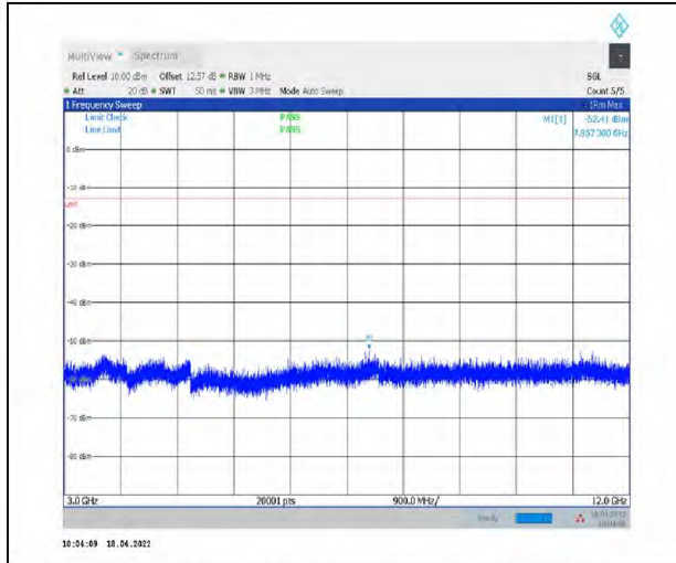
1-N2--15-20-H-1-DFT-PI2BPSK-Inner_1RB_Left- 1@1-3000-12000-Ant1--52.41--13-PASS
