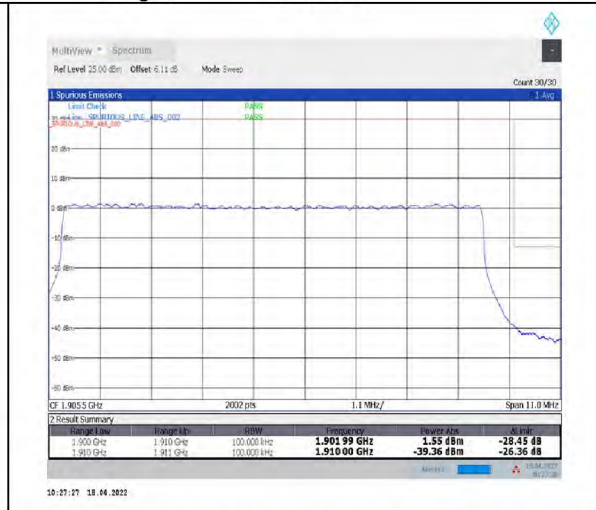
1-N2--15-10-H-3-DFT-PI2BPSK-Outer_Full-50@0-Ant1-seegraph-PASS-see graph
