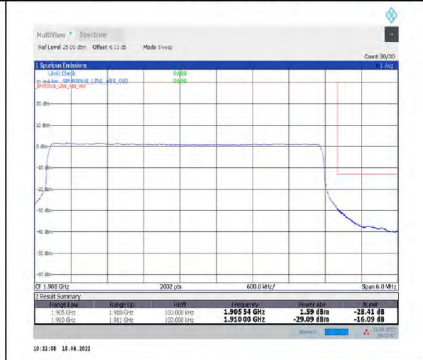
1-N2--15-5-H-6-CP-QPSK-Outer_Full-25@0-Ant1-seegraph-PASS-see graph
