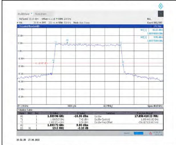
1-N2--15-20-H-4-DFT-64QAM-Outer_Full-100@0-Ant1-17.856-19.000-<20-PASS
