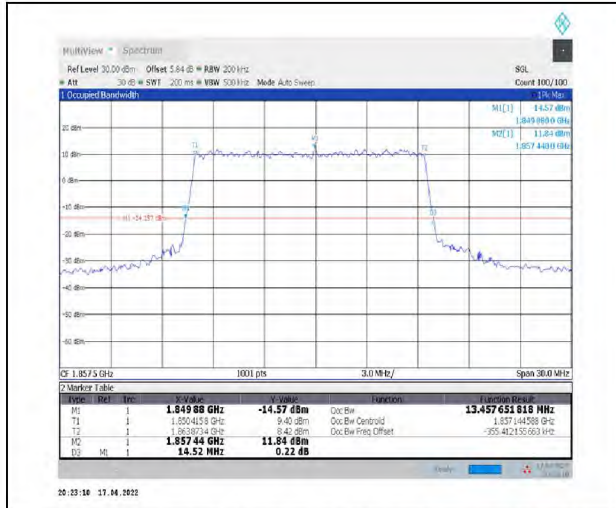
1-N2--15-15-L-3-DFT-16QAM-Outer_Full-75@0-Ant1-13.458-14.520-<=15-PASS
