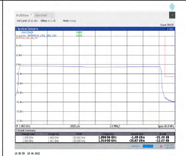
1-N2--15-15-H-6-CP-QPSK-Outer_Full-79@0-Ant1-seegraph-PASS-see graph
