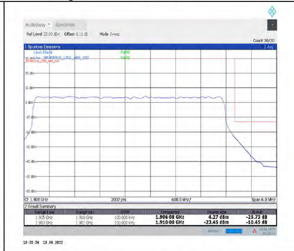
1-N2--15-5-H-3-DFT-PI2BPSK-Outer_Full-25@0-Ant1-seegraph-PASS-see graph
