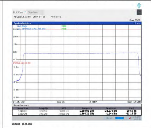
1-N2--15-15-L-6-CP-QPSK-Outer_Full-79@0-Ant1-seegraph-PASS-see graph
