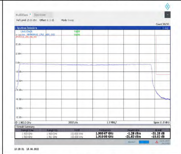
1-N2--15-10-H-6-CP-QPSK-Outer_Full-52@0-Ant1-seegraph-PASS-see graph
