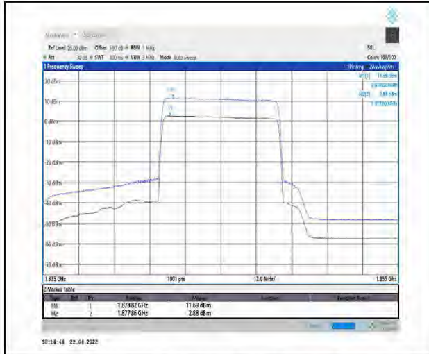
1-N25--15-40-H-1-DFT-256QAM-Outer_Full-216@0-Ant1-8.81-100%-0.00-8.81-PASS-<math>\leq 13</math>
