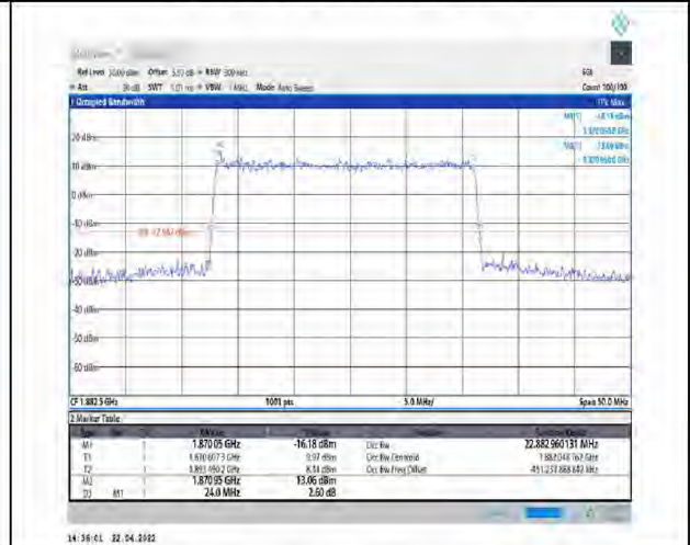
1-N25--15-25-M-3-DFT-16QAM-Outer_Full-128@0-Ant1-22.883-24.000-<=25-PASS
