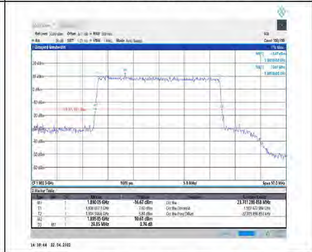
1-N25--15-25-H-6-CP-QPSK-Outer_Full-133@0-Ant1-23.741-24.850-<25-PASS
