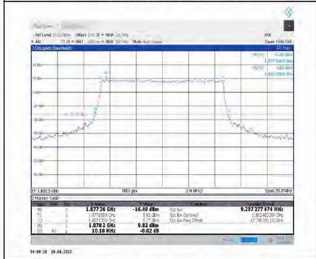
1-N25--15-10-M-7-CP-16QAM-Outer_Full-52@0-Ant1-9.297-10.180-<=10-PASS
