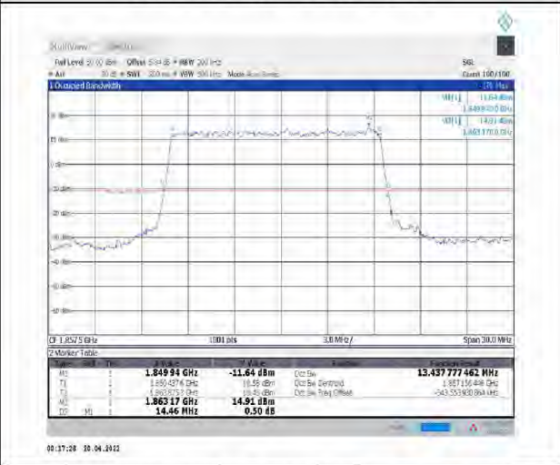
1-N25--15-15-L-2-DFT-PI2BPSK-Outer_Full-75@0-Ant1-13.438-14.460-≤15-PASS
