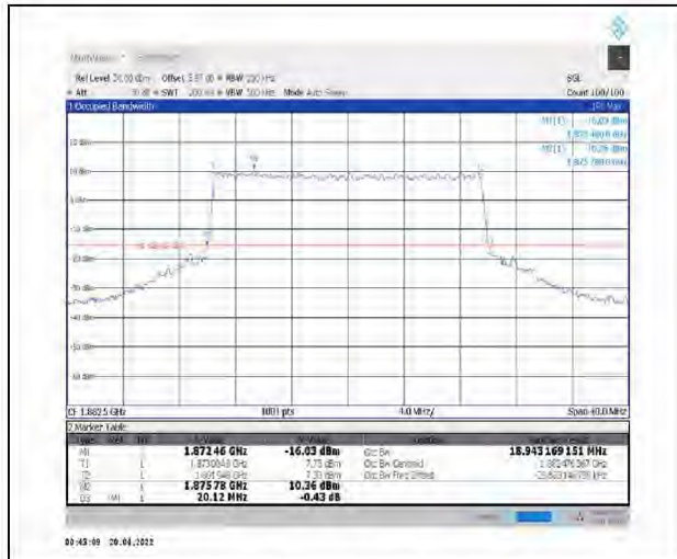
1-N25--15-20-M-7-CP-16QAM-Outer_Full-106@0-Ant1-18.943-20.120-<20-PASS
