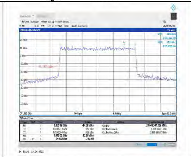
1-N25--15-30-L-3-DFT-16QAM-Outer_Full-160@0-Ant1-28.649-29.640-<30-PASS
