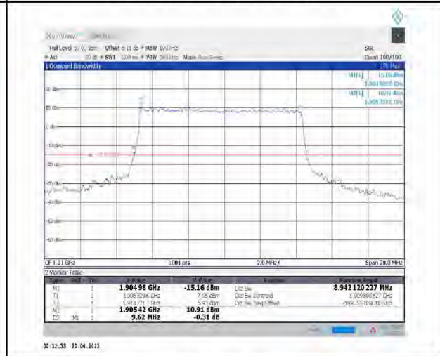
1-N25--15-10-H-3-DFT-16QAM-Outer_Full-50@0-Ant1-8.942-9.620-<=10-PASS
