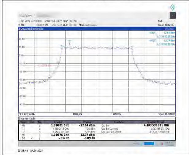
1-N25--15-5-H-1-DFT-QPSK-Outer_Full-25@0-Ant1-4,484-5.000-<math>\leq</math>5-PASS
