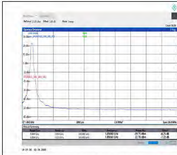
1-N25--15-25-L-1-DFT-PI2BPSK-Edge_1RB_Left-1@0-Ant1-seegraph-PASS-see graph
