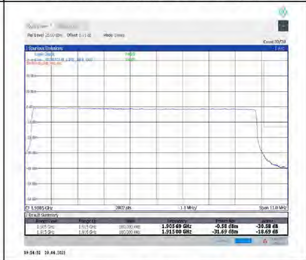
1-N25--15-10-H-6-CP-QPSK-Outer_Full-52@0-Ant1-see graph-PASS-see graph
