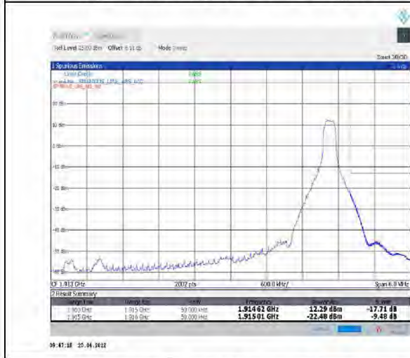
1-N25--15-5-H-5-CP-QPSK-Edge_1RB_Right-1@24-Ant1-seegraph-PASS-see graph
