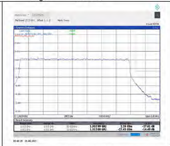
1-N25--15-5-H-3-DFT-PI2BPSK-Outer_Full-25@0-Ant1-seegraph-PASS-see graph
