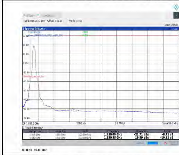
1-N25--15-20-L-4-CP-QPSK-Edge_1RB_Left-1@0-Ant1-seegraph-PASS-see graph
