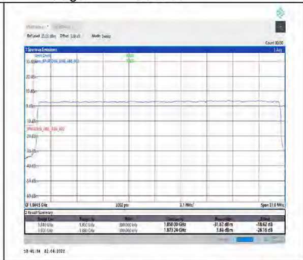
1-N25--15-30-L-3-DFT-PI2BPSK-Outer_Full-160@0-Ant1-seegraph-PASS-see graph
