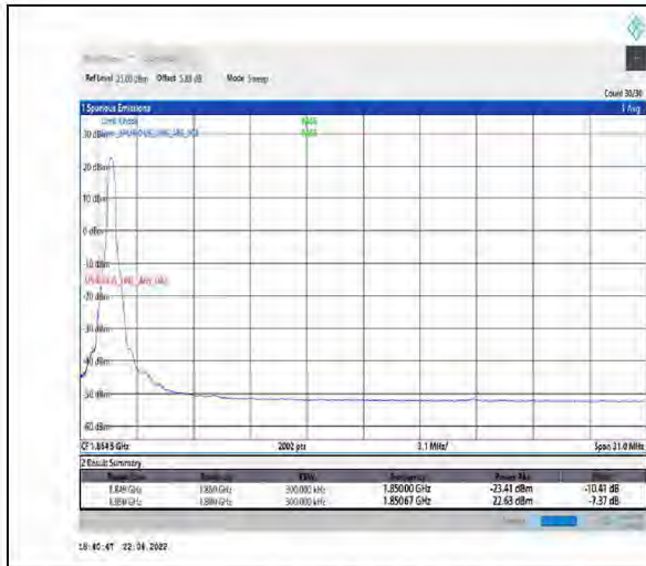
1-N25--15-30-L-1-DFT-PI2BPSK-Edge_1RB_Left-1@0-Ant1-seegraph-PASS-see graph
