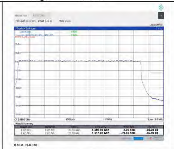
1-N25--15-10-H-3-DFT-PI2BPSK-Outer_Full-50@0-Ant1-see graph-PASS-see graph
