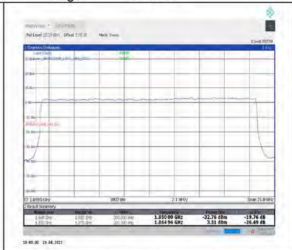
1-N25--15-20-L-3-DFT-PI2BPSK-Outer_Full-100@0-Ant1-seegraph-PASS-see graph
