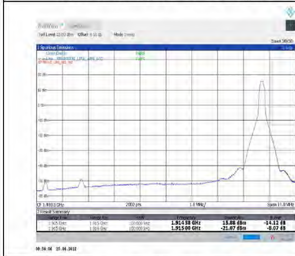
1-N25--15-10-H-5-CP-QPSK-Edge_1RB_Right-1@51-Ant1-see graph-PASS-see graph
