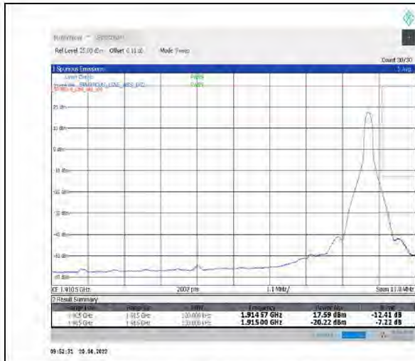
1-N25--15-10-H-2-DFT-PI2BPSK-Edge_1RB_Right-1@51-Ant1-see graph-PASS-see graph
