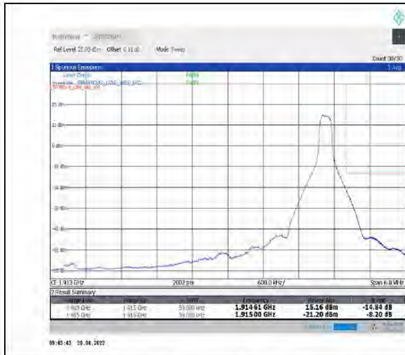
1-N25--15-5-H-2-DFT-PI2BPSK-Edge_1RB_Right-1@24-Ant1-seegraph-PASS-see graph
