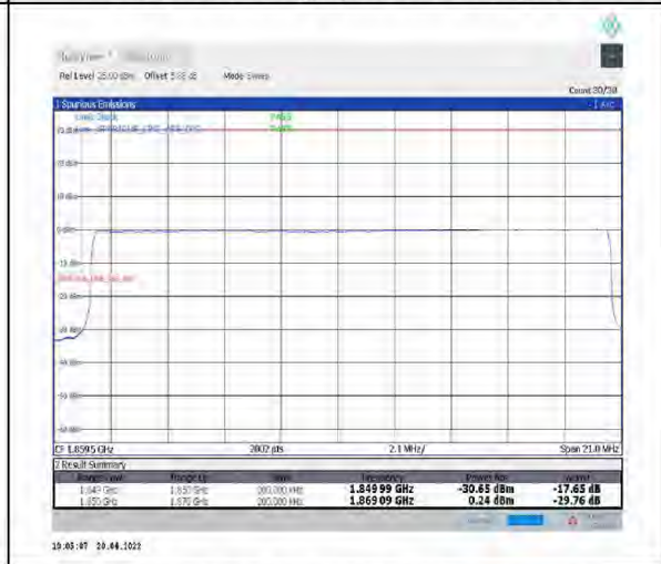
1-N25--15-20-L-6-CP-QPSK-Outer_Full-106@0-Ant1-seegraph-PASS-see graph
