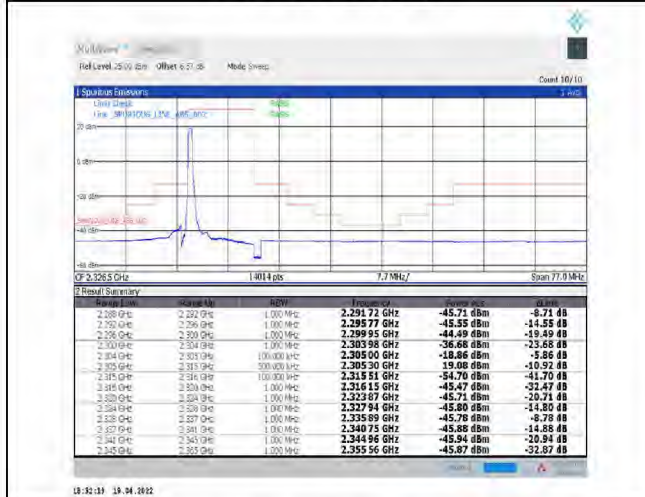
1-N30--30-10-L-4-CP-QPSK-Edge_1RB_Left-1@0-Ant1-PASS-see graph
