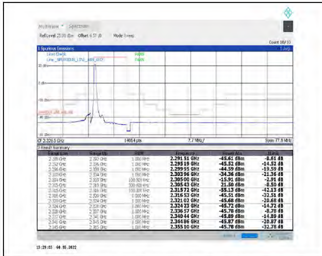
1-N30--15-10-L-1-DFT-PI2BPSK-Edge_1RB_Left-1@0-Ant1-PASS-see graph
