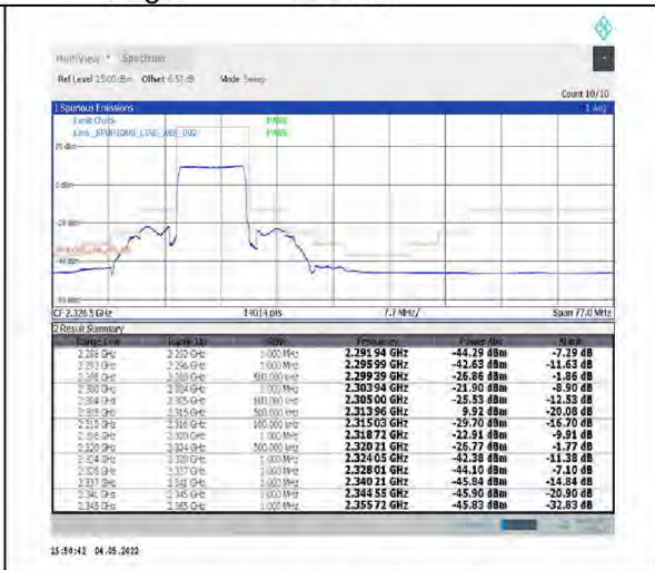
1-N30--15-10-L-3-DFT-PI2BPSK-Outer_Full-50@0-Ant1-PASS-see graph
