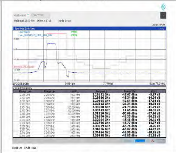
1-N30--30-10-L-3-DFT-PI2BPSK-Outer_Full-24@0-Ant1-PASS-see graph
