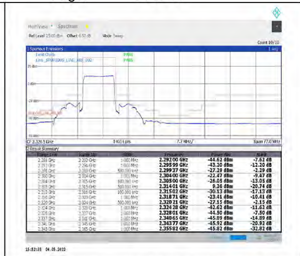
1-N30--15-10-H-3-DFT-PI2BPSK-Outer_Full-50@0-Ant1-PASS-see graph
