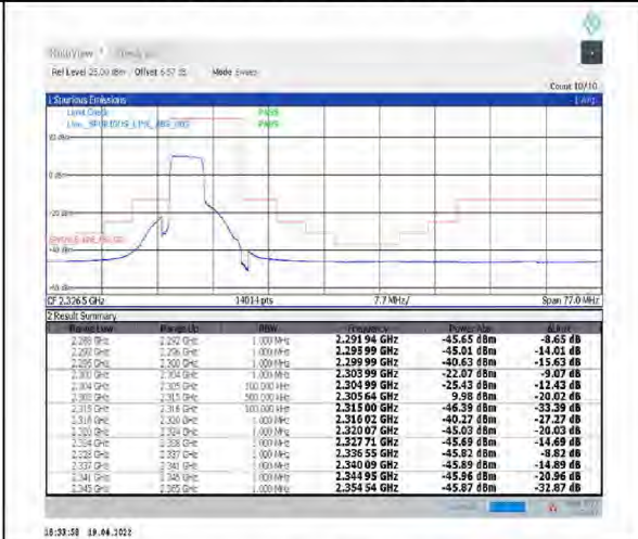
1-N30--30-10-L-6-CP-QPSK-Outer_Full-24@0-Ant1-PASS-see graph
