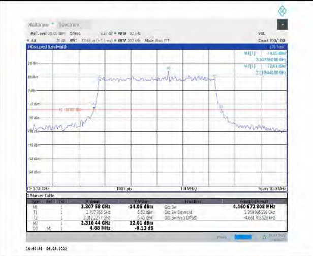
1-N30--15-5-M-3-DFT-16QAM-Outer_Full-25@0-Ant1-4.461-4.880-<math>\leq 5</math>-PASS
