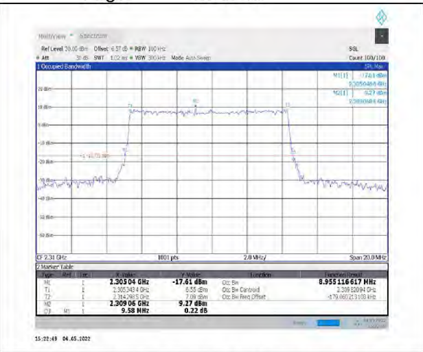
1-N30--15-10-H-5-DFT-256QAM-Outer_Full-50@0-Ant1-8.955-9.580-<=10-PASS
