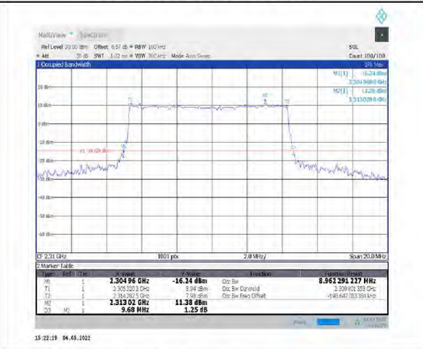
1-N30--15-10-H-3-DFT-16QAM-Outer_Full-50@0-Ant1-8.962-9.680-<=10-PASS
