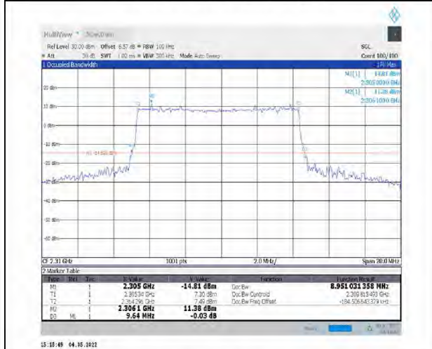
1-N30--15-10-L-4-DFT-64QAM-Outer_Full-50@0-Ant1-8.951-9.640-<math>\leq 10</math>-PASS
