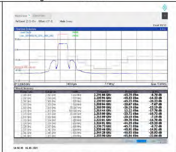
1-N30--15-5-H-3-DFT-PI2BPSK-Outer_Full-25@0-Ant1-PASS-see graph
