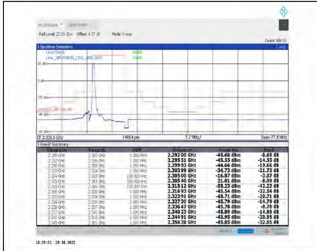
1-N30--30-10-L-1-DFT-PI2BPSK-Edge_1RB_Left-1@0-Ant1-PASS-see graph
