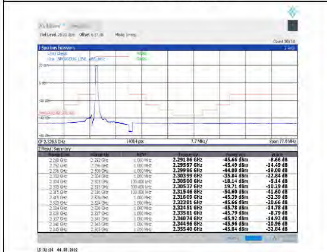
1-N30--15-10-L-4-CP-QPSK-Edge_1RB_Left-1@0-Ant1-PASS-see graph
