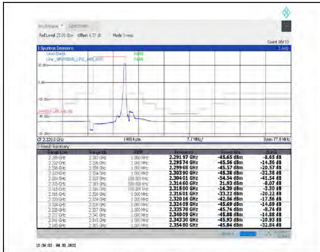
1-N30--15-10-H-2-DFT-PI2BPSK-Edge_1RB_Right-1@51-Ant1-PASS-see graph
