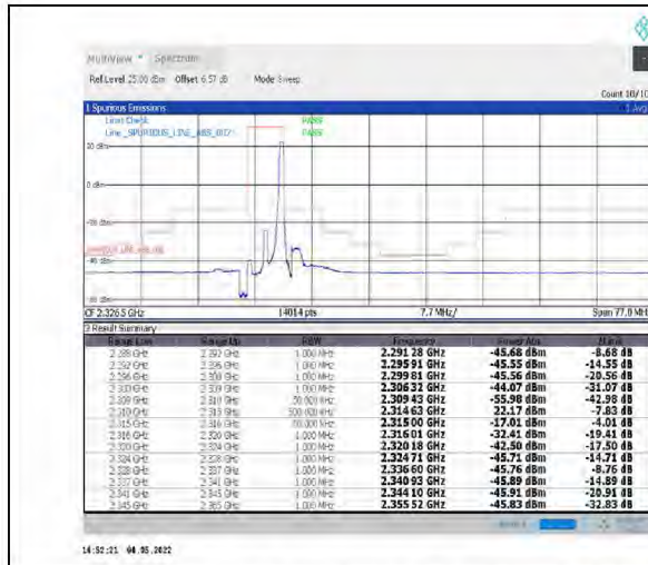
1-N30--15-5-H-2-DFT-PI2BPSK-Edge_1RB_Right-1@24-Ant1-PASS-see graph
