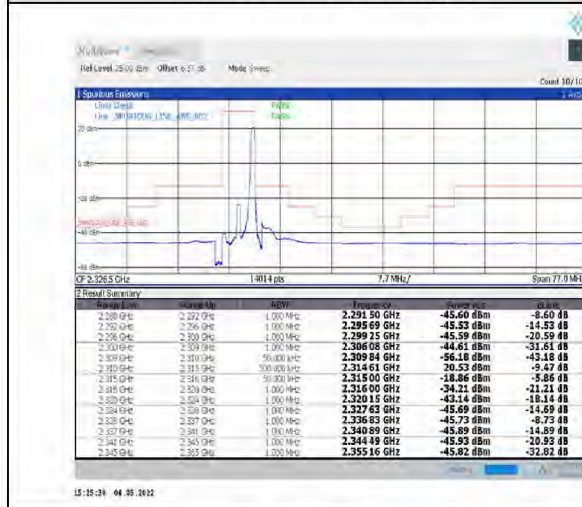
1-N30--15-5-H-5-CP-QPSK-Edge_1RB_Right-1@24-Ant1-PASS-see graph
