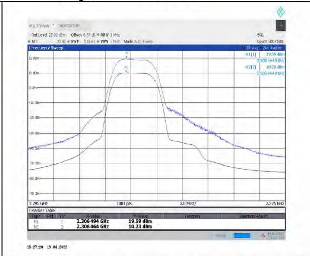
1-N30--15-10-H-2-CP-256QAM-Outer_Full-24@0-Ant1-9.36-100%-0.00-9.36-PASS- \leq 13
