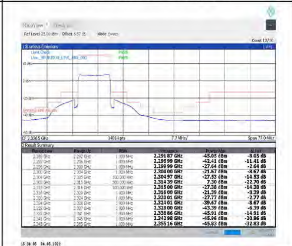
1-N30--15-10-L-6-CP-QPSK-Outer_Full-52@0-Ant1-PASS-see graph
