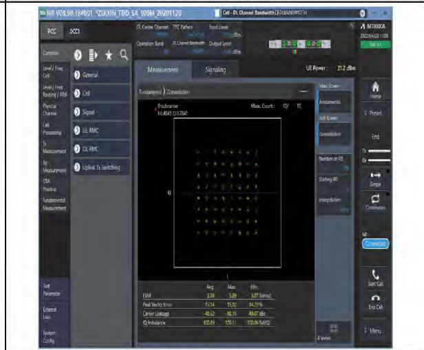
1-N38--30-40-M-8-CP-64QAM-Outer_Full-106@0- Ant1-see graph-PASS
