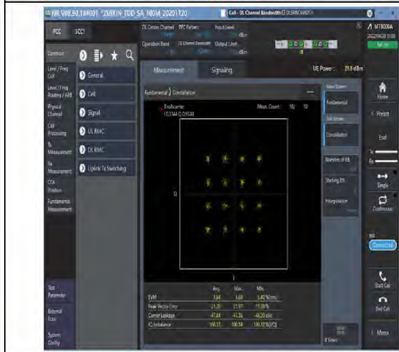
1-N38--30-40-M-7-CP-16QAM-Outer_Full-106@0- Ant1-see graph-PASS
