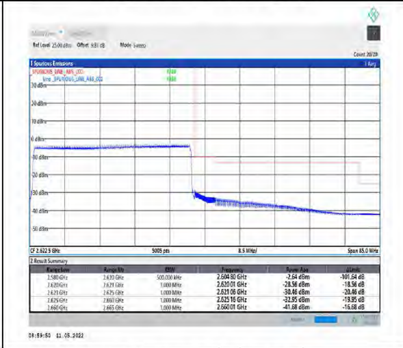
1-N38-PC2-30-40-H-6-CP-QPSK-Outer_Full-106@0-Ant1-PASS-see graph
