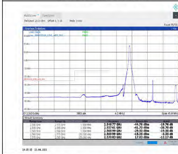
1-N38--30-15-L-4-CP-QPSK-Edge_1RB_Left-1@0-Ant1-PASS-see graph
