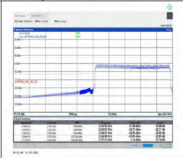
1-N38-PC2-30-30-L-6-CP-QPSK-Outer_Full-78@0-Ant1-PASS-see graph
