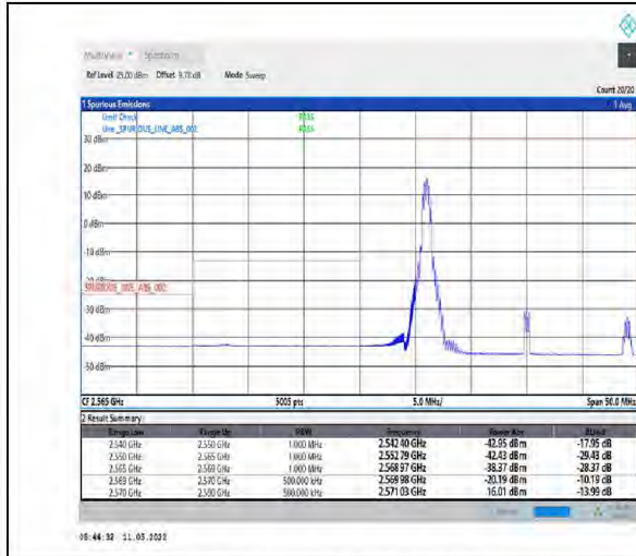
1-N38-PC2-30-20-L-4-CP-QPSK-Edge_1RB_Left-1@0-Ant1-PASS-see graph
