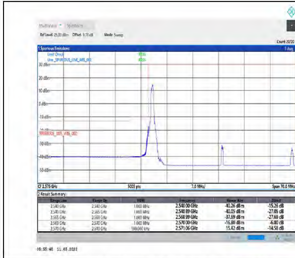
1-N38-PC2-30-40-L-4-CP-QPSK-Edge_1RB_Left-1@0-Ant1-PASS-see graph
