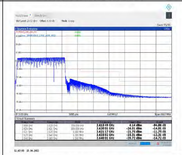
1-N38--30-20-H-6-CP-QPSK-Outer_Full-51@0-Ant1-PASS-see graph
