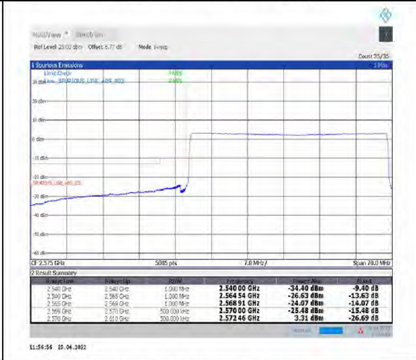
1-N38--30-40-L-6-CP-QPSK-Outer_Full-106@0-Ant1-PASS-see graph
