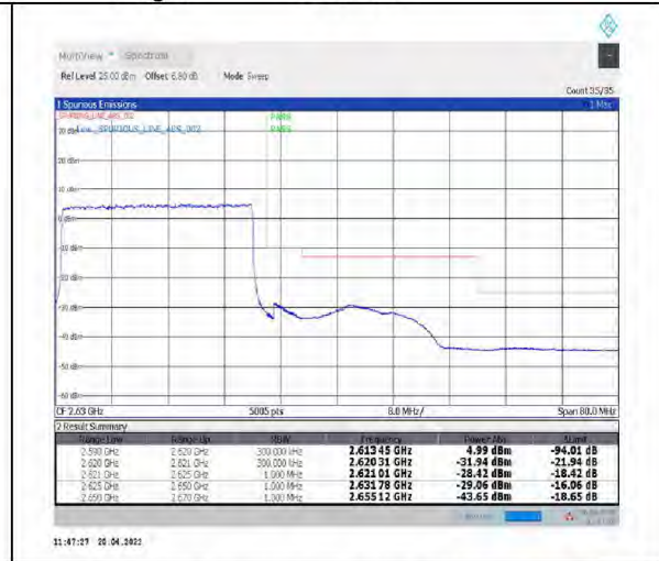
1-N38--30-30-H-3-DFT-PI2BPSK-Outer_Full-75@0-Ant1-PASS-see graph
