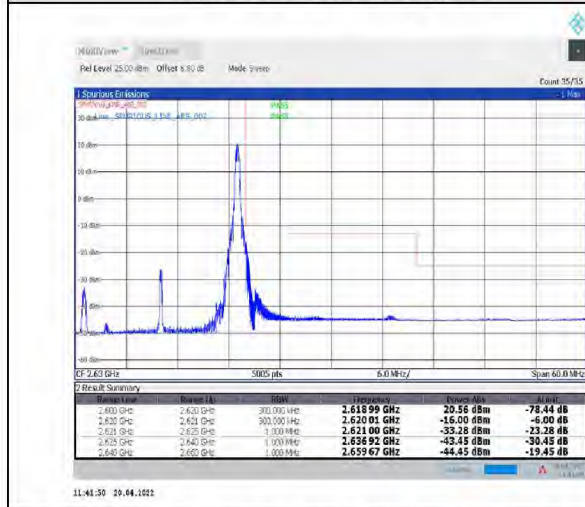
1-N38--30-20-H-5-CP-QPSK-Edge_1RB_Right-1@50-Ant1-PASS-see graph
