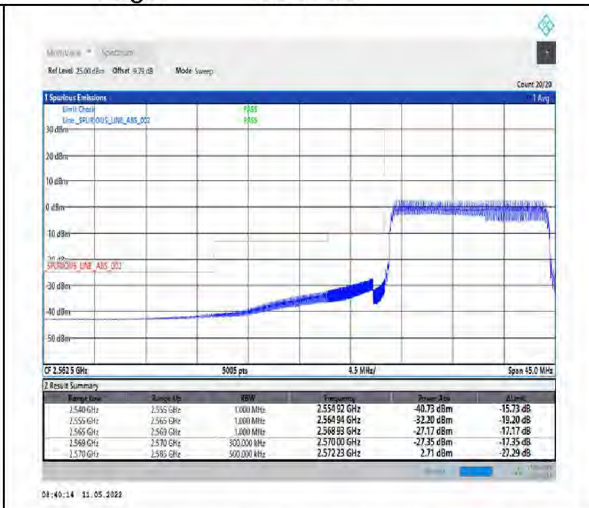
1-N38-PC2-30-15-L-6-CP-QPSK-Outer_Full-38@0-Ant1-PASS-see graph
