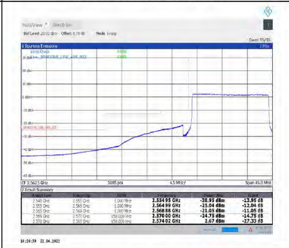
1-N38--30-15-L-6-CP-QPSK-Outer_Full-38@0-Ant1-PASS-see graph
