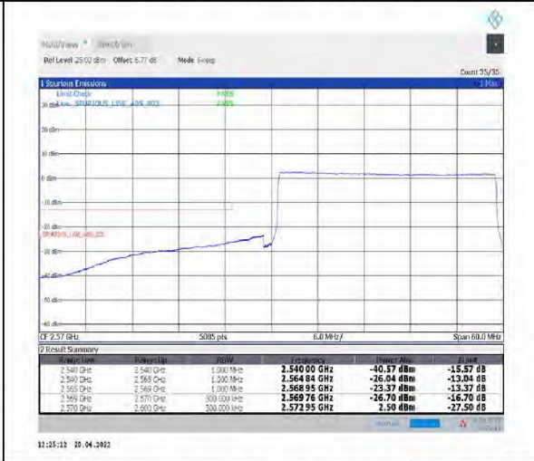
1-N38--30-30-L-6-CP-QPSK-Outer_Full-78@0-Ant1-PASS-see graph
