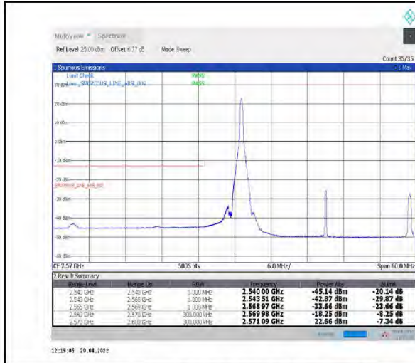
1-N38--30-30-L-1-DFT-PI2BPSK-Edge_1RB_Left-1@0-Ant1-PASS-see graph
