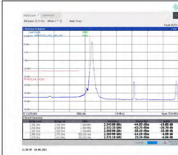
1-N38--30-40-L-1-DFT-PI2BPSK-Edge_1RB_Left-1@0-Ant1-PASS-see graph
