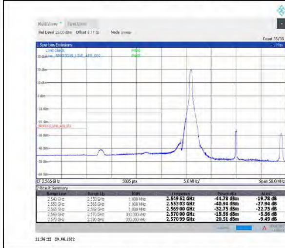
1-N38--30-20-L-4-CP-QPSK-Edge_1RB_Left-1@0-Ant1-PASS-see graph
