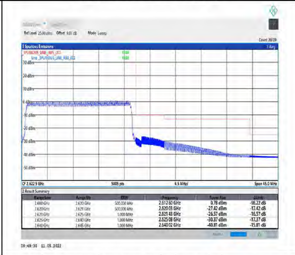
1-N38-PC2-30-20-H-6-CP-QPSK-Outer_Full-51@0-Ant1-PASS-see graph
