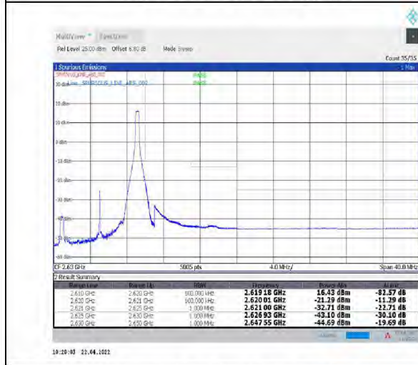
1-N38--30-10-H-5-CP-QPSK-Edge_1RB_Right-1@23-Ant1-PASS-see graph
