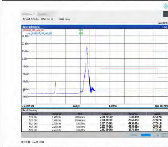
1-N38-PC2-30-30-H-5-CP-QPSK-Edge_1RB_Right-1@77-Ant1-PASS-see graph
