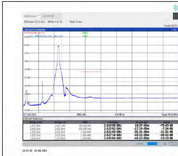
1-N38--30-10-H-2-DFT-PI2BPSK-Edge_1RB_Right-1@23-Ant1-PASS-see graph
