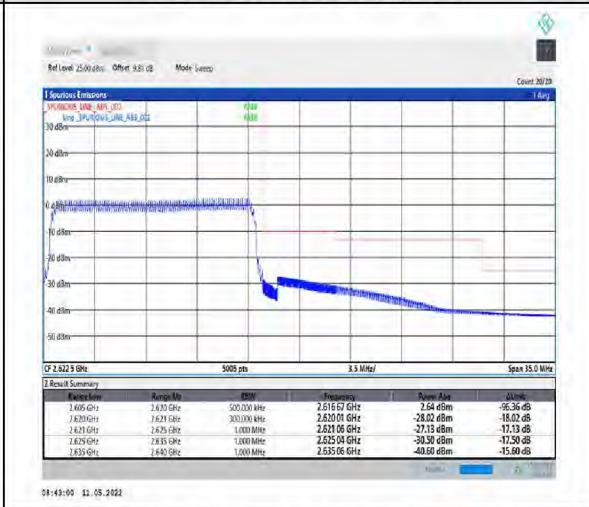
1-N38-PC2-30-15-H-6-CP-QPSK-Outer_Full-38@0-Ant1-PASS-see graph
