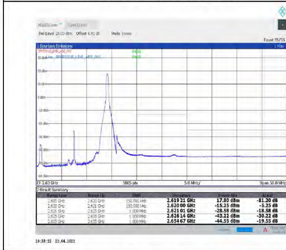
1-N38--30-15-H-5-CP-QPSK-Edge_1RB_Right-1@37-Ant1-PASS-see graph
