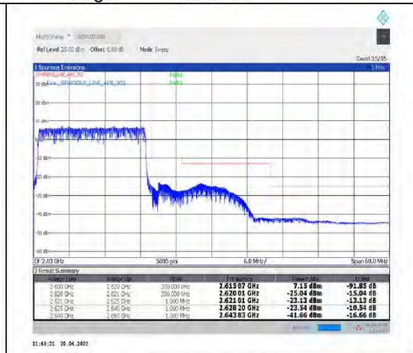
1-N38--30-20-H-3-DFT-PI2BPSK-Outer_Full-50@0-Ant1-PASS-see graph
