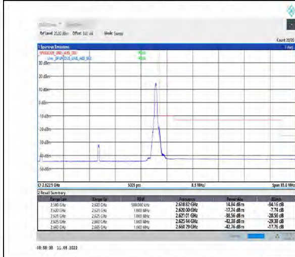
1-N38-PC2-30-40-H-5-CP-QPSK-Edge_1RB_Right-1@105-Ant1-PASS-see graph
