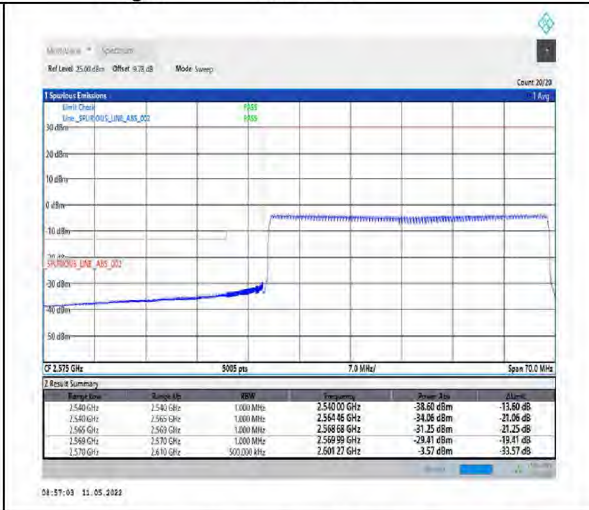
1-N38-PC2-30-40-L-6-CP-QPSK-Outer_Full-106@0-Ant1-PASS-see graph
