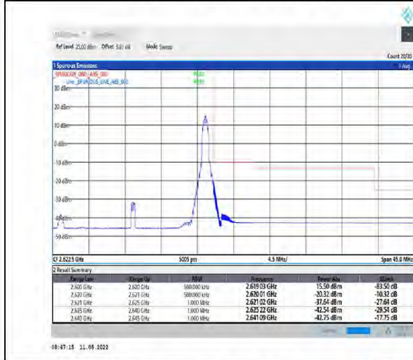
1-N38-PC2-30-20-H-5-CP-QPSK-Edge_1RB_Right-1@50-Ant1-PASS-see graph
