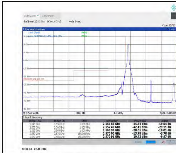
1-N38--30-15-L-1-DFT-PI2BPSK-Edge_1RB_Left-1@0-Ant1-PASS-see graph
