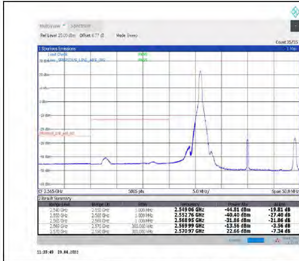
1-N38--30-20-L-1-DFT-PI2BPSK-Edge_1RB_Left-1@0-Ant1-PASS-see graph
