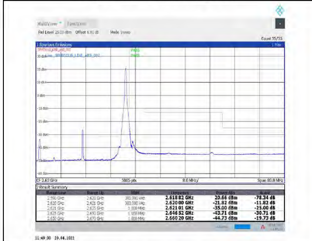
1-N38--30-30-H-5-CP-QPSK-Edge_1RB_Right-1@77-Ant1-PASS-see graph
