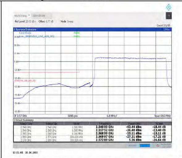
1-N38--30-30-L-3-DFT-PI2BPSK-Outer_Full-75@0-Ant1-PASS-see graph
