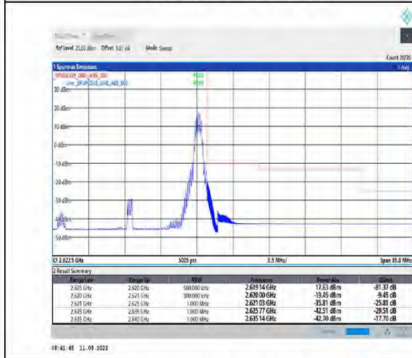
1-N38-PC2-30-15-H-5-CP-QPSK-Edge_1RB_Right-1@37-Ant1-PASS-see graph
