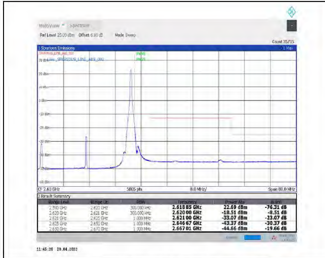
1-N38--30-30-H-2-DFT-PI2BPSK-Edge_1RB_Right-1@77-Ant1-PASS-see graph
