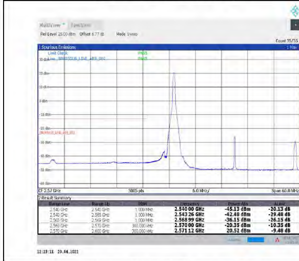
1-N38--30-30-L-4-CP-QPSK-Edge_1RB_Left-1@0-Ant1-PASS-see graph
