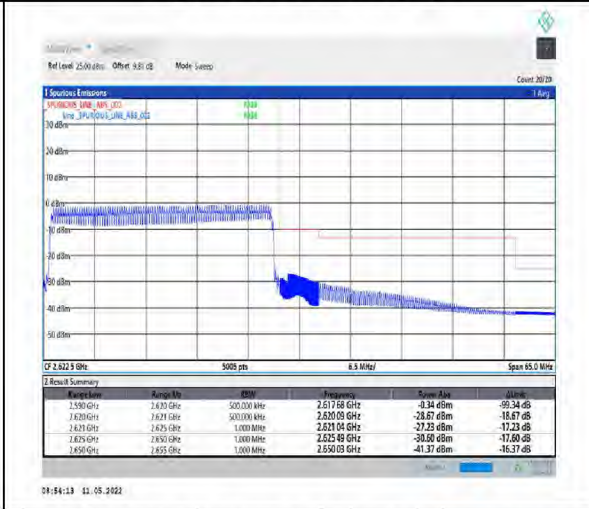
1-N38-PC2-30-30-H-6-CP-QPSK-Outer_Full-78@0-Ant1-PASS-see graph
