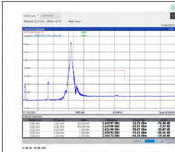
1-N38--30-20-H-2-DFT-PI2BPSK-Edge_1RB_Right-1@50-Ant1-PASS-see graph
