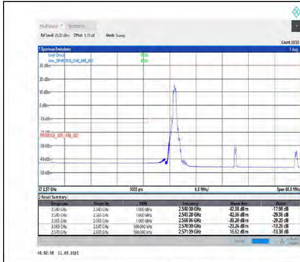
1-N38-PC2-30-30-L-4-CP-QPSK-Edge_1RB_Left-1@0-Ant1-PASS-see graph
