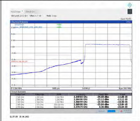
1-N38--30-20-L-6-CP-QPSK-Outer_Full-51@0-Ant1-PASS-see graph
