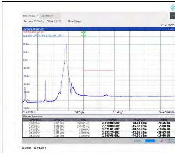
1-N38--30-15-H-2-DFT-PI2BPSK-Edge_1RB_Right-1@37-Ant1-PASS-see graph
