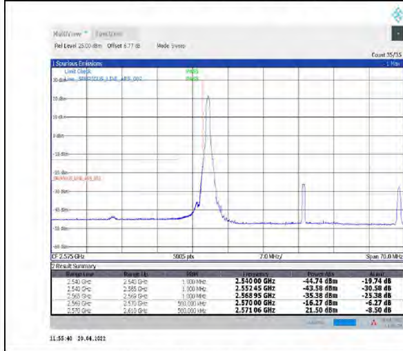
1-N38--30-40-L-4-CP-QPSK-Edge_1RB_Left-1@0-Ant1-PASS-see graph
