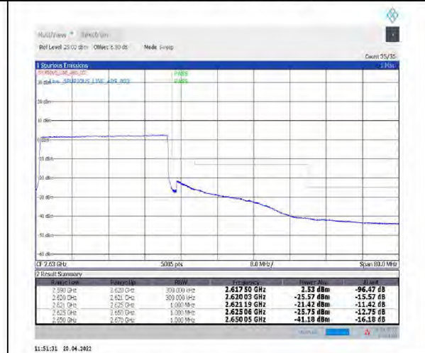
1-N38--30-30-H-6-CP-QPSK-Outer_Full-78@0-Ant1-PASS-see graph
