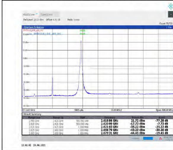
1-N38--30-40-H-5-CP-QPSK-Edge_1RB_Right-1@105-Ant1-PASS-see graph
