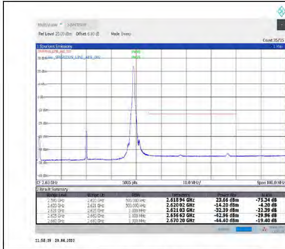
1-N38--30-40-H-2-DFT-PI2BPSK-Edge_1RB_Right-1@105-Ant1-PASS-see graph
