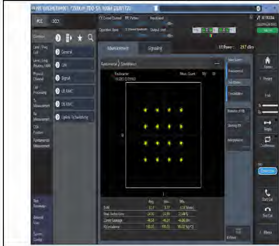
1-N41--30-100-M-7-CP-16QAM-Outer_Full-273@0-Ant1-see graph-PASS
