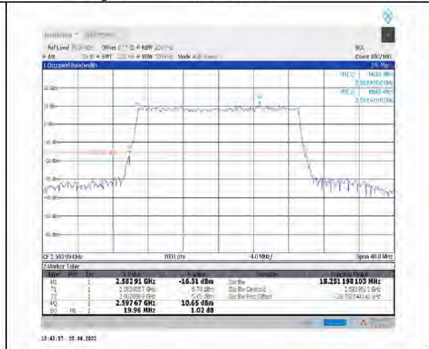
1-N41--30-20-M-9-CP-256QAM-Outer_Full-51@0-Ant1-18.251-19.960-<20-PASS
