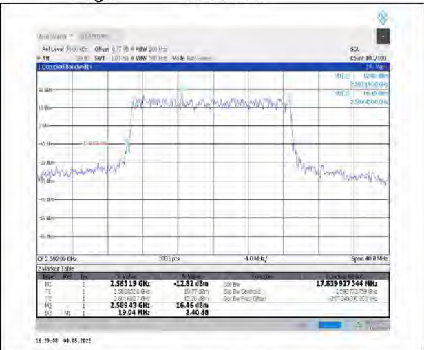
1-N41--30-20-M-1-DFT-QPSK-Outer_Full-50@0-Ant1-17.84-19.040-<20-PASS
