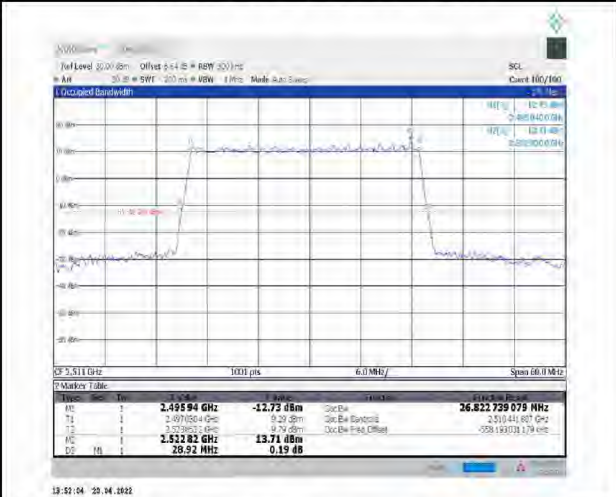
1-N41--30-30-L-5-DFT-256QAM-Outer_Full-75@0-Ant1-26.823-28.920-<30-PASS
