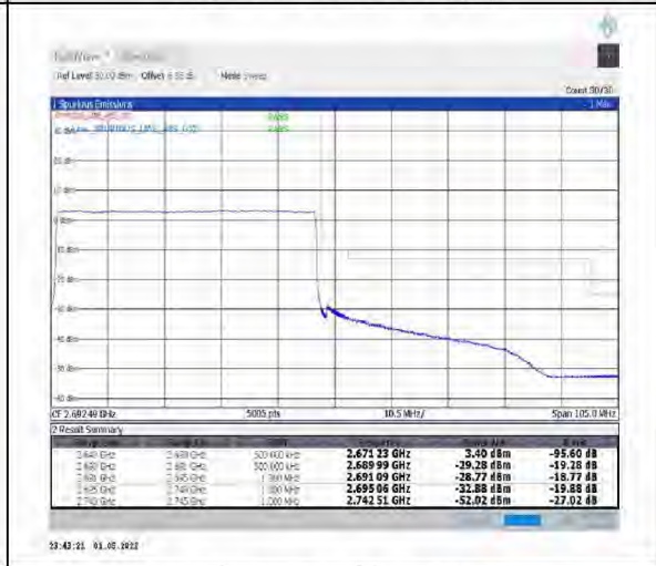
1-N41-PC2-30-50-H-6-CP-QPSK-Outer_Full-133@0-Ant2-PASS-see graph
