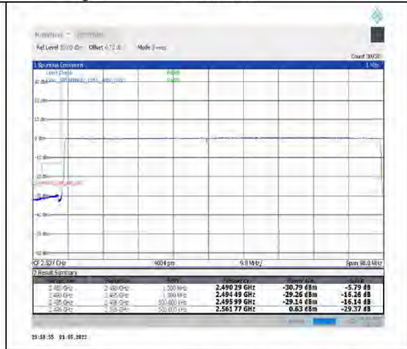
1-N41-PC2-30-90-L-6-CP-QPSK-Outer_Full-245@0-Ant2-PASS-see graph
