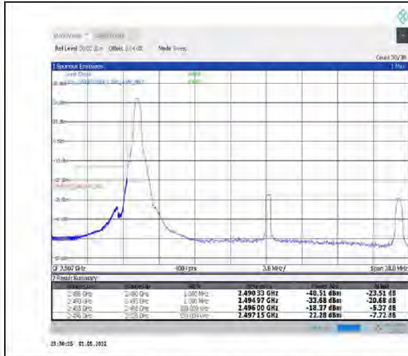
1-N41-PC2-30-30-L-4-CP-QPSK-Edge_1RB_Left-1@0-Ant2-PASS-see graph
