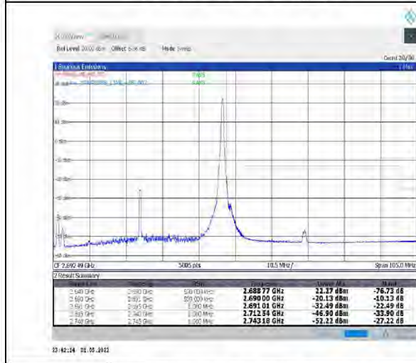
1-N41-PC2-30-50-H-5-CP-QPSK-Edge_1RB_Right-1@132-Ant2-PASS-see graph
