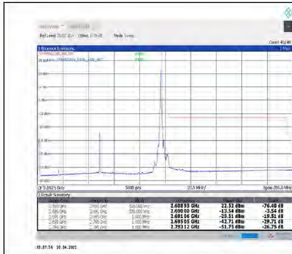
1-N41--30-100-H-2-DFT-PI2BPSK-Edge_1RB_Right-1@272-Ant1-PASS-see graph
