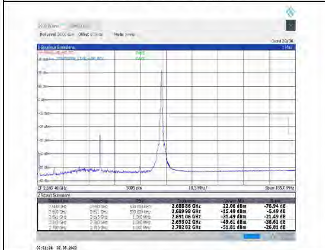
1-N41-PC2-30-90-H-5-CP-QPSK-Edge_1RB_Right-1@244-Ant2-PASS-see graph
