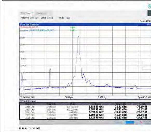
1-N41--30-30-H-5-CP-QPSK-Edge_1RB_Right-1@77-Ant1-PASS-see graph
