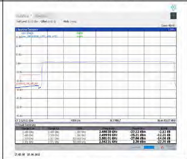
1-N41--30-70-L-6-CP-QPSK-Outer_Full-189@0-Ant1-PASS-see graph
