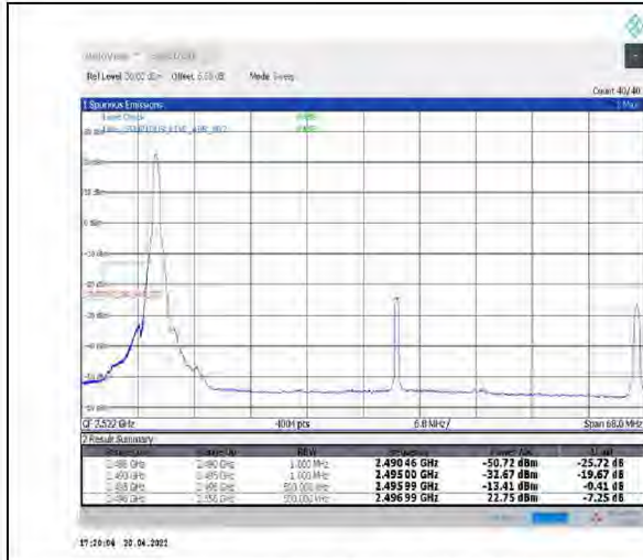
1-N41--30-60-L-1-DFT-PI2BPSK-Edge_1RB_Left-1@0-Ant1-PASS-see graph
