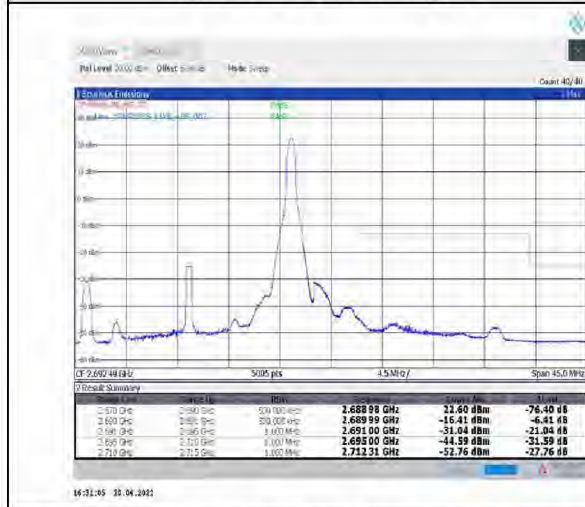
1-N41--30-20-H-5-CP-QPSK-Edge_1RB_Right-1@50-Ant1-PASS-see graph
