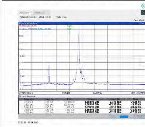
1-N41--30-60-H-5-CP-QPSK-Edge_1RB_Right-1@161-Ant1-PASS-see graph
