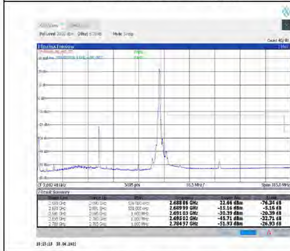
1-N41--30-90-H-5-CP-QPSK-Edge_1RB_Right-1@244-Ant1-PASS-see graph
