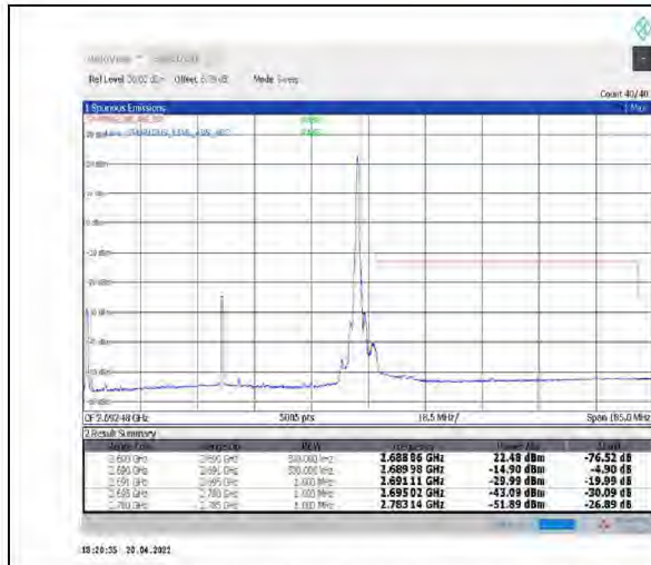
1-N41--30-90-H-2-DFT-PI2BPSK-Edge_1RB_Right-1@244-Ant1-PASS-see graph
