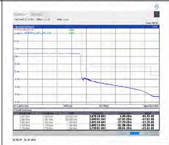
1-N41-PC2-30-40-H-6-CP-QPSK-Outer_Full-106@0-Ant2-PASS-see graph
