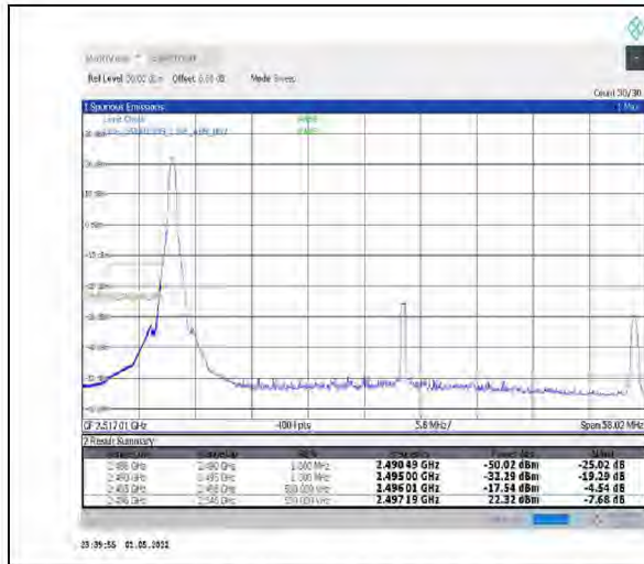
1-N41-PC2-30-50-L-4-CP-QPSK-Edge_1RB_Left-1@0-Ant2-PASS-see graph
