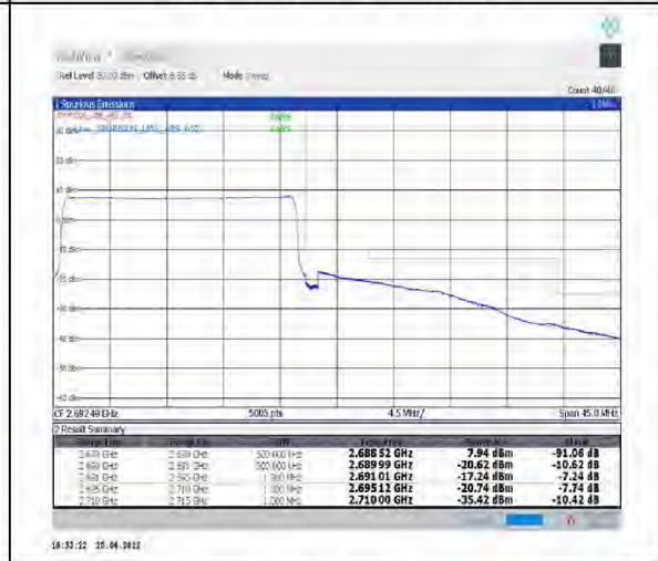
1-N41--30-20-H-6-CP-QPSK-Outer_Full-51@0-Ant1-PASS-see graph
