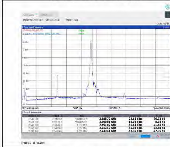
1-N41--30-50-H-5-CP-QPSK-Edge_1RB_Right-1@132-Ant1-PASS-see graph
