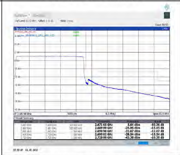
1-N41-PC2-30-30-H-6-CP-QPSK-Outer_Full-78@0-Ant2-PASS-see graph
