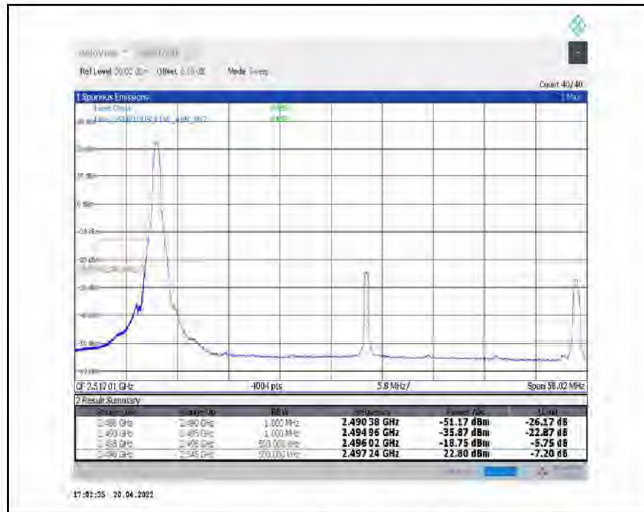
1-N41--30-50-L-1-DFT-PI2BPSK-Edge_1RB_Left-1@0-Ant1-PASS-see graph
