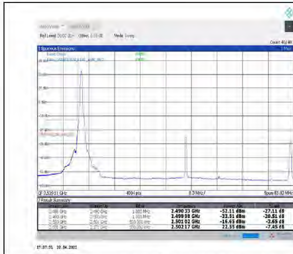
1-N41--30-70-L-1-DFT-PI2BPSK-Edge_1RB_Left-1@0-Ant1-PASS-see graph
