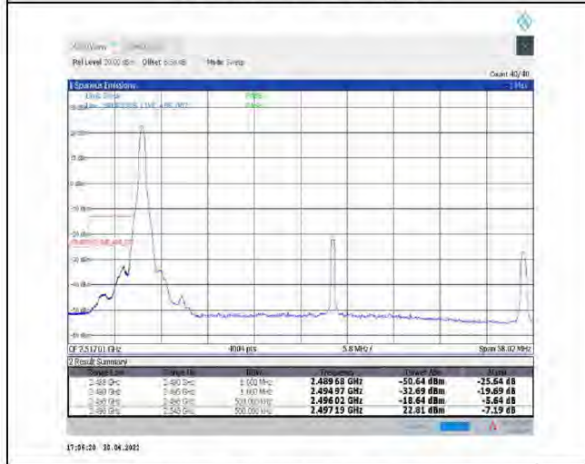
1-N41--30-50-L-4-CP-QPSK-Edge_1RB_Left-1@0-Ant1-PASS-see graph
