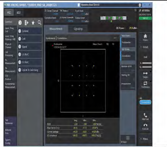
1-N66-PC3-15-40-M-3-DFT-16QAM-Outer_Full_216@0-Ant1-see graph-PASS
