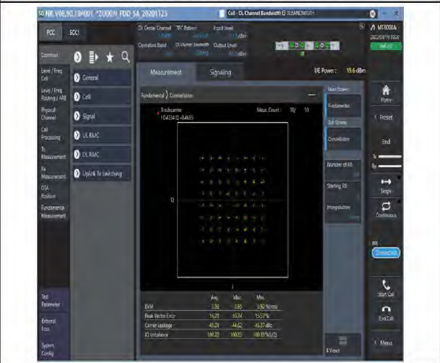
1-N66-PC3-15-20-M-8-CP-64QAM-Outer_Full-106@0-Ant1-see graph-PASS
