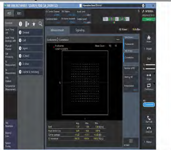
1-N66-PC3-15-40-M-5-DFT-256QAM-Outer_Full-216@0-Ant1-see graph-PASS
