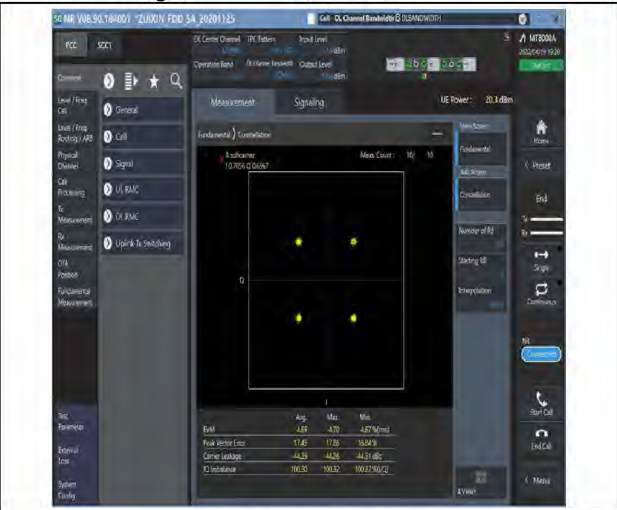
1-N66-PC3-15-20-M-6-CP-QPSK-Outer_Full-106@0-Ant1-see graph-PASS
