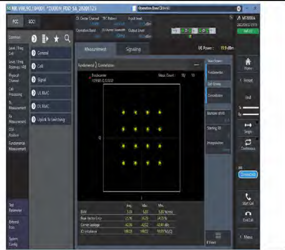
1-N66-PC3-15-40-M-7-CP-16QAM-Outer_Full-216@0-Ant1-see graph-PASS
