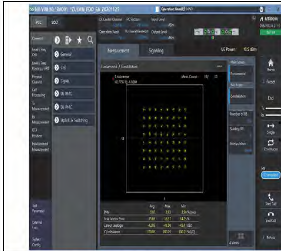
1-N66-PC3-15-40-M-8-CP-64QAM-Outer_Full-216@0-Ant1-see graph-PASS
