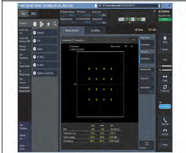
1-N66-PC3-15-20-M-7-CP-16QAM-Outer_Full-106@0-Ant1-see graph-PASS
