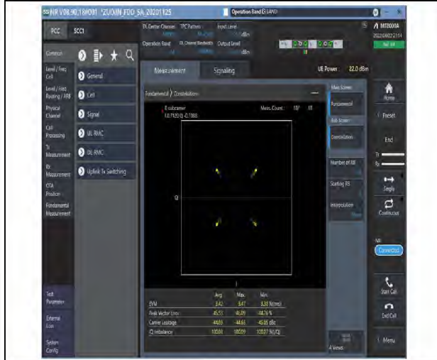
1-N66-PC3-15-40-M-2-DFT-QPSK-Outer_Full_216@0-Ant1-see graph-PASS
