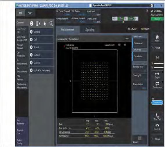
1-N66-PC3-15-40-M-9-CP-256QAM-Outer_Full-216@0-Ant1-see graph-PASS
