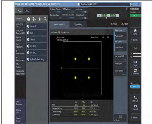
1-N66-PC3-15-40-M-6-CP-QPSK-Outer_Full-216@0-Ant1-see graph-PASS
