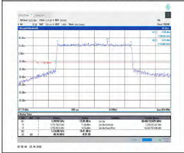
1-N66-PC3-15-40-L-4-DFT-64QAM-Outer_Full-216@0-Ant1-38.467-40.160-≤40-PASS
