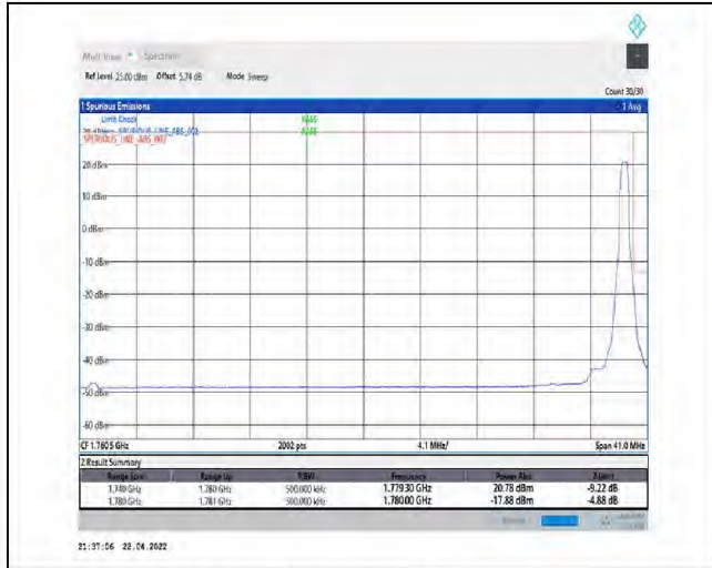
1-N66-PC3-15-40-H-2-DFT-PI2BPSK-Edge_1RB_Right-1@215-Ant1-seegraph-PASS-see graph
