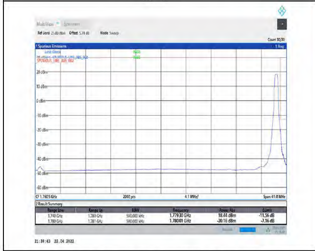
1-N66-PC3-15-40-H-5-CP-QPSK-Edge_1RB_Right-1@215-Ant1-seegraph-PASS-see graph
