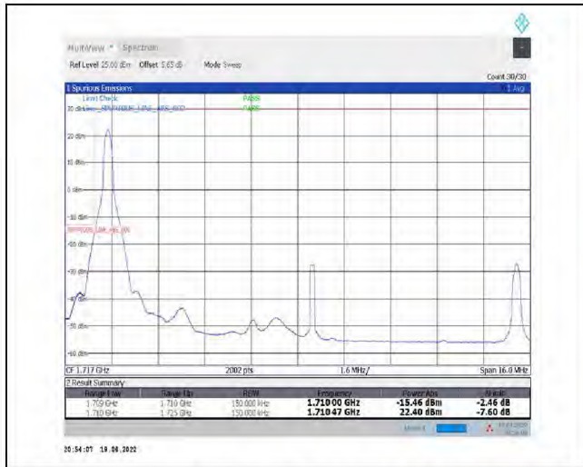
1-N66-PC3-15-15-L-1-DFT-PI2BPSK-Edge_1RB_Left-1@0-Ant1-seegraph-PASS-see graph
