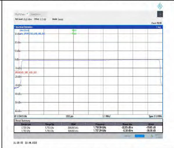
1-N66-PC3-15-30-L-6-CP-QPSK-Outer_Full-160@0-Ant1-seegraph-PASS-see graph
