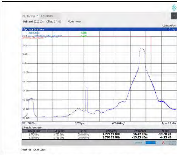
1-N66-PC3-15-5-H-2-DFT-PI2BPSK-Edge_1RB_Right-1@24-Ant1-seegraph-PASS-see graph
