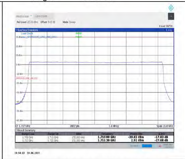
1-N66-PC3-15-15-L-3-DFT-PI2BPSK-Outer_Full-75@0-Ant1-seegraph-PASS-see graph
