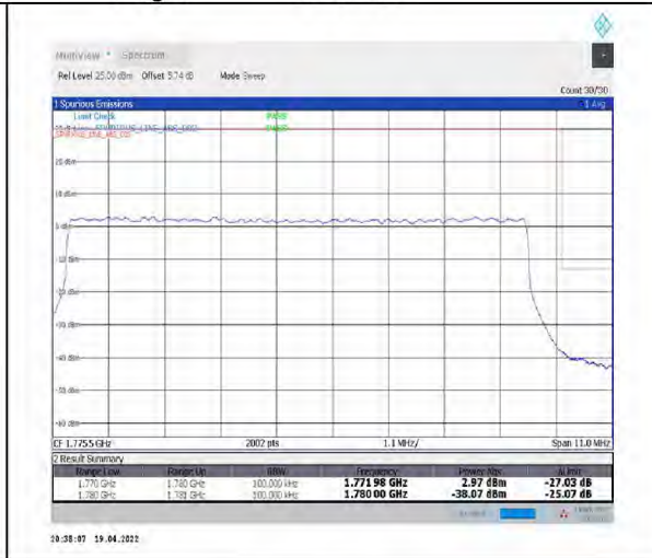
1-N66-PC3-15-10-H-3-DFT-PI2BPSK-Outer_Full-50@0-Ant1-seegraph-PASS-see graph
