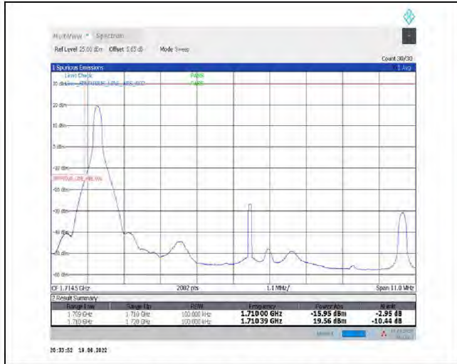
1-N66-PC3-15-10-L-1-DFT-PI2BPSK-Edge_1RB_Left-1@0-Ant1-seegraph-PASS-see graph
