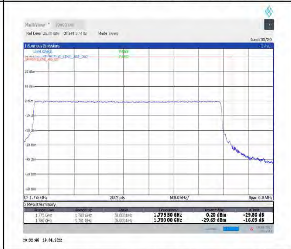
1-N66-PC3-15-5-H-6-CP-QPSK-Outer_Full-25@0-Ant1-seegraph-PASS-see graph
