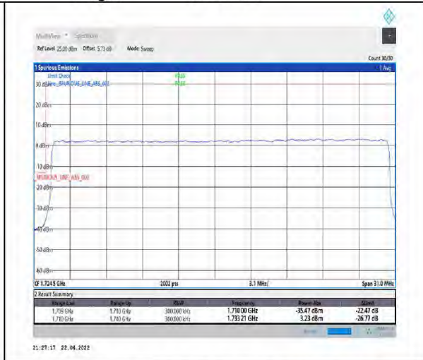
1-N66-PC3-15-30-L-3-DFT-PI2BPSK-Outer_Full-160@0-Ant1-seegraph-PASS-see graph
