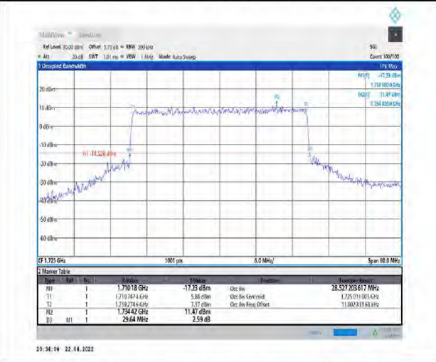
1-N66-PC3-15-30-L-8-CP-64QAM-Outer_Full-160@0-Ant1-28.527-29.640-≤30-PASS
