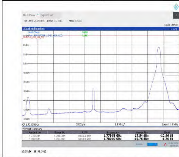
1-N66-PC3-15-10-H-5-CP-QPSK-Edge_1RB_Right-1@51-Ant1-seegraph-PASS-see graph
