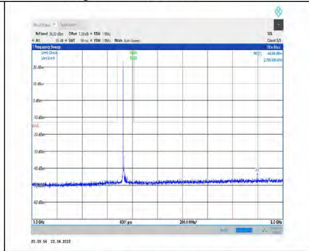
1-N66-PC3-15-40-M-1-DFT-PI2BPSK- Inner_1RB_Left-1@1-1000-3000-Ant1--44.44--13-PASS
