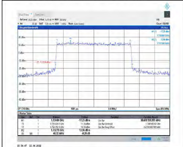
1-N66-PC3-15-40-M-3-DFT-16QAM-Outer_Full-216@0-Ant1-38.619-40.320-≤40-PASS
