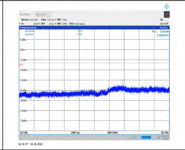
1-N66-PC3-15-40-M-1-DFT-PI2BPSK- Inner_1RB_Left-1@1-12000-20000-Ant1--33.38--13-PASS
