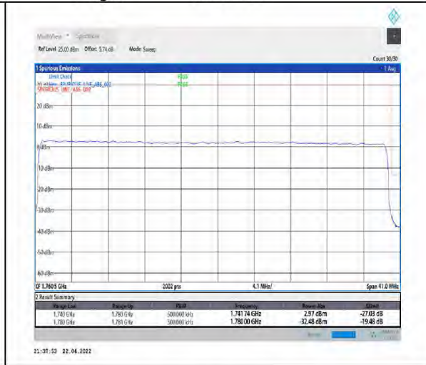
1-N66-PC3-15-40-H-3-DFT-PI2BPSK-Outer_Full-216@0-Ant1-seegraph-PASS-see graph
