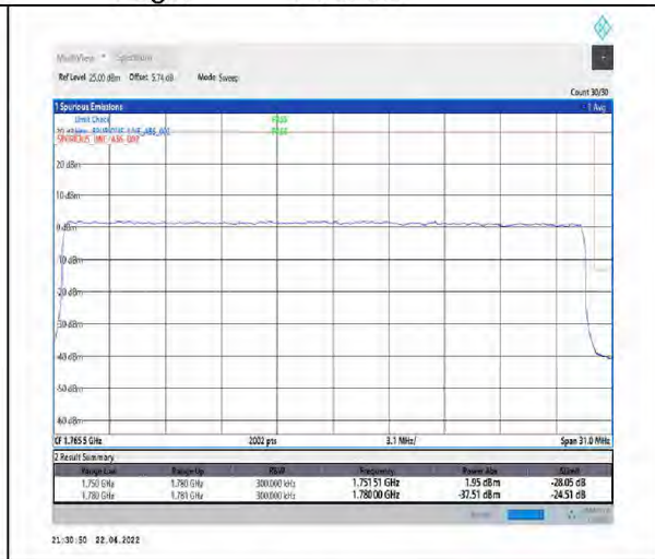
1-N66-PC3-15-30-H-3-DFT-PI2BPSK-Outer_Full-160@0-Ant1-seegraph-PASS-see graph
