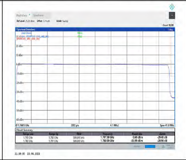
1-N66-PC3-15-40-H-6-CP-QPSK-Outer_Full-216@0-Ant1-seegraph-PASS-see graph
