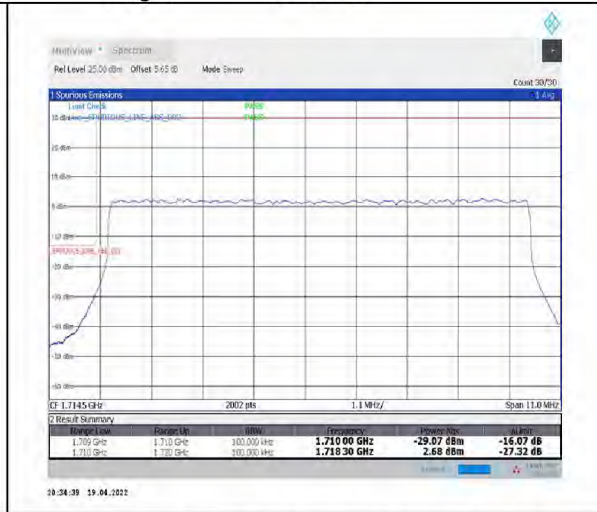
1-N66-PC3-15-10-L-3-DFT-PI2BPSK-Outer_Full-50@0-Ant1-seegraph-PASS-see graph
