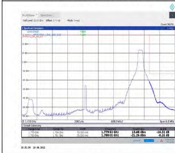
1-N66-PC3-15-5-H-5-CP-QPSK-Edge_1RB_Right-1@24-Ant1-seegraph-PASS-see graph
