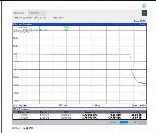
1-N66-PC3-15-10-H-6-CP-QPSK-Outer_Full-52@0-Ant1-seegraph-PASS-see graph
