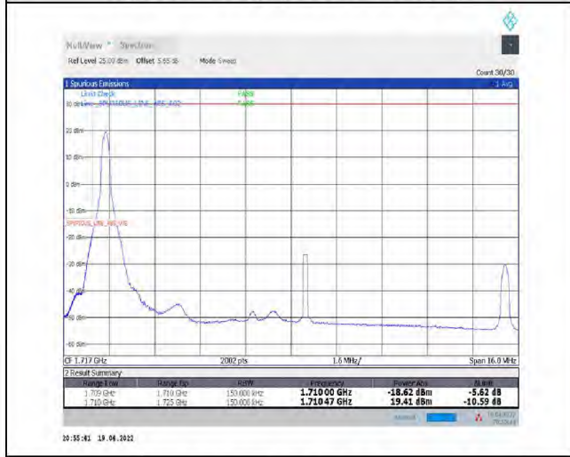
1-N66-PC3-15-15-L-4-CP-QPSK-Edge_1RB_Left-1@0-Ant1-seegraph-PASS-see graph
