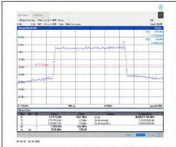
1-N66-PC3-15-30-L-9-CP-256QAM-Outer_Full-160@0-Ant1-28.538-29.760-≤30-PASS
