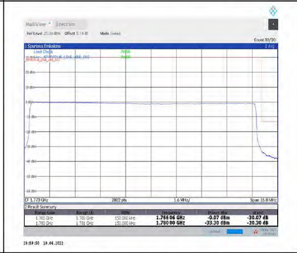
1-N66-PC3-15-15-H-6-CP-QPSK-Outer_Full-79@0-Ant1-seegraph-PASS-see graph
