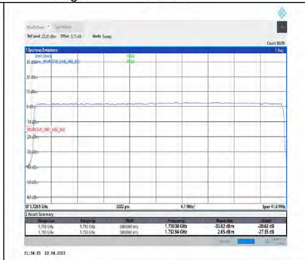
1-N66-PC3-15-40-L-3-DFT-PI2BPSK-Outer_Full-216@0-Ant1-seegraph-PASS-see graph
