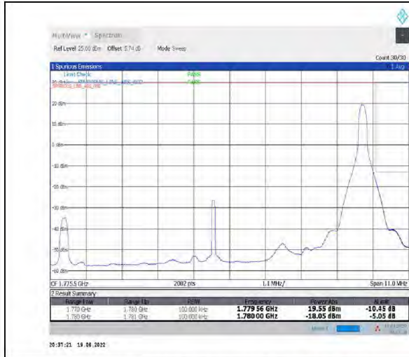
1-N66-PC3-15-10-H-2-DFT-PI2BPSK-Edge_1RB_Right-1@51-Ant1-seegraph-PASS-see graph
