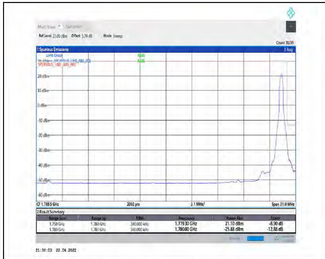
1-N66-PC3-15-30-H-2-DFT-PI2BPSK-Edge_1RB_Right-1@159-Ant1-seegraph-PASS-see graph
