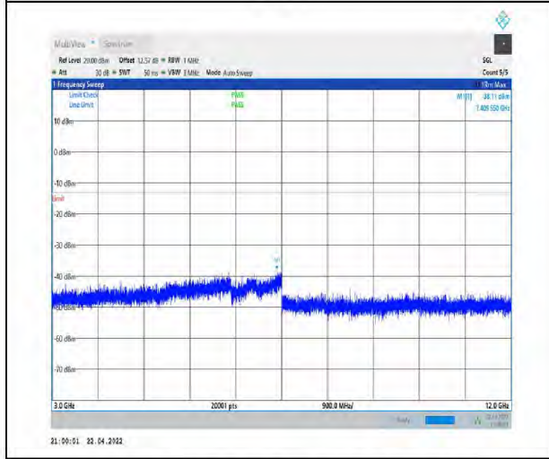
1-N66-PC3-15-40-M-1-DFT-PI2BPSK- Inner_1RB_Left-1@1-3000-12000-Ant1--38.11--13-PASS
