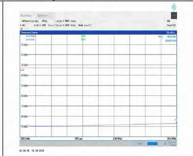
1-N66-PC3-15-40-H-1-DFT-PI2BPSK- Inner_1RB_Left-1@1-0.15-30-Ant1--86.92--33-PASS
