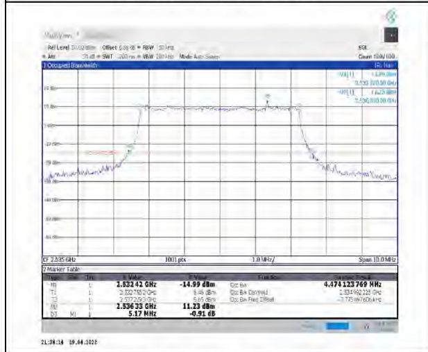
1-N7--15-5-M-6-CP-QPSK-Outer_Full-25@0-Ant1-4,474-5.170-<math>\leq</math>5-PASS
