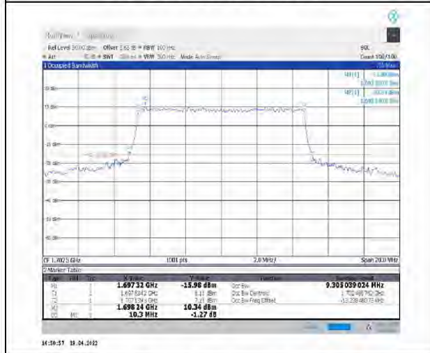
1-N70--15-10-M-7-CP-16QAM-Outer_Full-52@0-Ant1-9.305-10.300-<=10-PASS
