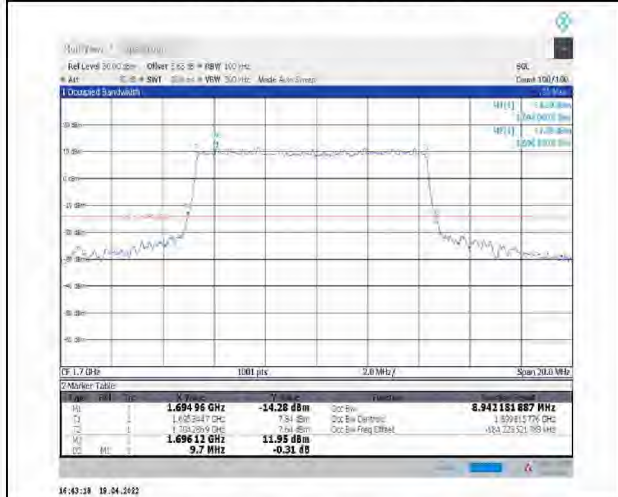
1-N70--15-10-L-4-DFT-64QAM-Outer_Full-50@0-Ant1-8.942-9.700-<math>\leq 10</math>-PASS
