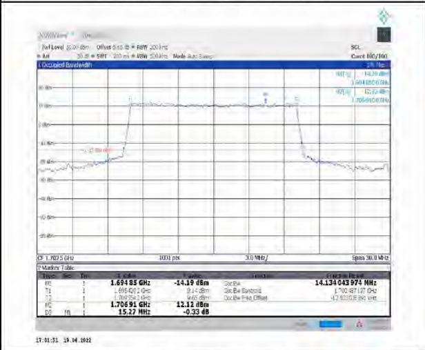
1-N70--15-15-L-6-CP-QPSK-Outer_Full-79@0-Ant1-14.134-15.270-≤15-PASS
