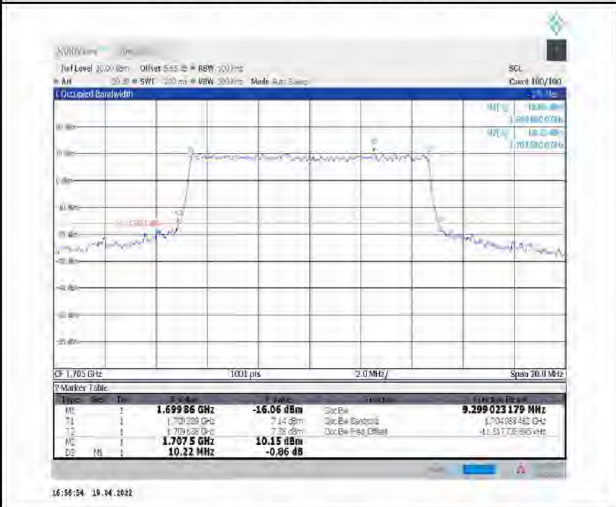
1-N70--15-10-H-7-CP-16QAM-Outer_Full-52@0-Ant1-9.299-10.220-<=10-PASS
