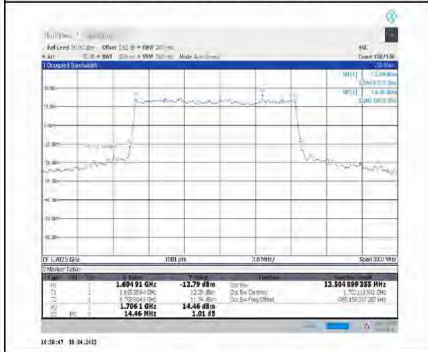
1-N70--15-15-L-1-DFT-QPSK-Outer_Full-75@0- Ant1-13.505-14.460-≤15-PASS
