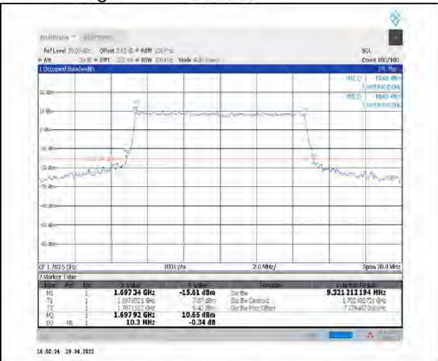
1-N70--15-10-M-6-CP-QPSK-Outer_Full-52@0-Ant1-9.321-10.300-<=10-PASS
