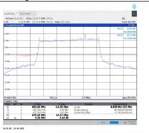
1-N71--15-10-L-3-DFT-16QAM-Outer_Full-50@0-Ant1-8.94-9.580-≤10-PASS
