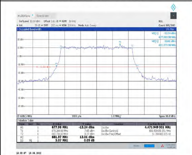
1-N71--15-5-M-3-DFT-16QAM-Outer_Full-25@0- Ant1-4.472-5.070-<math>\leq 5</math>-PASS
