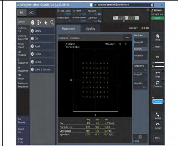
1-N71--15-20-M-8-CP-64QAM-Outer_Full-106@0- Ant1-see graph-PASS
