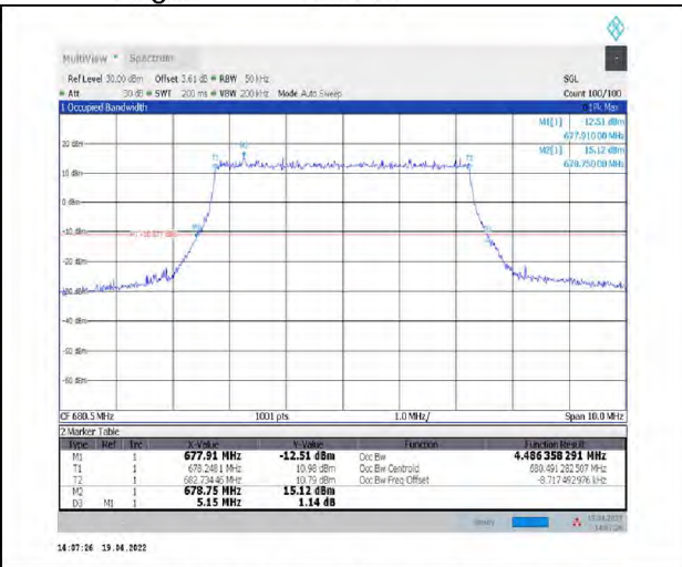
1-N71--15-5-M-1-DFT-QPSK-Outer_Full-25@0- Ant1-4.486-5.150-<math>\leq 5</math>-PASS
