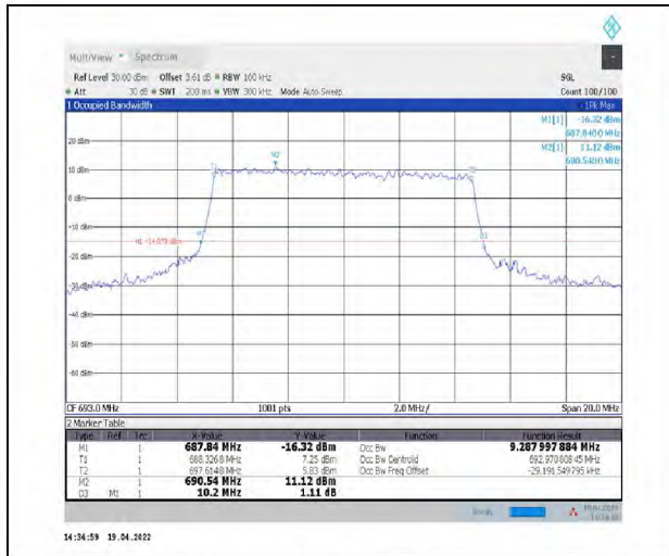
1-N71--15-10-H-8-CP-64QAM-Outer_Full-52@0- Ant1-9.288-10.200-<=10-PASS
