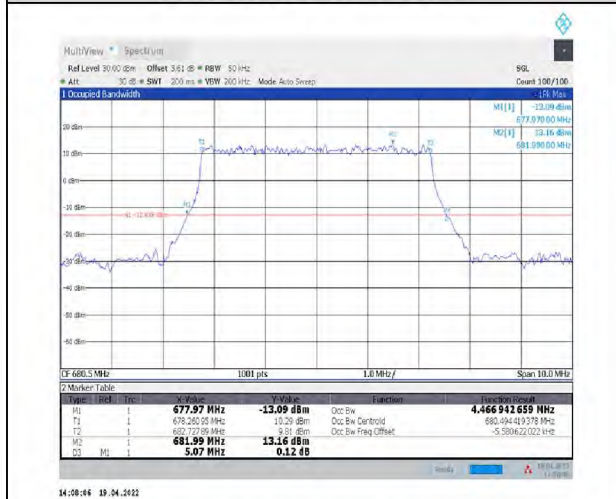
1-N71--15-5-M-2-DFT-PI2BPSK-Outer_Full-25@0- Ant1-4.467-5.070-<math>\leq 5</math>-PASS
