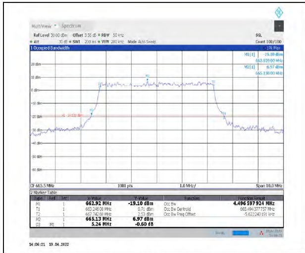
1-N71--15-5-L-9-CP-256QAM-Outer_Full-25@0- Ant1-4.497-5.240-<math>\leq 5</math>-PASS
