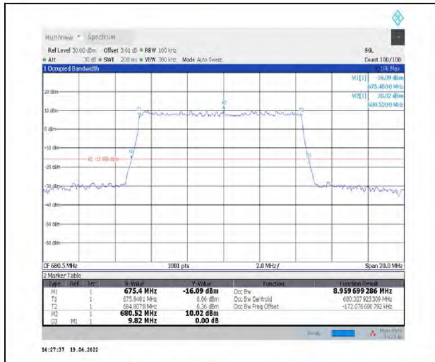
1-N71--15-10-M-5-DFT-256QAM-Outer_Full-50@0-Ant1-8.96-9.820-<=10-PASS
