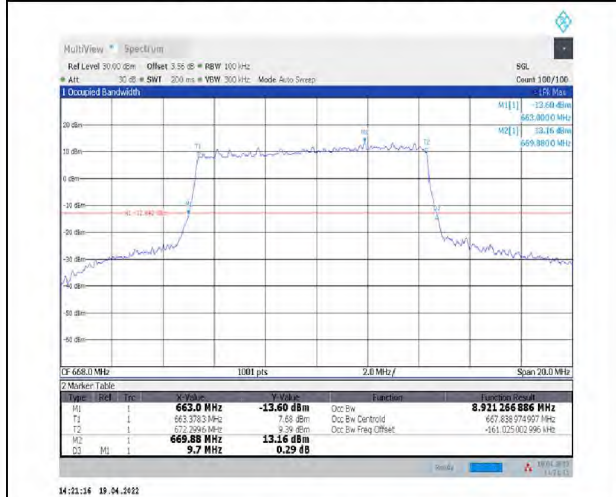
1-N71--15-10-L-4-DFT-64QAM-Outer_Full-50@0-Ant1-8.921-9.700-≤10-PASS
