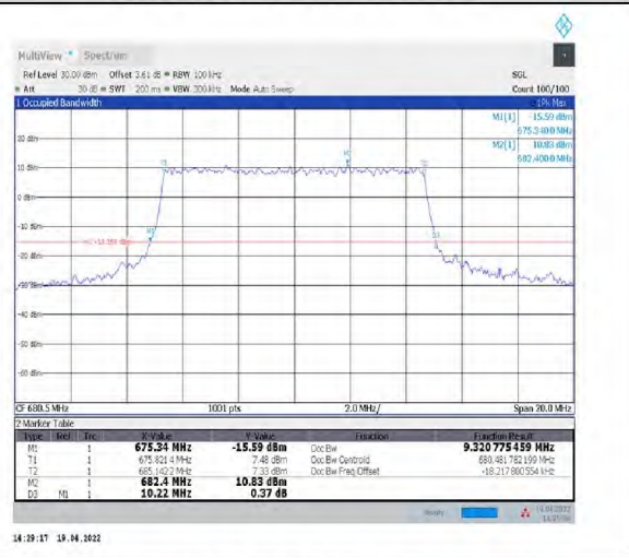
1-N71--15-10-M-8-CP-64QAM-Outer_Full-52@0-Ant1-9.321-10.220-<=10-PASS
