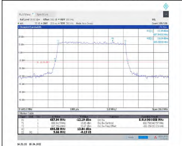
1-N71--15-10-H-2-DFT-PI2BPSK-Outer_Full-50@0-Ant1-8.915-9.660-≤10-PASS
