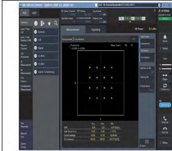
1-N71--15-20-M-7-CP-16QAM-Outer_Full-106@0- Ant1-see graph-PASS
