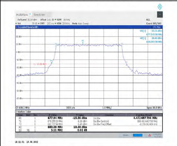
1-N71--15-5-M-7-CP-16QAM-Outer_Full-25@0-Ant1-4.473-5.110-<math>\leq 5</math>-PASS
