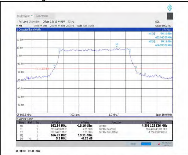
1-N71--15-5-L-6-CP-QPSK-Outer_Full-25@0-Ant1-4.501-5.200-<math>\leq</math>5-PASS
