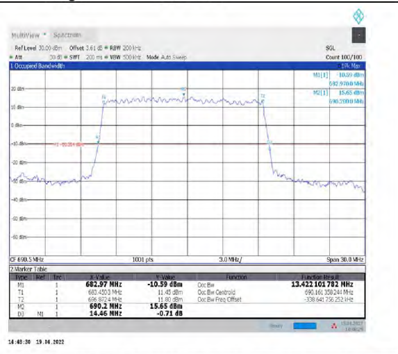
1-N71--15-15-H-2-DFT-PI2BPSK-Outer_Full-75@0- Ant1-13.422-14.460-<=15-PASS
