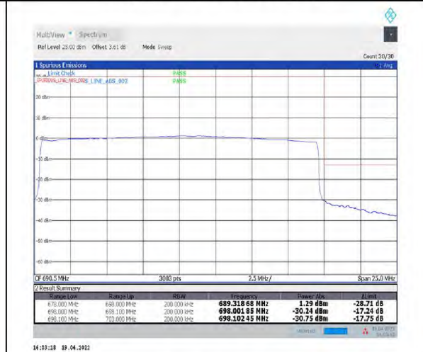
1-N71--15-20-H-6-CP-QPSK-Outer_Full-106@0-Ant1-PASS-see graph
