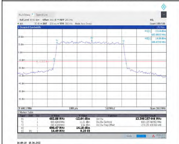
1-N71--15-15-H-3-DFT-16QAM-Outer_Full-75@0- Ant1-13.398-14.490-<=15-PASS
