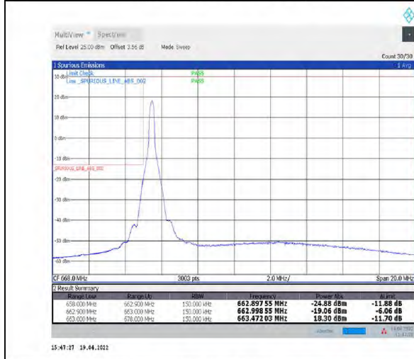
1-N71--15-15-L-4-CP-QPSK-Edge_1RB_Left-1@0-Ant1-PASS-see graph
