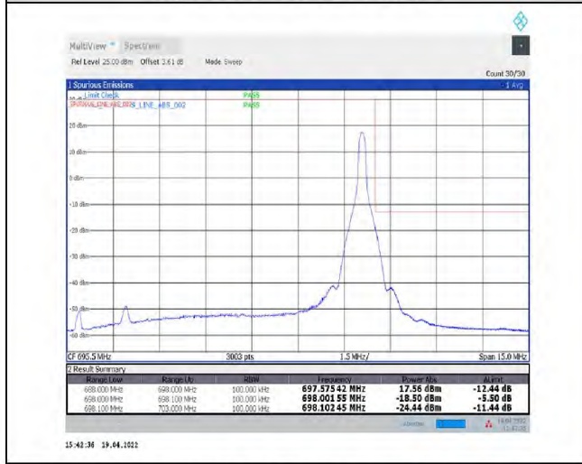
1-N71--15-10-H-5-CP-QPSK-Edge_1RB_Right-1@51-Ant1-PASS-see graph
