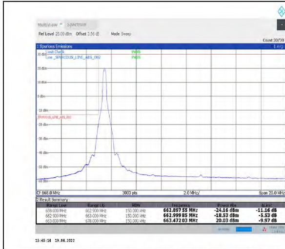
1-N71--15-15-L-1-DFT-PI2BPSK-Edge_1RB_Left-1@0-Ant1-PASS-see graph
