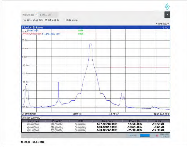
1-N71--15-5-H-2-DFT-PI2BPSK-Edge_1RB_Right-1@24-Ant1-PASS-see graph
