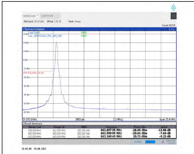
1-N71--15-20-L-1-DFT-PI2BPSK-Edge_1RB_Left-1@0-Ant1-PASS-see graph
