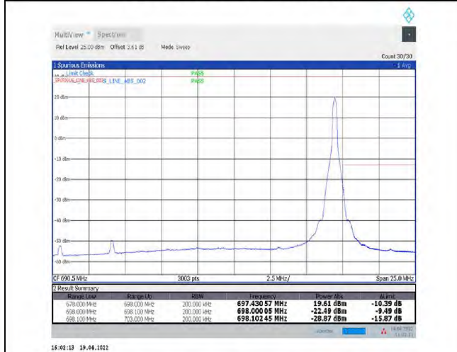
1-N71--15-20-H-5-CP-QPSK-Edge_1RB_Right-1@105-Ant1-PASS-see graph
