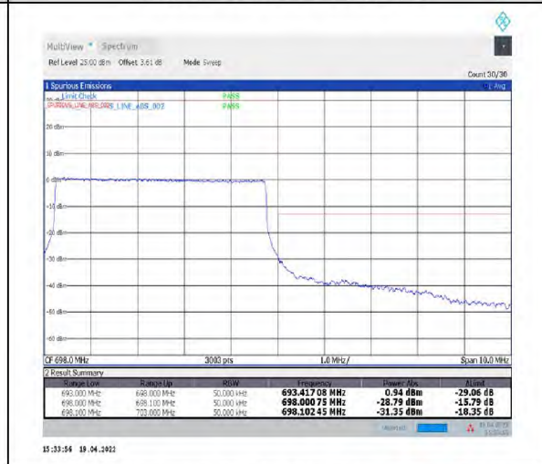
1-N71--15-5-H-6-CP-QPSK-Outer_Full-25@0-Ant1-PASS-see graph
