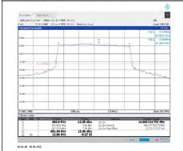
1-N71--15-15-H-7-CP-16QAM-Outer_Full-79@0-Ant1-14.065-15.060-<=15-PASS
