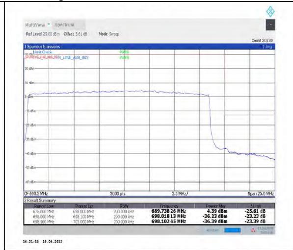
1-N71--15-20-H-3-DFT-PI2BPSK-Outer_Full-100@0-Ant1-PASS-see graph
