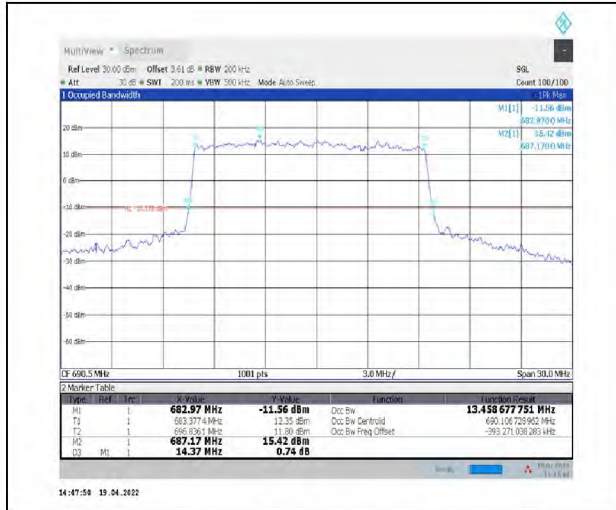
1-N71--15-15-H-1-DFT-QPSK-Outer_Full-75@0- Ant1-13.459-14.370-<=15-PASS
