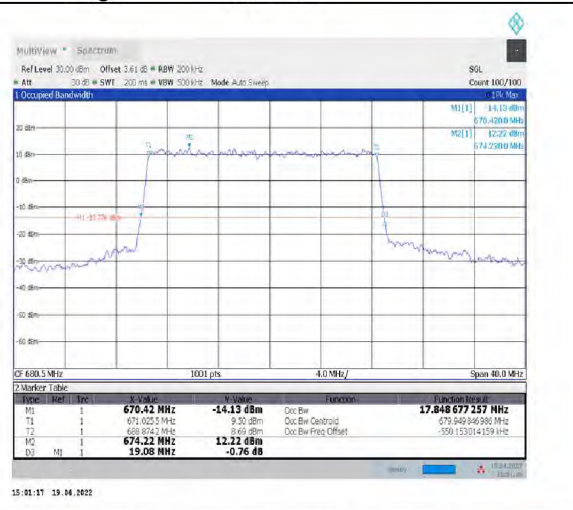
1-N71--15-20-M-4-DFT-64QAM-Outer_Full-100@0-Ant1-17.849-19.080-<20-PASS
