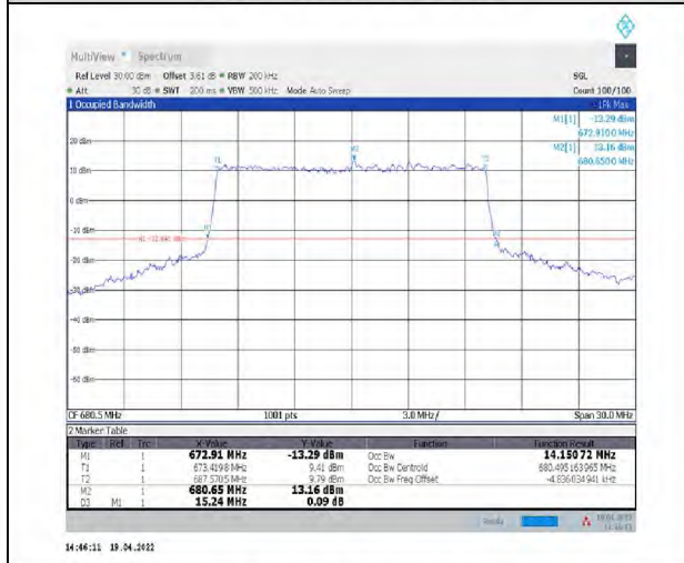
1-N71--15-15-M-8-CP-64QAM-Outer_Full-79@0-Ant1-14.151-15.240-≤15-PASS
