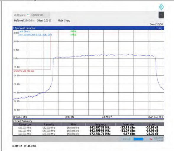
1-N71--15-15-L-3-DFT-PI2BPSK-Outer_Full-75@0-Ant1-PASS-see graph
