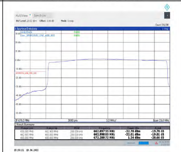
1-N71--15-20-L-6-CP-QPSK-Outer_Full-106@0-Ant1-PASS-see graph
