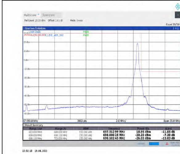
1-N71--15-15-H-5-CP-QPSK-Edge_1RB_Right-1@78-Ant1-PASS-see graph
