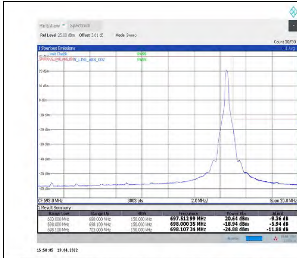
1-N71--15-15-H-2-DFT-PI2BPSK-Edge_1RB_Right-1@78-Ant1-PASS-see graph
