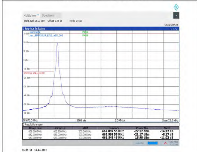
1-N71--15-20-L-4-CP-QPSK-Edge_1RB_Left-1@0-Ant1-PASS-see graph
