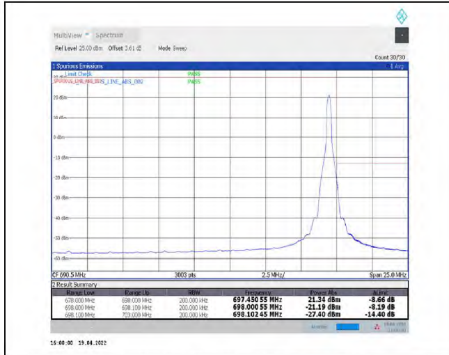
1-N71--15-20-H-2-DFT-PI2BPSK-Edge_1RB_Right-1@105-Ant1-PASS-see graph
