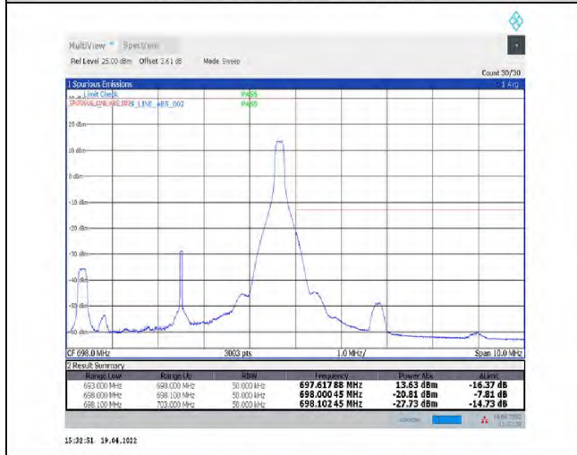
1-N71--15-5-H-5-CP-QPSK-Edge_1RB_Right-1@24-Ant1-PASS-see graph
