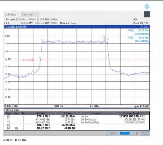
1-N71--15-20-M-2-DFT-PI2BPSK-Outer_Full-100@0-Ant1-17.86-18.920-<20-PASS
