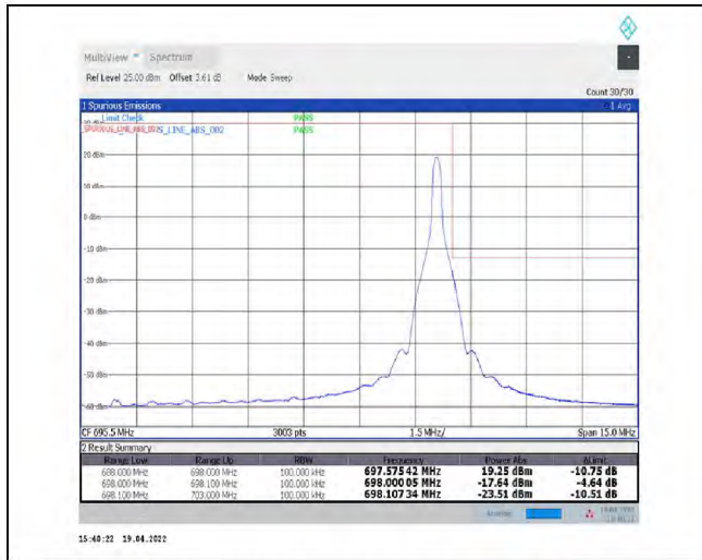
1-N71--15-10-H-2-DFT-PI2BPSK-Edge_1RB_Right-1@51-Ant1-PASS-see graph
