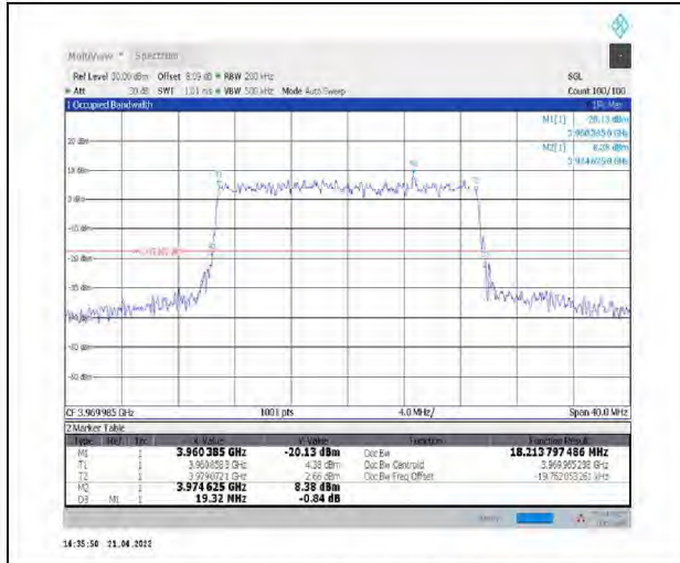
1-N77-3700-3980--30-20-H-9-CP-256QAM-Outer_Full-51@0-Ant1-18,214-19,320-<math>\leq 20</math>-PASS
