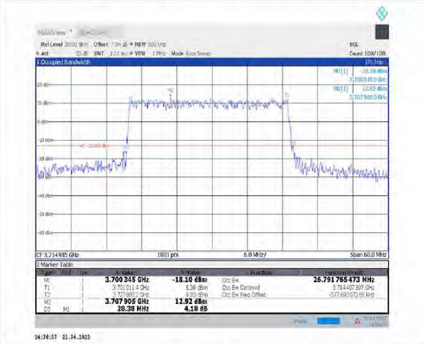
1-N77-3700-3980--30-30-L-3-DFT-16QAM-Outer_Full-75@0-Ant1-26,795-28,380-<math>\leq 30</math>-PASS
