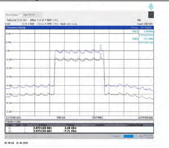
1-N77-3700-3980--30-100-H-2-CP-256QAM-Outer_Full-273@0-Ant1-10.19-100%-0.00-10.19-PASS- \leq 13
