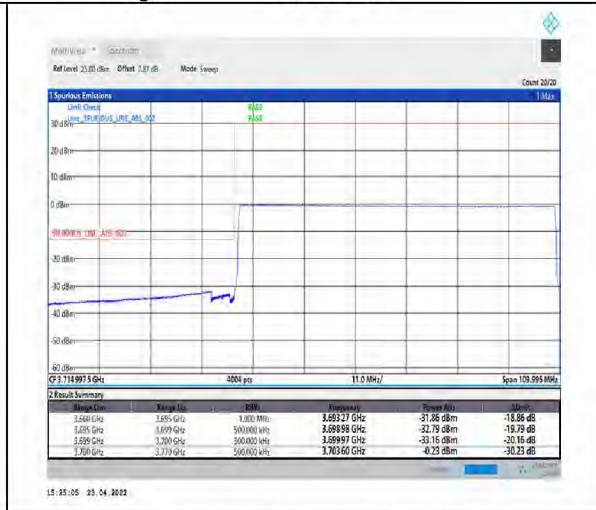
1-N77-3700-3980-PC2-30-70-L-6-CP-QPSK-Outer_Full-189@0-Ant1-PASS-see graph
