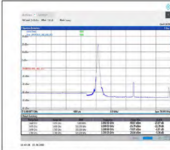
1-N77-3700-3980-PC2-30-40-L-4-CP-QPSK-Edge_1RB_Left-1@0-Ant1-PASS-see graph
