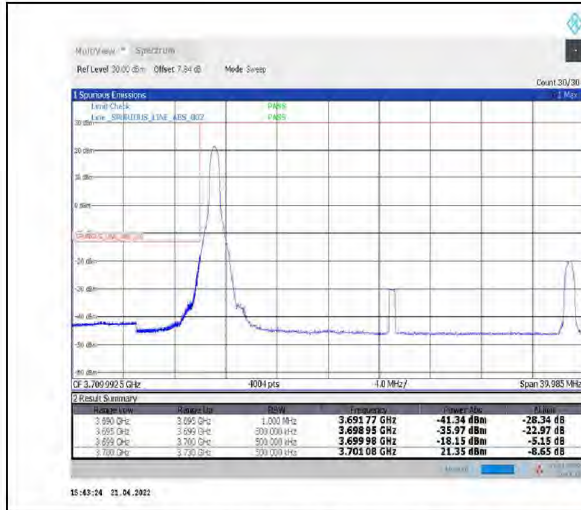
1-N77-3700-3980--30-30-L-1-DFT-PI2BPSK-Edge_1RB_Left-1@0-Ant1-PASS-see graph
