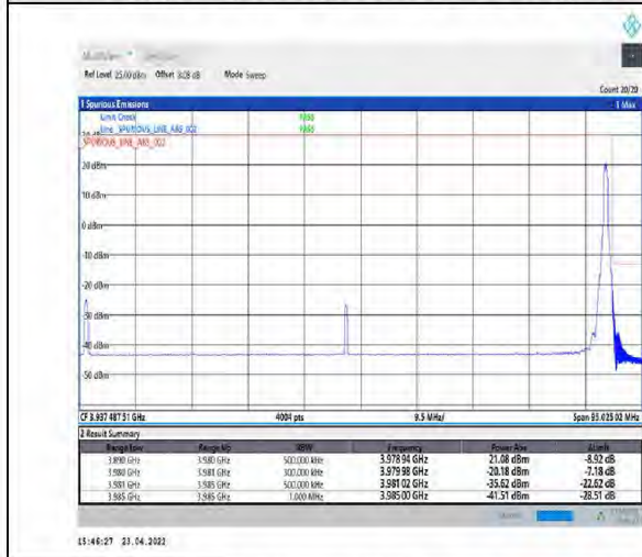
1-N77-3700-3980-PC2-30-90-H-5-CP-QPSK-Edge_1RB_Right-1@244-Ant1-PASS-see graph
