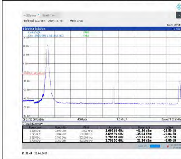
1-N77-3700-3980--30-60-L-4-CP-QPSK-Edge_1RB_Left-1@0-Ant1-PASS-see graph
