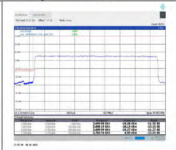
1-N77-3700-3980--30-70-L-3-DFT-PI2BPSK-Outer_Full-180@0-Ant1-PASS-see graph
