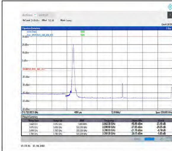
1-N77-3700-3980-PC2-30-80-L-4-CP-QPSK-Edge_1RB_Left-1@0-Ant1-PASS-see graph
