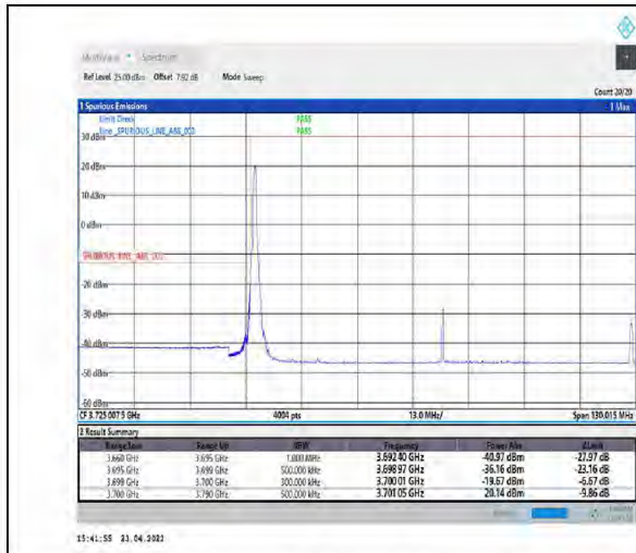
1-N77-3700-3980-PC2-30-90-L-4-CP-QPSK-Edge_1RB_Left-1@0-Ant1-PASS-see graph
