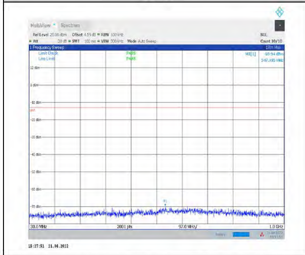
1-N77-3700-3980--30-100-H-1-DFT-PI2BPSK- Inner_1RB_Left-1@1-30-1000-Ant1--69.94--13- PASS
