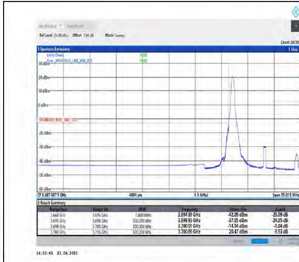
1-N77-3700-3980-PC2-30-15-L-4-CP-QPSK-Edge_1RB_Left-1@0-Ant1-PASS-see graph
