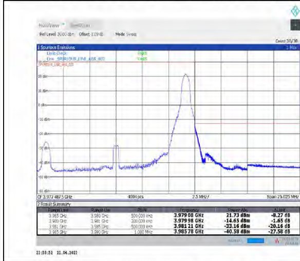
1-N77-3700-3980--30-15-H-5-CP-QPSK-Edge_1RB_Right-1@37-Ant1-PASS-see graph
