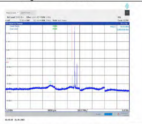
1-N77-3700-3980--30-100-M-1-DFT-PI2BPSK- Inner_1RB_Left-1@1-1000-6000-Ant1--40.56--13- PASS
