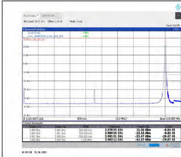
1-N77-3700-3980--30-100-H-2-DFT-PI2BPSK-Edge_1RB_Right-1@272-Ant1-PASS-see graph
