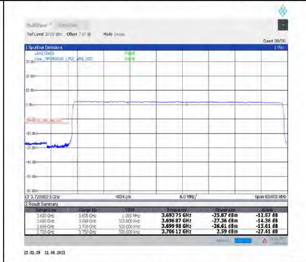
1-N77-3700-3980--30-50-L-6-CP-QPSK-Outer_Full-133@0-Ant1-PASS-see graph
