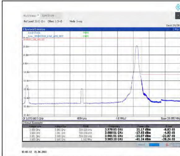
1-N77-3700-3980--30-30-H-2-DFT-PI2BPSK-Edge_1RB_Right-1@77-Ant1-PASS-see graph
