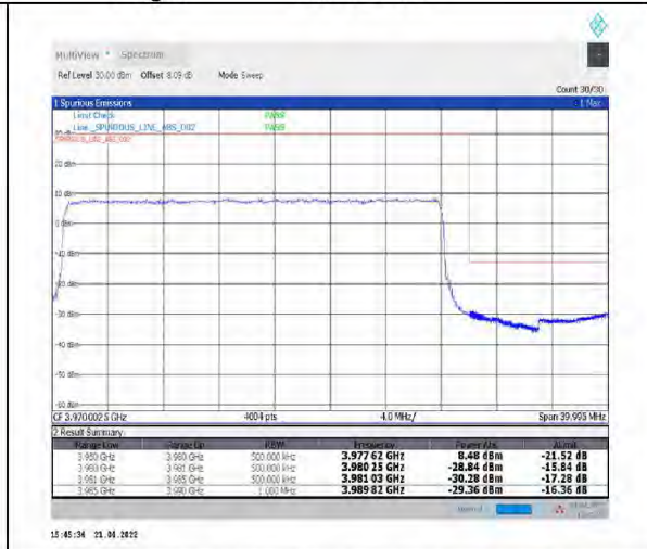
1-N77-3700-3980--30-30-H-3-DFT-PI2BPSK-Outer_Full-75@0-Ant1-PASS-see graph
