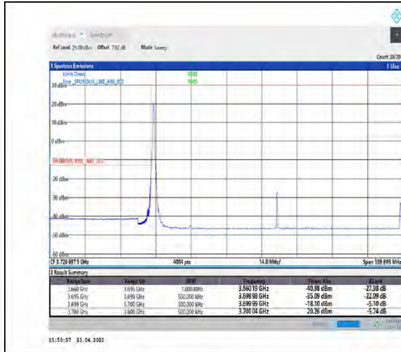
1-N77-3700-3980-PC2-30-100-L-4-CP-QPSK-Edge_1RB_Left-1@0-Ant1-PASS-see graph
