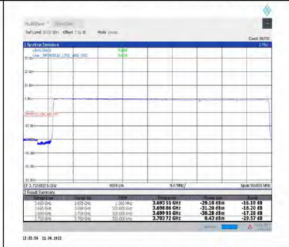
1-N77-3700-3980--30-80-L-6-CP-QPSK-Outer_Full-217@0-Ant1-PASS-see graph
