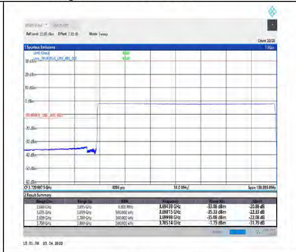
1-N77-3700-3980-PC2-30-100-L-6-CP-QPSK-Outer_Full-273@0-Ant1-PASS-see graph
