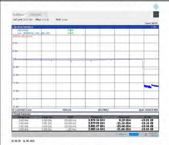
1-N77-3700-3980--30-90-H-6-CP-QPSK-Outer_Full-245@0-Ant1-PASS-see graph
