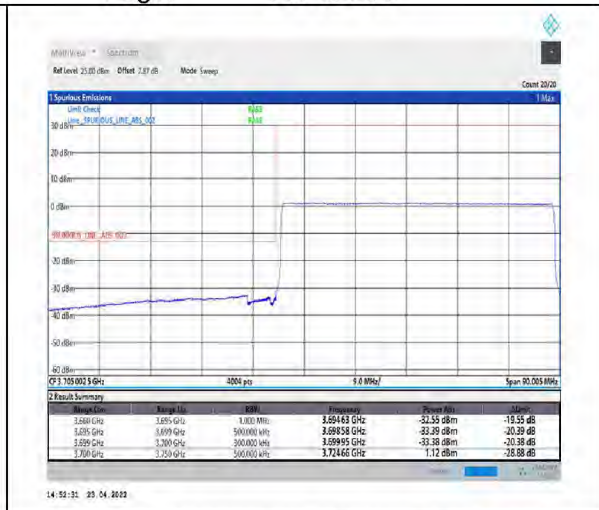
1-N77-3700-3980-PC2-30-50-L-6-CP-QPSK-Outer_Full-133@0-Ant1-PASS-see graph
