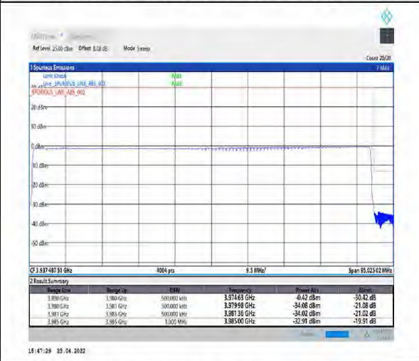
1-N77-3700-3980-PC2-30-90-H-6-CP-QPSK-Outer_Full-245@0-Ant1-PASS-see graph
