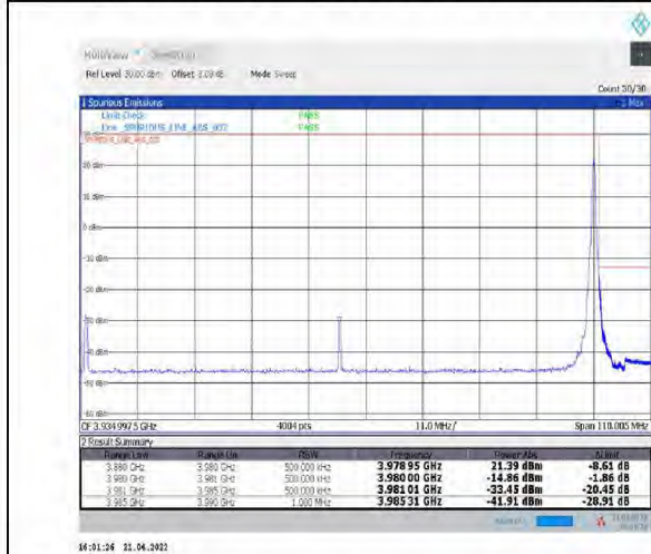
1-N77-3700-3980--30-100-H-5-CP-QPSK-Edge_1RB_Right-1@272-Ant1-PASS-see graph
