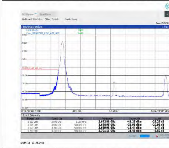
1-N77-3700-3980--30-30-L-4-CP-QPSK-Edge_1RB_Left-1@0-Ant1-PASS-see graph
