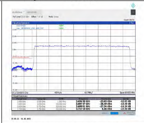
1-N77-3700-3980--30-50-L-3-DFT-PI2BPSK-Outer_Full-128@0-Ant1-PASS-see graph
