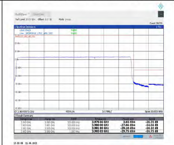
1-N77-3700-3980--30-40-H-6-CP-QPSK-Outer_Full-106@0-Ant1-PASS-see graph
