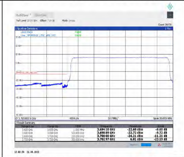
1-N77-3700-3980--30-20-L-6-CP-QPSK-Outer_Full-51@0-Ant1-PASS-see graph
