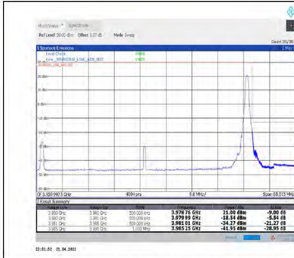
1-N77-3700-3980--30-50-H-2-DFT-PI2BPSK-Edge_1RB_Right-1@132-Ant1-PASS-see graph
