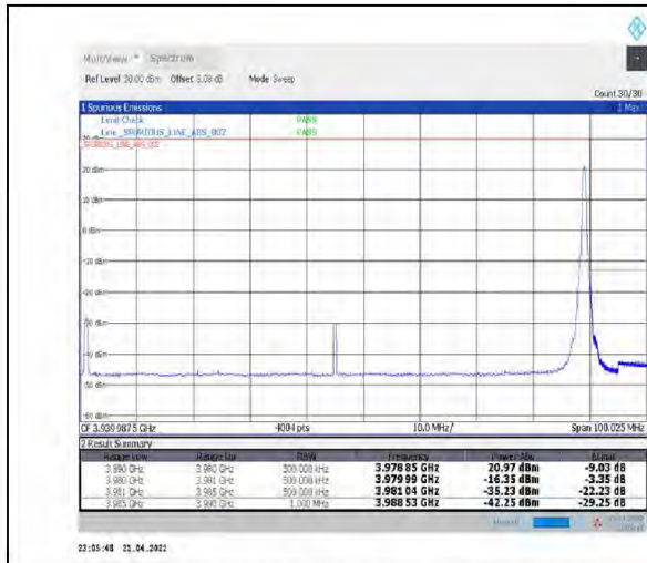
1-N77-3700-3980--30-90-H-2-DFT-PI2BPSK-Edge_1RB_Right-1@244-Ant1-PASS-see graph
