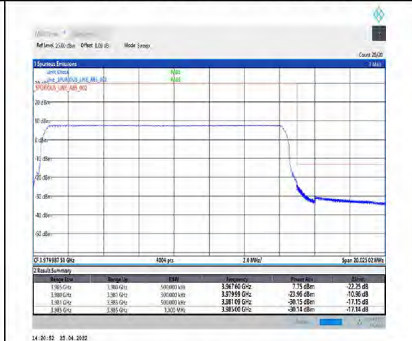
1-N77-3700-3980-PC2-30-15-H-6-CP-QPSK-Outer_Full-38@0-Ant1-PASS-see graph
