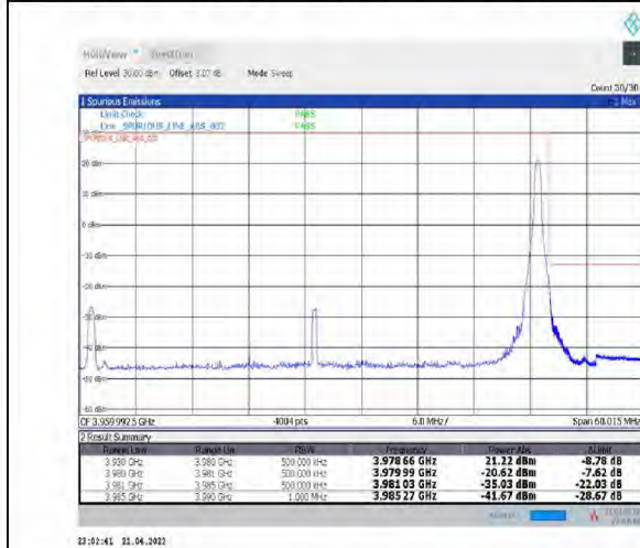
1-N77-3700-3980--30-50-H-5-CP-QPSK-Edge_1RB_Right-1@132-Ant1-PASS-see graph
