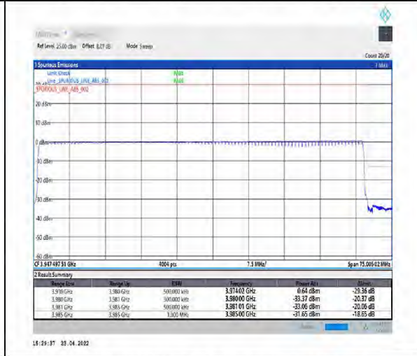
1-N77-3700-3980-PC2-30-70-H-6-CP-QPSK-Outer_Full-189@0-Ant1-PASS-see graph
