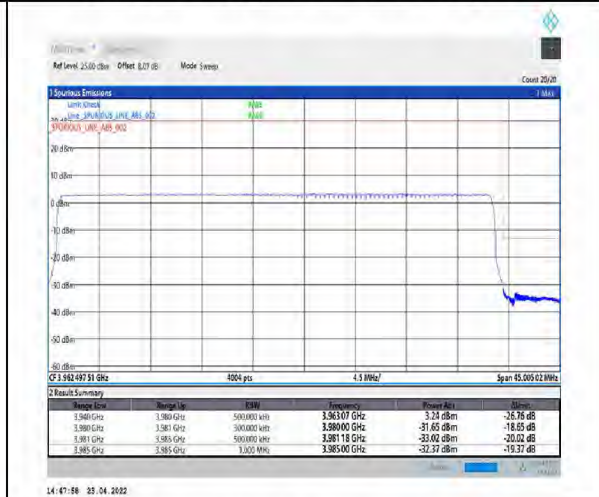
1-N77-3700-3980-PC2-30-40-H-6-CP-QPSK-Outer_Full-106@0-Ant1-PASS-see graph
