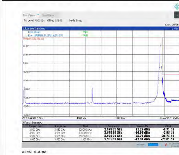
1-N77-3700-3980--30-80-H-5-CP-QPSK-Edge_1RB_Right-1@216-Ant1-PASS-see graph
