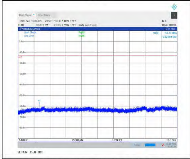
1-N77-3700-3980--30-100-M-1-DFT-PI2BPSK- Inner_1RB_Left-1@1-6000-18000-Ant1--58.13--13- PASS
