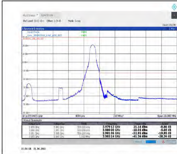
1-N77-3700-3980--30-10-H-2-DFT-PI2BPSK-Edge_1RB_Right-1@23-Ant1-PASS-see graph
