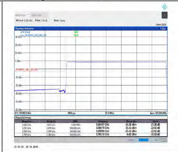
1-N77-3700-3980-PC2-30-80-L-6-CP-QPSK-Outer_Full-217@0-Ant1-PASS-see graph
