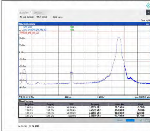
1-N77-3700-3980-PC2-30-20-H-5-CP-QPSK-Edge_1RB_Right-1@50-Ant1-PASS-see graph
