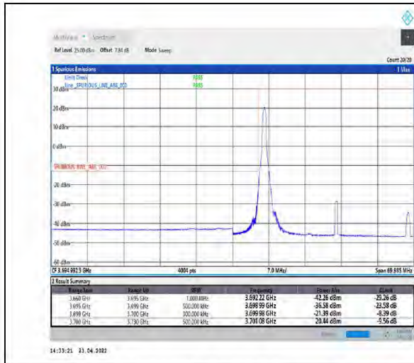
1-N77-3700-3980-PC2-30-30-L-4-CP-QPSK-Edge_1RB_Left-1@0-Ant1-PASS-see graph
