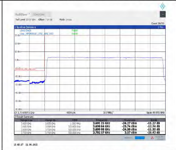
1-N77-3700-3980--30-40-L-6-CP-QPSK-Outer_Full-106@0-Ant1-PASS-see graph
