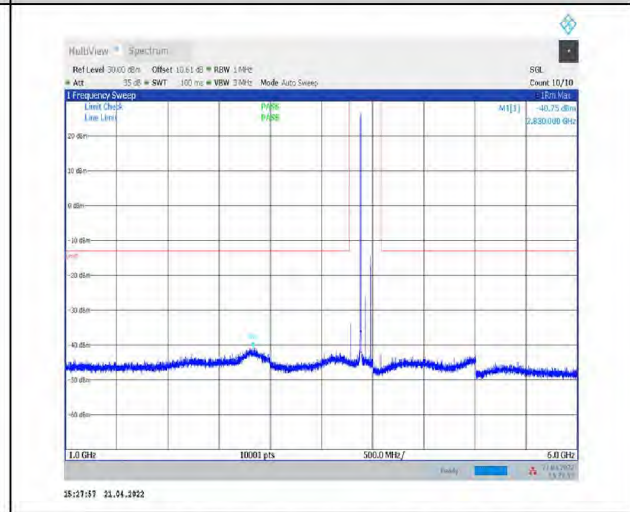
1-N77-3700-3980--30-100-H-1-DFT-PI2BPSK- Inner_1RB_Left-1@1-1000-6000-Ant1--40.75--13- PASS
