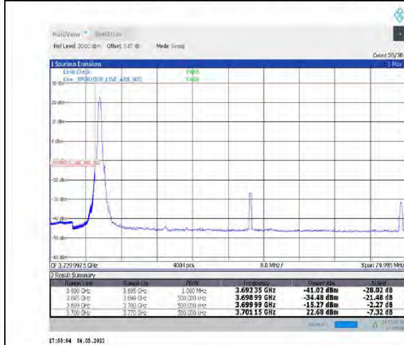
1-N77-3700-3980--30-70-L-4-CP-QPSK-Edge_1RB_Left-1@0-Ant1-PASS-see graph
