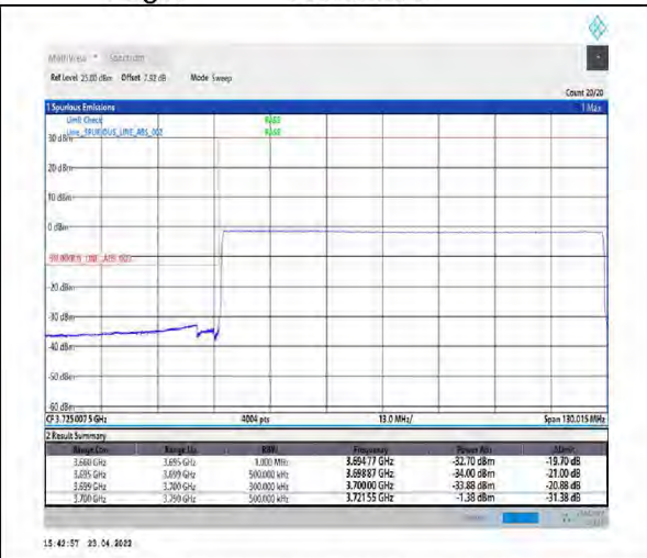
1-N77-3700-3980-PC2-30-90-L-6-CP-QPSK-Outer_Full-245@0-Ant1-PASS-see graph
