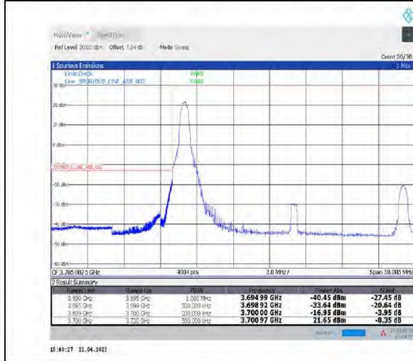
1-N77-3700-3980--30-20-L-4-CP-QPSK-Edge_1RB_Left-1@0-Ant1-PASS-see graph
