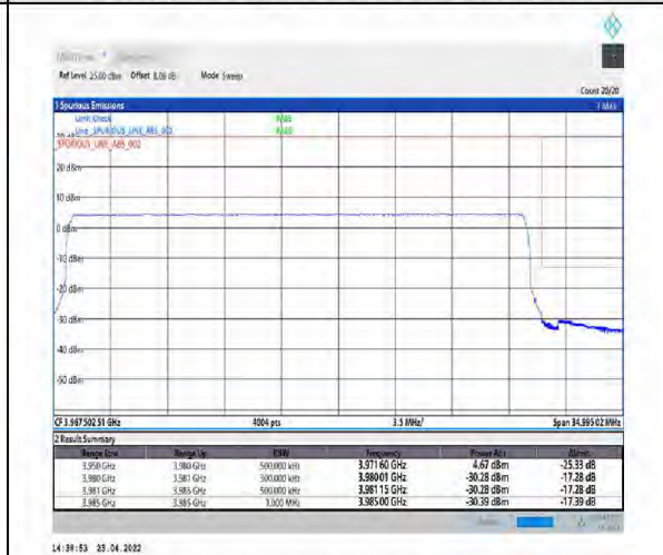
1-N77-3700-3980-PC2-30-30-H-6-CP-QPSK-Outer_Full-78@0-Ant1-PASS-see graph
