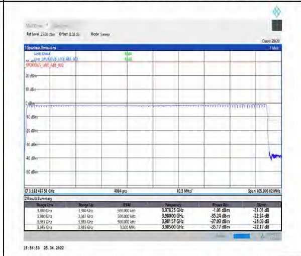
1-N77-3700-3980-PC2-30-100-H-6-CP-QPSK-Outer_Full-273@0-Ant1-PASS-see graph
