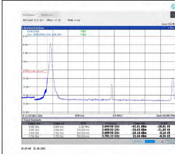
1-N77-3700-3980--30-50-L-4-CP-QPSK-Edge_1RB_Left-1@0-Ant1-PASS-see graph
