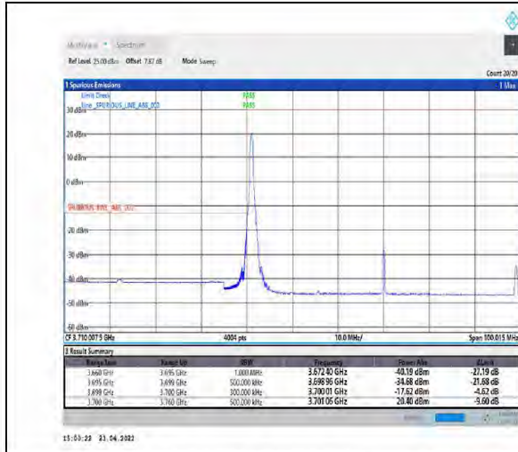
1-N77-3700-3980-PC2-30-60-L-4-CP-QPSK-Edge_1RB_Left-1@0-Ant1-PASS-see graph
