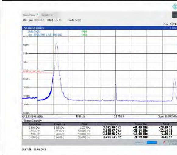
1-N77-3700-3980--30-40-L-4-CP-QPSK-Edge_1RB_Left-1@0-Ant1-PASS-see graph
