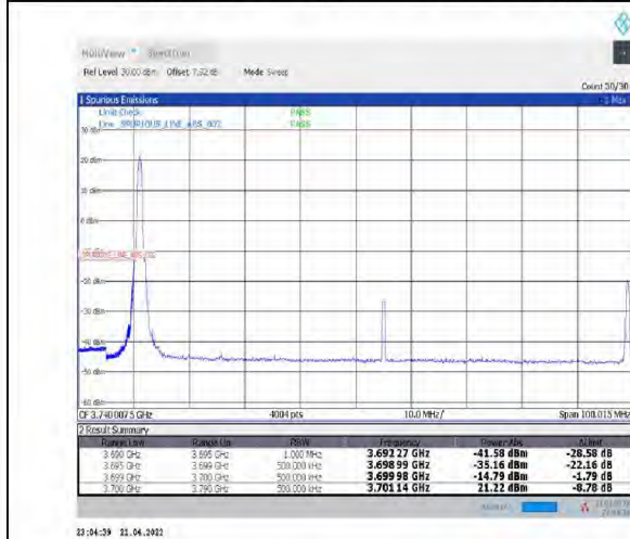
1-N77-3700-3980--30-90-L-4-CP-QPSK-Edge_1RB_Left-1@0-Ant1-PASS-see graph
