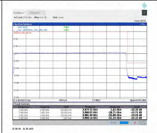
1-N77-3700-3980--30-60-H-6-CP-QPSK-Outer_Full-162@0-Ant1-PASS-see graph
