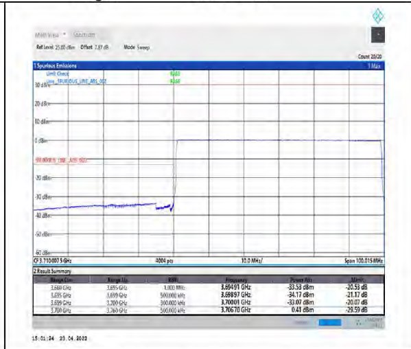
1-N77-3700-3980-PC2-30-60-L-6-CP-QPSK-Outer_Full-162@0-Ant1-PASS-see graph
