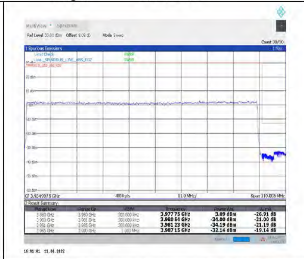
1-N77-3700-3980--30-100-H-3-DFT-PI2BPSK-Outer_Full-270@0-Ant1-PASS-see graph
