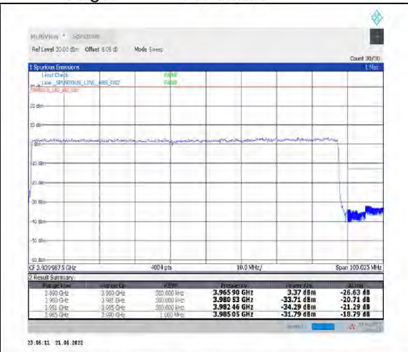
1-N77-3700-3980--30-90-H-3-DFT-PI2BPSK-Outer_Full-240@0-Ant1-PASS-see graph
