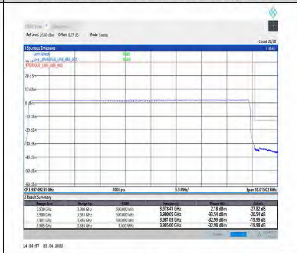
1-N77-3700-3980-PC2-30-50-H-6-CP-QPSK-Outer_Full-133@0-Ant1-PASS-see graph
