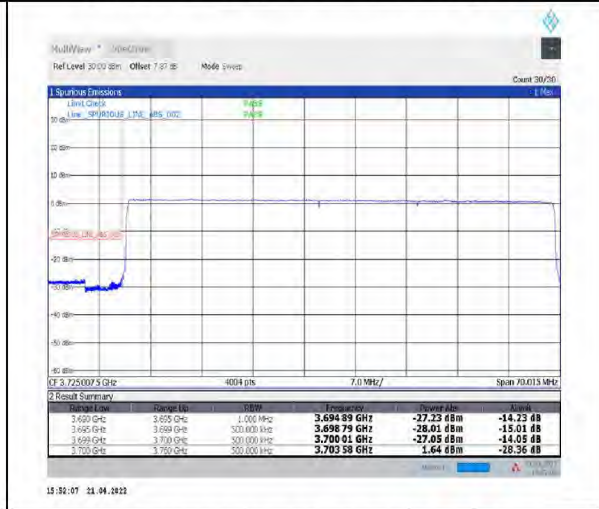
1-N77-3700-3980--30-60-L-6-CP-QPSK-Outer_Full-162@0-Ant1-PASS-see graph
