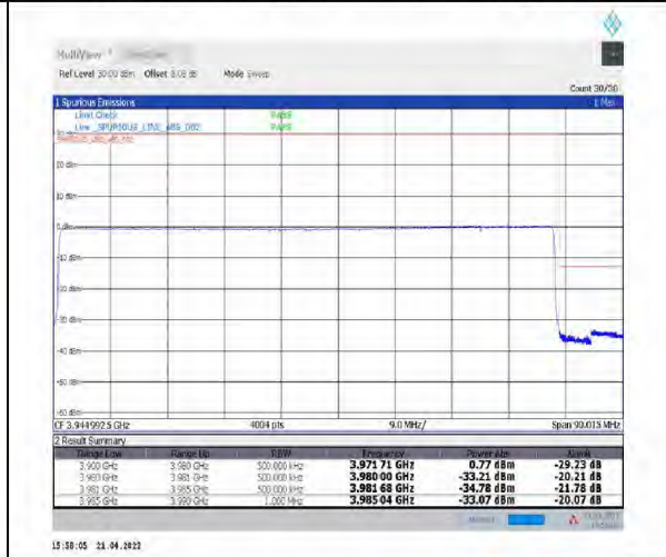
1-N77-3700-3980--30-80-H-6-CP-QPSK-Outer_Full-217@0-Ant1-PASS-see graph
