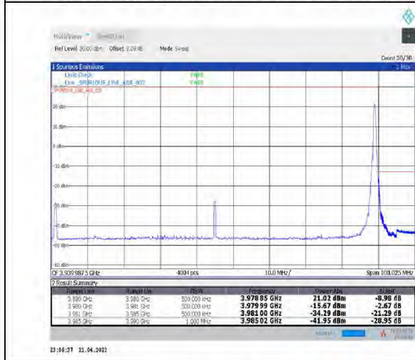
1-N77-3700-3980--30-90-H-5-CP-QPSK-Edge_1RB_Right-1@244-Ant1-PASS-see graph
