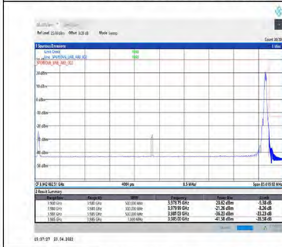
1-N77-3700-3980-PC2-30-80-H-5-CP-QPSK-Edge_1RB_Right-1@216-Ant1-PASS-see graph
