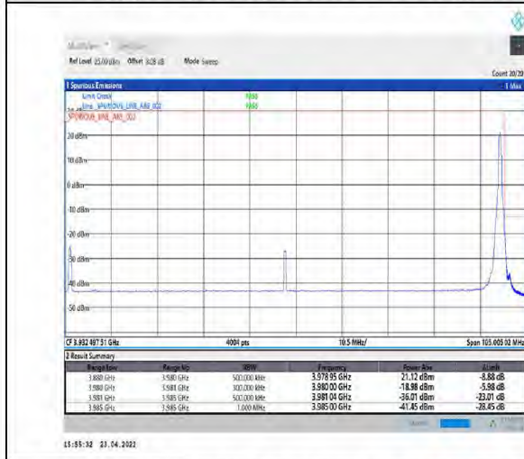
1-N77-3700-3980-PC2-30-100-H-5-CP-QPSK-Edge_1RB_Right-1@272-Ant1-PASS-see graph
