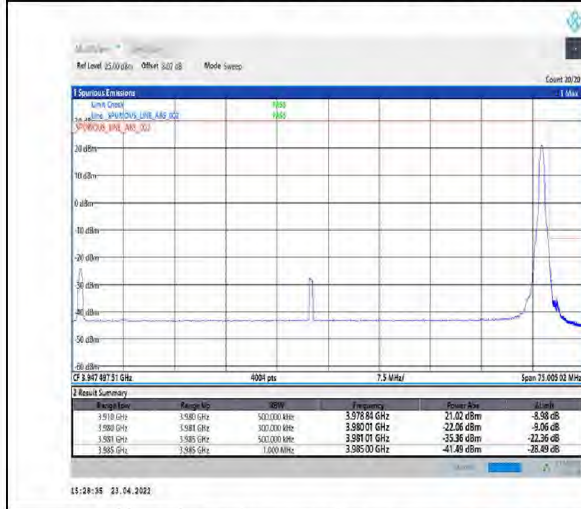
1-N77-3700-3980-PC2-30-70-H-5-CP-QPSK-Edge_1RB_Right-1@188-Ant1-PASS-see graph
