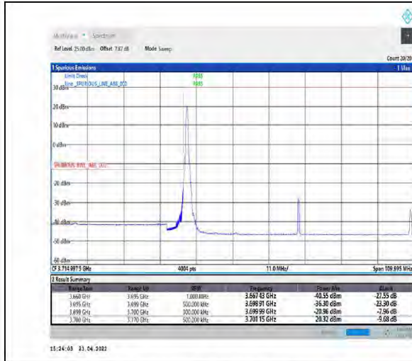
1-N77-3700-3980-PC2-30-70-L-4-CP-QPSK-Edge_1RB_Left-1@0-Ant1-PASS-see graph
