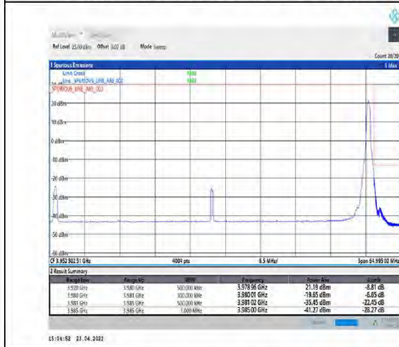
1-N77-3700-3980-PC2-30-60-H-5-CP-QPSK-Edge_1RB_Right-1@161-Ant1-PASS-see graph
