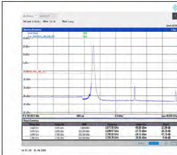
1-N77-3700-3980-PC2-30-50-L-4-CP-QPSK-Edge_1RB_Left-1@0-Ant1-PASS-see graph
