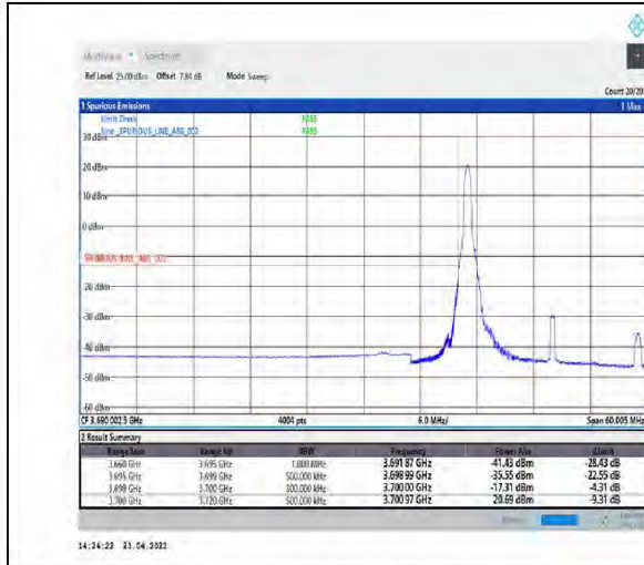
1-N77-3700-3980-PC2-30-20-L-4-CP-QPSK-Edge_1RB_Left-1@0-Ant1-PASS-see graph
