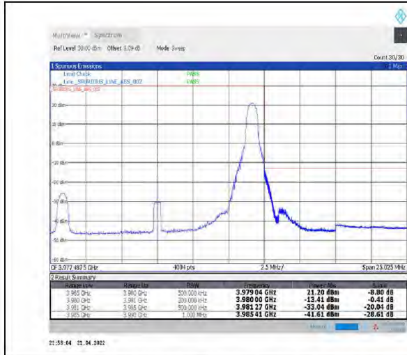
1-N77-3700-3980--30-15-H-2-DFT-PI2BPSK-Edge_1RB_Right-1@37-Ant1-PASS-see graph
