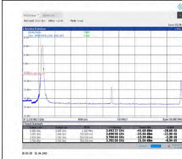
1-N77-3700-3980--30-80-L-4-CP-QPSK-Edge_1RB_Left-1@0-Ant1-PASS-see graph
