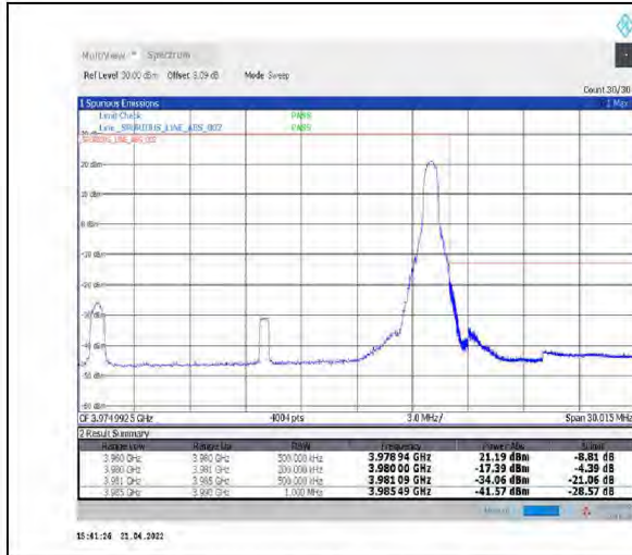
1-N77-3700-3980--30-20-H-2-DFT-PI2BPSK-Edge_1RB_Right-1@50-Ant1-PASS-see graph
