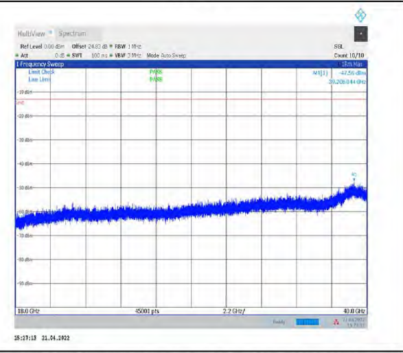
1-N77-3700-3980--30-100-M-1-DFT-PI2BPSK- Inner_1RB_Left-1@1-18000-40000-Ant1--47.56--13- PASS
