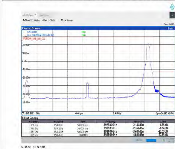
1-N77-3700-3980-PC2-30-30-H-5-CP-QPSK-Edge_1RB_Right-1@77-Ant1-PASS-see graph
