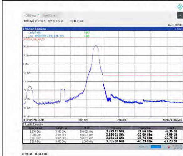
1-N77-3700-3980--30-10-H-5-CP-QPSK-Edge_1RB_Right-1@23-Ant1-PASS-see graph
