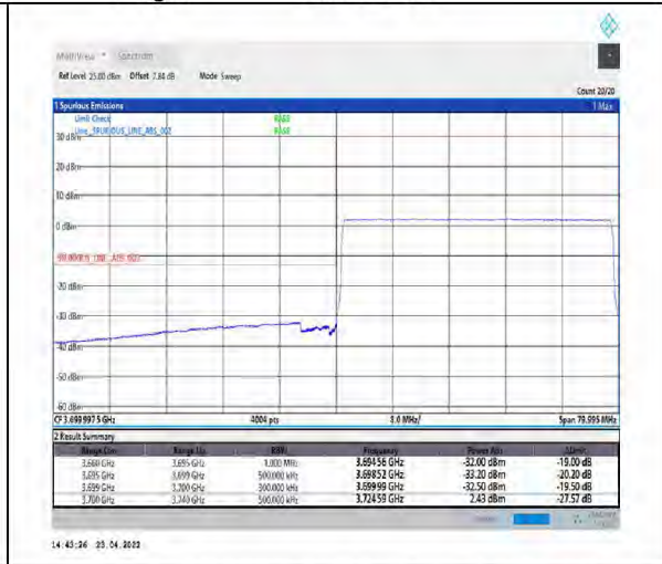
1-N77-3700-3980-PC2-30-40-L-6-CP-QPSK-Outer_Full-106@0-Ant1-PASS-see graph
