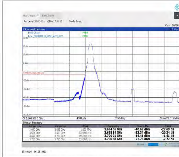
1-N77-3700-3980--30-15-L-1-DFT-PI2BPSK-Edge_1RB_Left-1@0-Ant1-PASS-see graph
