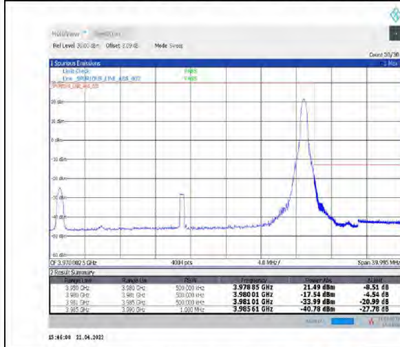
1-N77-3700-3980--30-30-H-5-CP-QPSK-Edge_1RB_Right-1@77-Ant1-PASS-see graph
