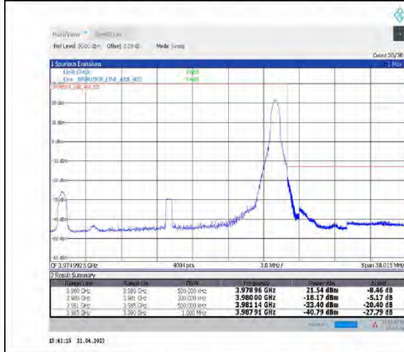
1-N77-3700-3980--30-20-H-5-CP-QPSK-Edge_1RB_Right-1@50-Ant1-PASS-see graph
