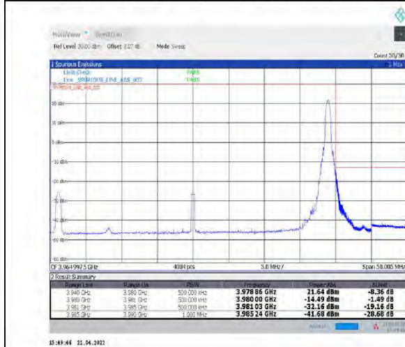
1-N77-3700-3980--30-40-H-5-CP-QPSK-Edge_1RB_Right-1@105-Ant1-PASS-see graph
