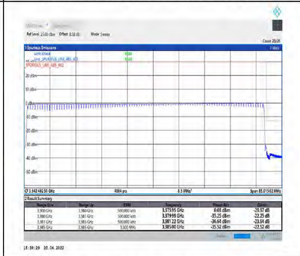
1-N77-3700-3980-PC2-30-80-H-6-CP-QPSK-Outer_Full-217@0-Ant1-PASS-see graph
