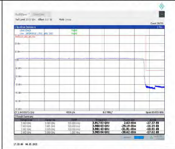
1-N77-3700-3980--30-70-H-6-CP-QPSK-Outer_Full-189@0-Ant1-PASS-see graph
