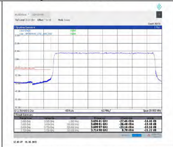
1-N77-3700-3980--30-30-L-3-DFT-PI2BPSK-Outer_Full-75@0-Ant1-PASS-see graph
