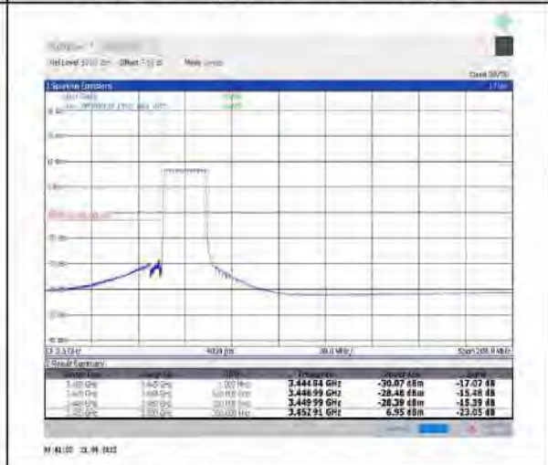
1-N78-3450-3550-30-20-L-6-CP-QPSK-Outer_Full-51@0-Ant1-PASS-see graph
