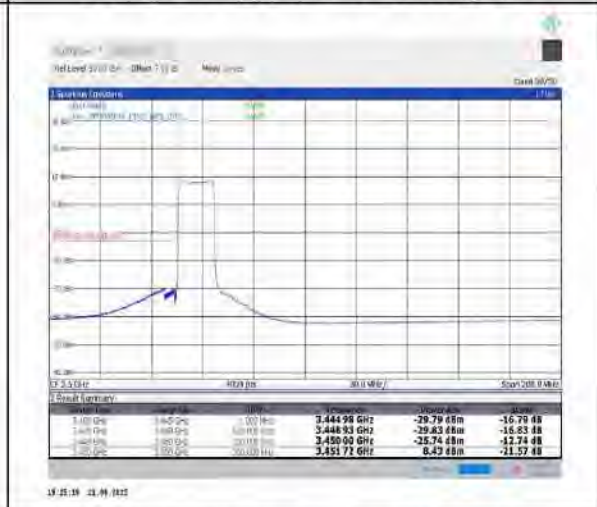
1-N78-3450-3550-30-15-L-6-CP-QPSK-Outer_Full-38@0-Ant1-PASS-see graph
