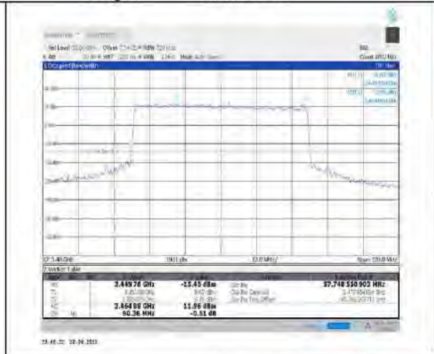
1-N78-3450-3550--30-60-L-8-CP-64QAM-Outer_Full-162@0-Ant1-57.749-60.360-≤60-PASS
