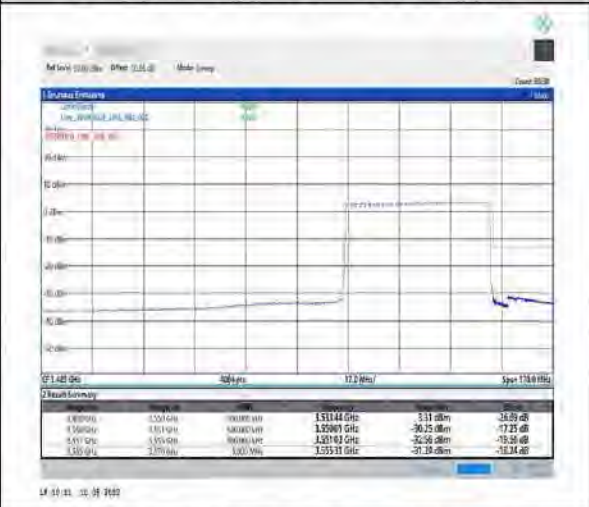
1-N78-3450-3550-PC2-30-50-H-6-CP-QPSK-Outer_Full-133@0-Ant1-PASS-see graph
