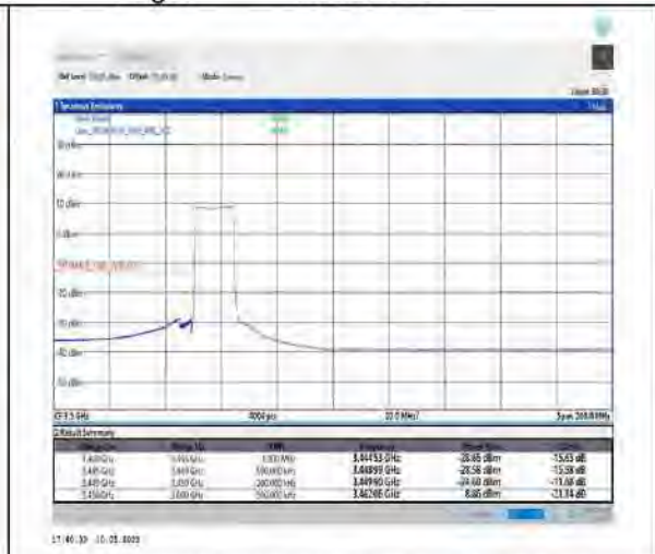
1-N78-3450-3550-PC2-30-15-L-6-CP-QPSK-Outer_Full-38@0-Ant1-PASS-see graph
