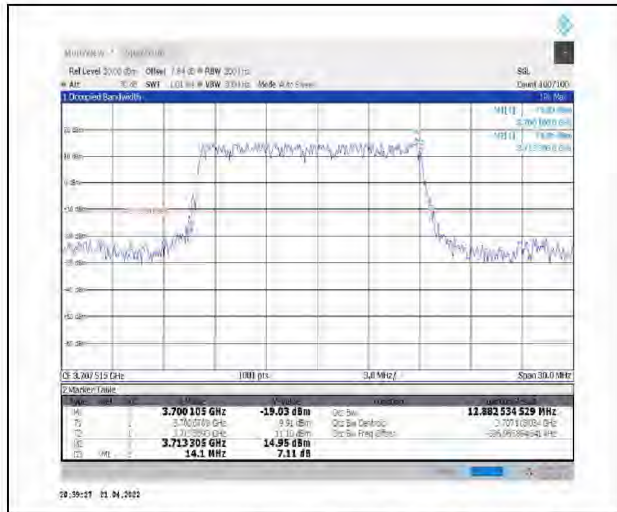
1-N78-3700-3800--30-15-L-2-DFT-PI2BPSK-Outer_Full-36@0-Ant1-12.883-14.100-<=15-PASS
