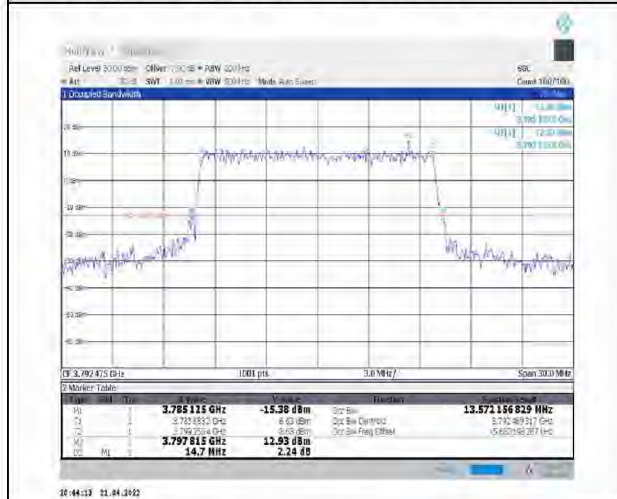
1-N78-3700-3800--30-15-H-6-CP-QPSK-Outer_Full-38@0-Ant1-13.572-14.700-≤15-PASS
