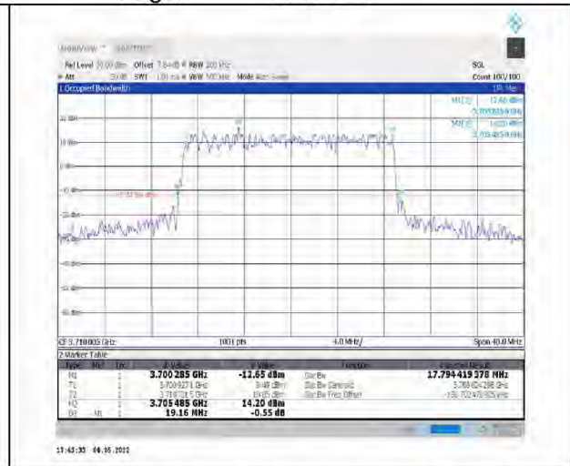
1-N78-3700-3800--30-20-L-4-DFT-64QAM-Outer_Full-50@0-Ant1-17.794-19.160-<20-PASS
