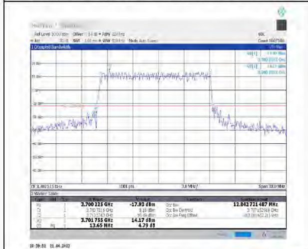
1-N78-3700-3800--30-15-L-4-DFT-64QAM-Outer_Full-36@0-Ant1-12.843-13.650-<=15-PASS
