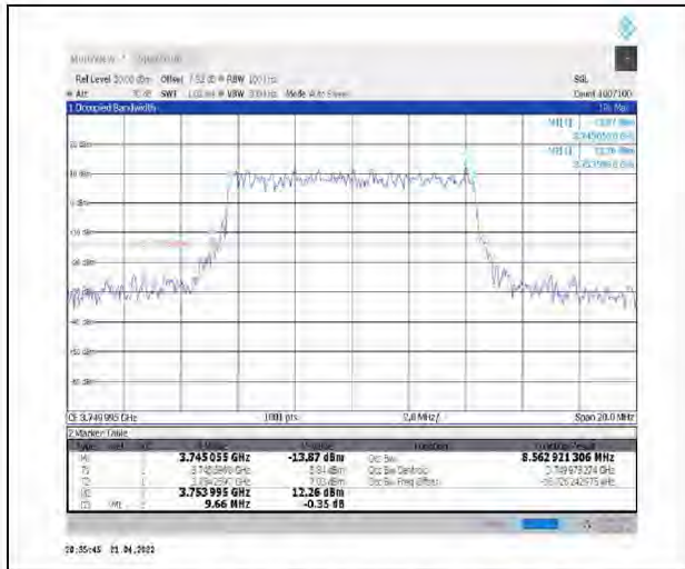
1-N78-3700-3800--30-10-M-4-DFT-64QAM-Outer_Full-24@0-Ant1-8.563-9.660-≤10-PASS
