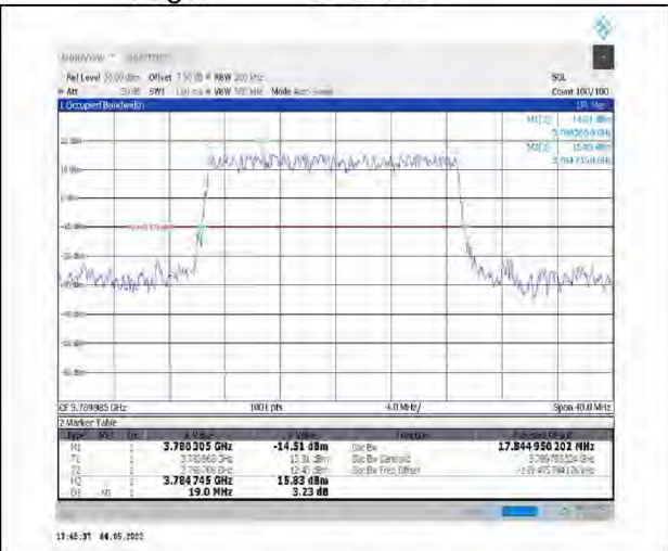
1-N78-3700-3800--30-20-H-2-DFT-PI2BPSK-Outer_Full-50@0-Ant1-17.845-19.000-<20-PASS
