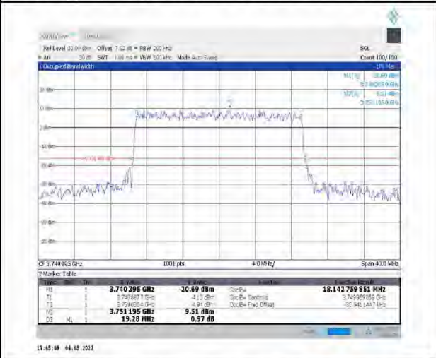
1-N78-3700-3800--30-20-M-9-CP-256QAM-Outer_Full-51@0-Ant1-18.143-19.280-<20-PASS
