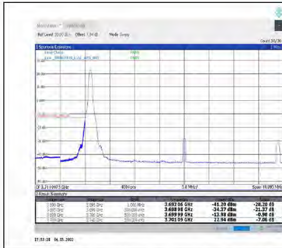
1-N78-3700-3800--30-40-L-1-DFT-PI2BPSK-Edge_1RB_Left-1@0-Ant1-PASS-see graph
