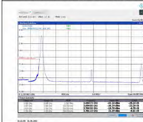
1-N78-3700-3800--30-50-L-4-CP-QPSK-Edge_1RB_Left-1@0-Ant1-PASS-see graph
