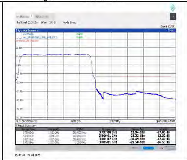
1-N78-3700-3800--30-10-H-3-DFT-PI2BPSK-Outer_Full-24@0-Ant1-PASS-see graph
