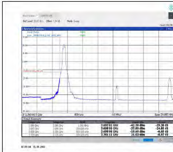
1-N78-3700-3800--30-30-L-1-DFT-PI2BPSK-Edge_1RB_Left-1@0-Ant1-PASS-see graph
