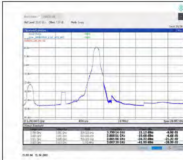
1-N78-3700-3800--30-10-H-2-DFT-PI2BPSK-Edge_1RB_Right-1@23-Ant1-PASS-see graph
