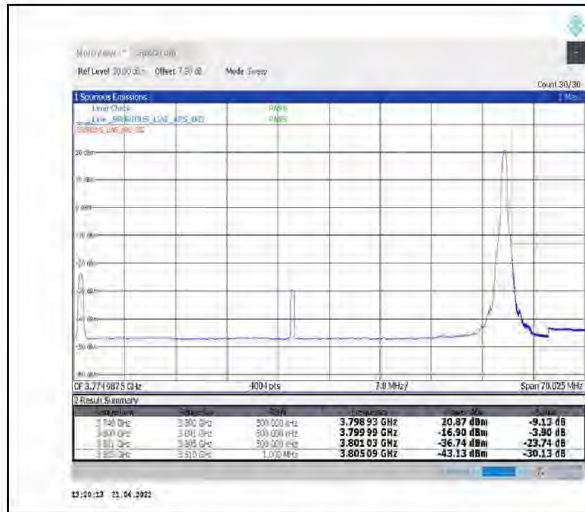
1-N78-3700-3800--30-60-H-2-DFT-PI2BPSK-Edge_1RB_Right-1@161-Ant1-PASS-see graph
