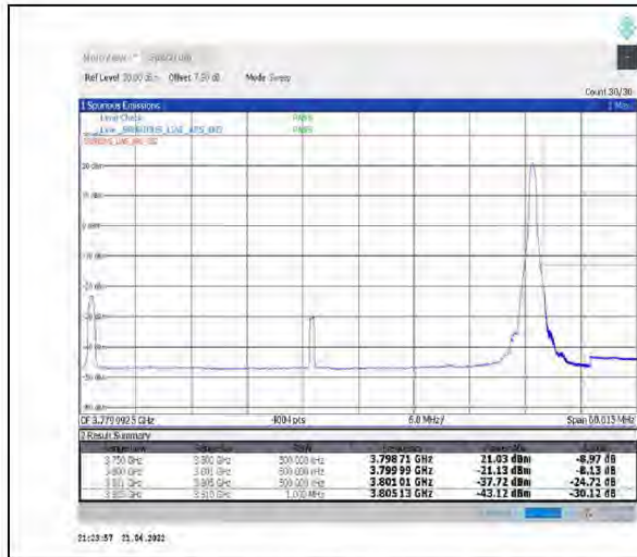
1-N78-3700-3800--30-50-H-2-DFT-PI2BPSK-Edge_1RB_Right-1@132-Ant1-PASS-see graph
