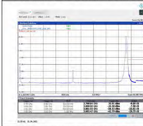
1-N78-3700-3800--30-70-H-5-CP-QPSK-Edge_1RB_Right-1@188-Ant1-PASS-see graph
