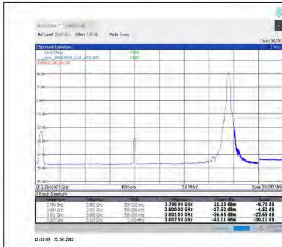
1-N78-3700-3800--30-40-H-2-DFT-PI2BPSK-Edge_1RB_Right-1@105-Ant1-PASS-see graph
