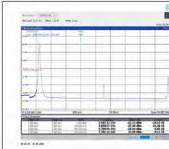
1-N78-3700-3800--30-80-L-1-DFT-PI2BPSK-Edge_1RB_Left-1@0-Ant1-PASS-see graph
