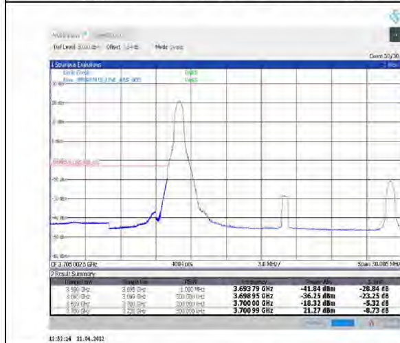
1-N78-3700-3800--30-20-L-4-CP-QPSK-Edge_1RB_Left-1@0-Ant1-PASS-see graph
