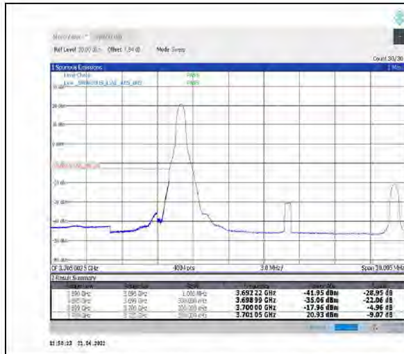
1-N78-3700-3800--30-20-L-1-DFT-PI2BPSK-Edge_1RB_Left-1@0-Ant1-PASS-see graph
