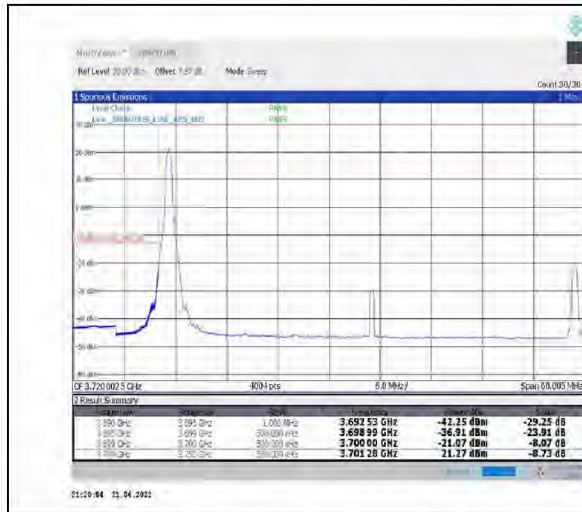
1-N78-3700-3800--30-50-L-1-DFT-PI2BPSK-Edge_1RB_Left-1@0-Ant1-PASS-see graph
