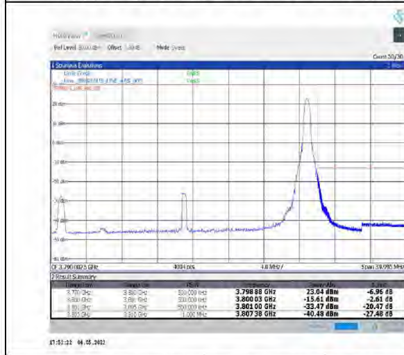
1-N78-3700-3800--30-30-H-5-CP-QPSK-Edge_1RB_Right-1@77-Ant1-PASS-see graph
