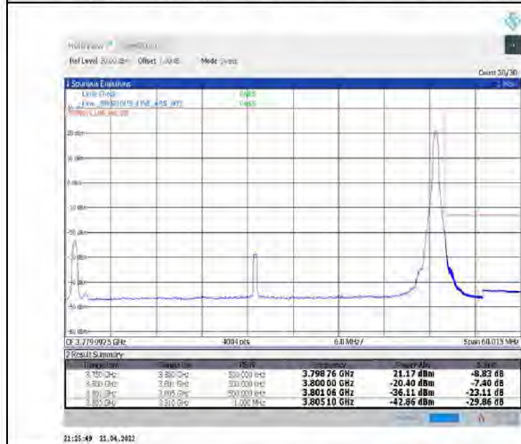
1-N78-3700-3800--30-50-H-5-CP-QPSK-Edge_1RB_Right-1@132-Ant1-PASS-see graph
