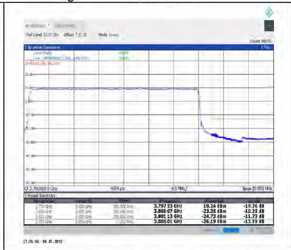
1-N78-3700-3800--30-30-H-3-DFT-PI2BPSK-Outer_Full-75@0-Ant1-PASS-see graph
