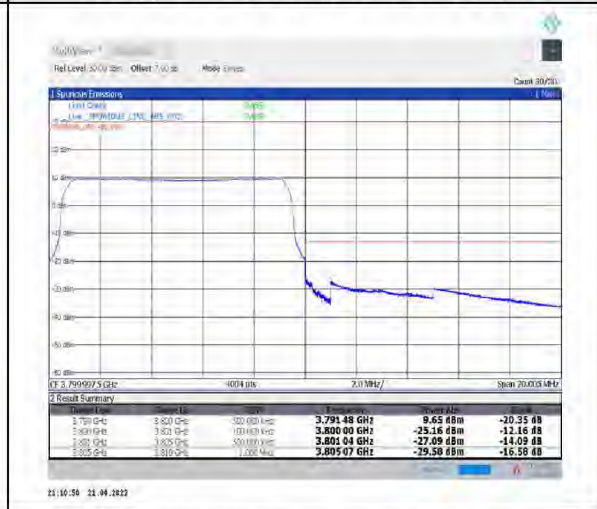
1-N78-3700-3800--30-10-H-6-CP-QPSK-Outer_Full-24@0-Ant1-PASS-see graph
