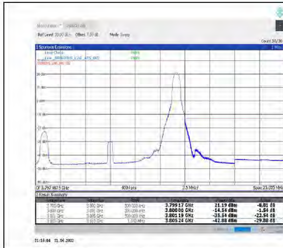
1-N78-3700-3800--30-15-H-2-DFT-PI2BPSK-Edge_1RB_Right-1@37-Ant1-PASS-see graph
