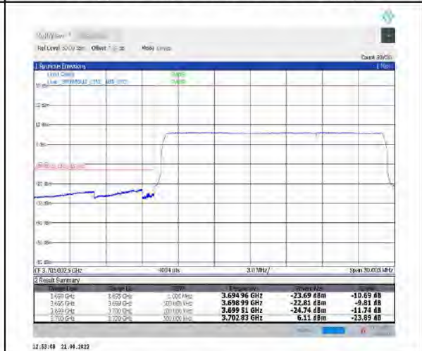
1-N78-3700-3800--30-20-L-6-CP-QPSK-Outer_Full-51@0-Ant1-PASS-see graph
