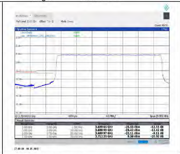
1-N78-3700-3800--30-30-L-3-DFT-PI2BPSK-Outer_Full-75@0-Ant1-PASS-see graph
