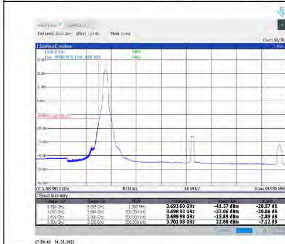
1-N78-3700-3800--30-30-L-4-CP-QPSK-Edge_1RB_Left-1@0-Ant1-PASS-see graph
