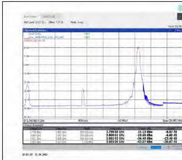
1-N78-3700-3800--30-30-H-2-DFT-PI2BPSK-Edge_1RB_Right-1@77-Ant1-PASS-see graph
