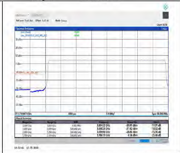
1-N78-3700-3800-PC2-30-40-L-6-CP-QPSK-Outer_Full-106@0-Ant1-PASS-see graph
