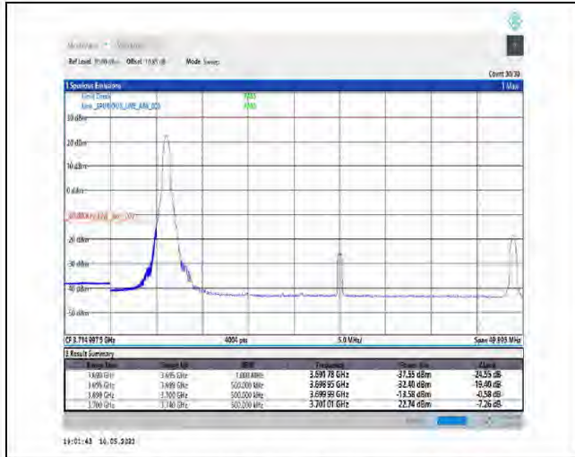
1-N78-3700-3800-PC2-30-40-L-4-CP-QPSK-Edge_1RB_Left-1@0-Ant1-PASS-see graph
