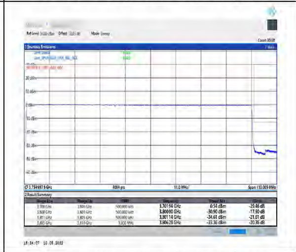
1-N78-3700-3800-PC2-30-100-H-6-CP-QPSK-Outer_Full-273@0-Ant1-PASS-see graph
