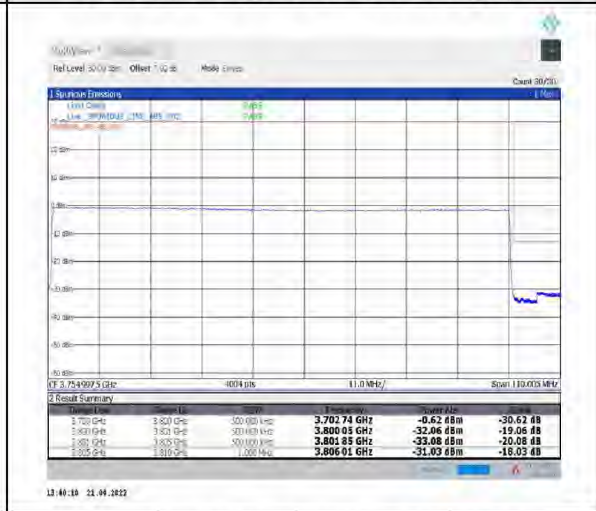
1-N78-3700-3800--30-100-H-6-CP-QPSK-Outer_Full-273@0-Ant1-PASS-see graph
