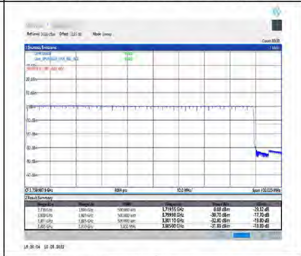
1-N78-3700-3800-PC2-30-90-H-6-CP-QPSK-Outer_Full-245@0-Ant1-PASS-see graph
