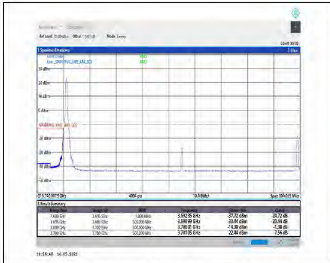
1-N78-3700-3800-PC2-30-90-L-4-CP-QPSK-Edge_1RB_Left-1@0-Ant1-PASS-see graph
