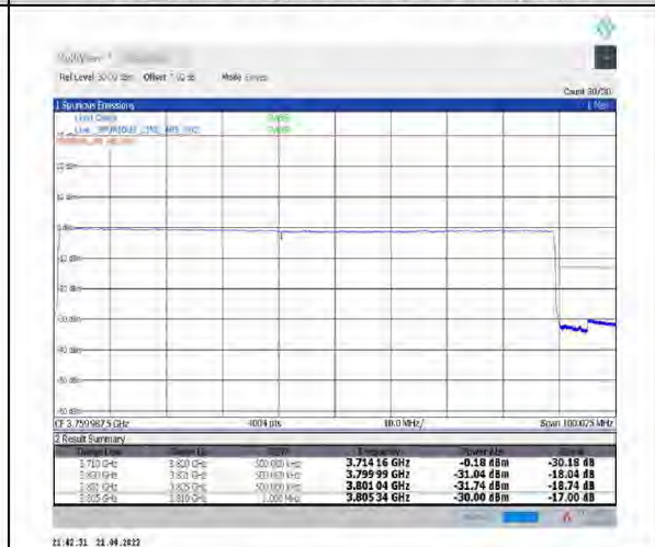
1-N78-3700-3800--30-90-H-6-CP-QPSK-Outer_Full-245@0-Ant1-PASS-see graph
