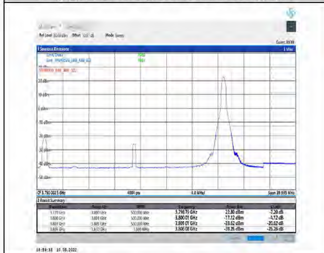
1-N78-3700-3800-PC2-30-30-H-5-CP-QPSK-Edge_1RB_Right-1@77-Ant1-PASS-see graph
