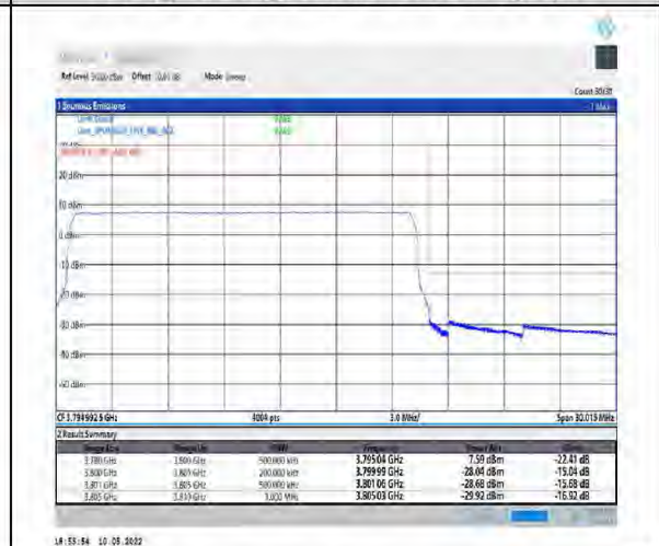
1-N78-3700-3800-PC2-30-20-H-6-CP-QPSK-Outer_Full-51@0-Ant1-PASS-see graph
