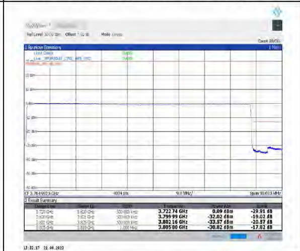
1-N78-3700-3800--30-80-H-6-CP-QPSK-Outer_Full-217@0-Ant1-PASS-see graph
