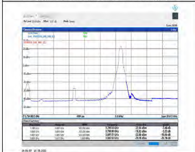
1-N78-3700-3800-PC2-30-20-H-5-CP-QPSK-Edge_1RB_Right-1@50-Ant1-PASS-see graph
