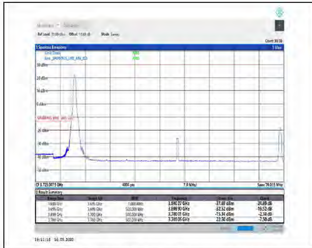
1-N78-3700-3800-PC2-30-60-L-4-CP-QPSK-Edge_1RB_Left-1@0-Ant1-PASS-see graph
