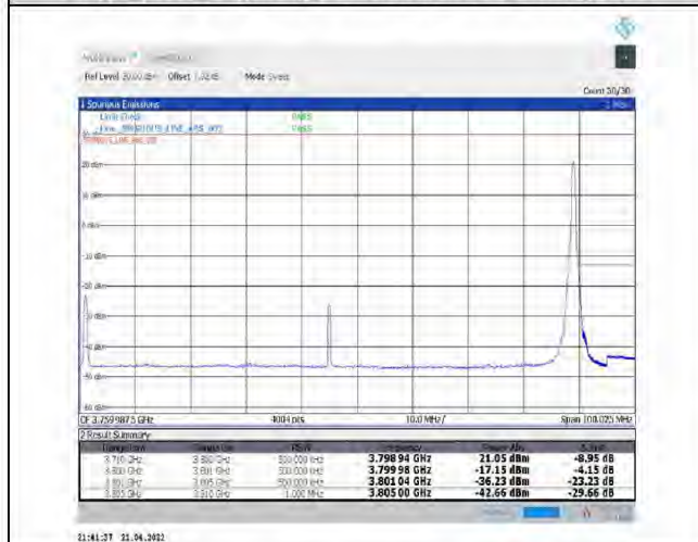
1-N78-3700-3800--30-90-H-5-CP-QPSK-Edge_1RB_Right-1@244-Ant1-PASS-see graph
