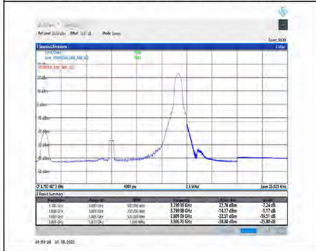
1-N78-3700-3800-PC2-30-15-H-5-CP-QPSK-Edge_1RB_Right-1@37-Ant1-PASS-see graph
