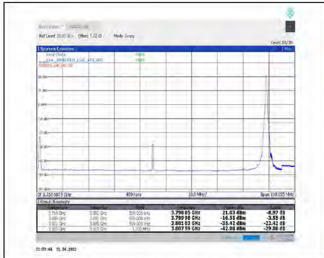
1-N78-3700-3800--30-90-H-2-DFT-PI2BPSK-Edge_1RB_Right-1@244-Ant1-PASS-see graph
