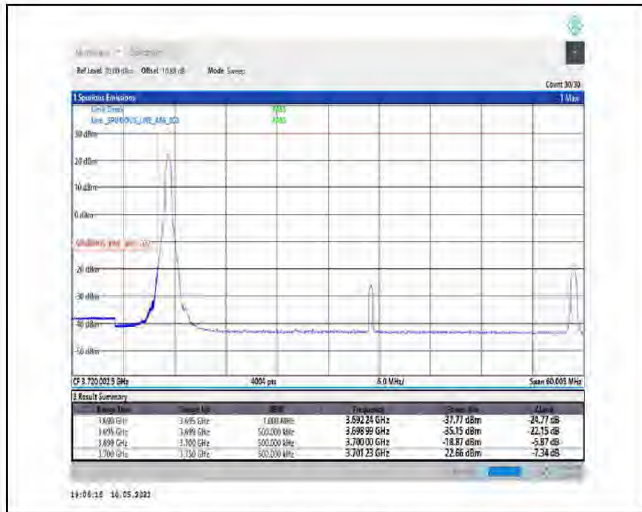
1-N78-3700-3800-PC2-30-50-L-4-CP-QPSK-Edge_1RB_Left-1@0-Ant1-PASS-see graph
