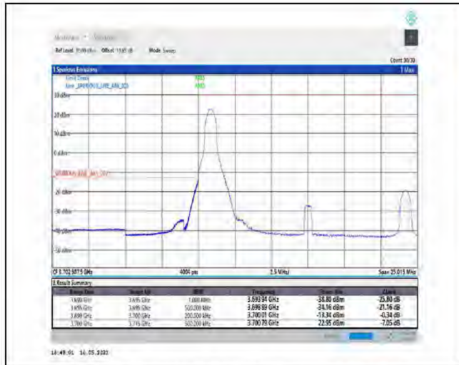
1-N78-3700-3800-PC2-30-15-L-4-CP-QPSK-Edge_1RB_Left-1@0-Ant1-PASS-see graph
