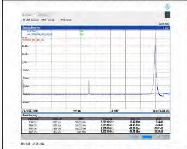
1-N78-3700-3800-PC2-30-100-H-5-CP-QPSK-Edge_1RB_Right-1@272-Ant1-PASS-see graph
