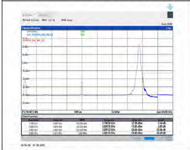
1-N78-3700-3800-PC2-30-40-H-5-CP-QPSK-Edge_1RB_Right-1@105-Ant1-PASS-see graph
