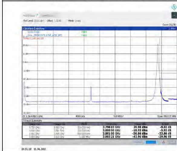
1-N78-3700-3800--30-80-H-5-CP-QPSK-Edge_1RB_Right-1@216-Ant1-PASS-see graph
