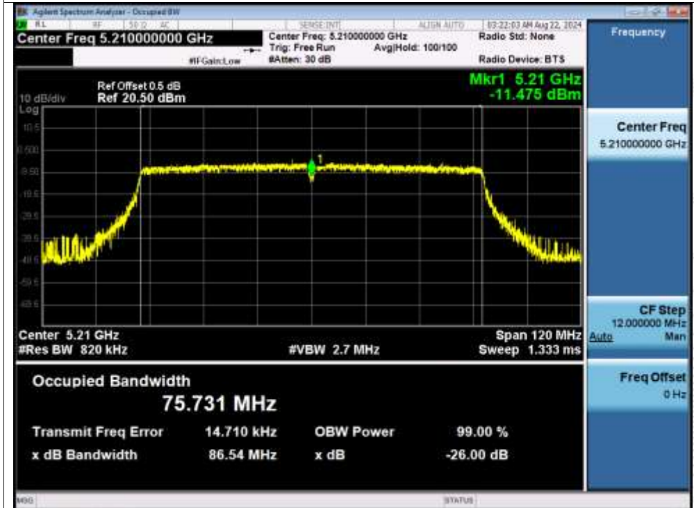
-26dB Bandwidth NVNT ac80 5210MHz
