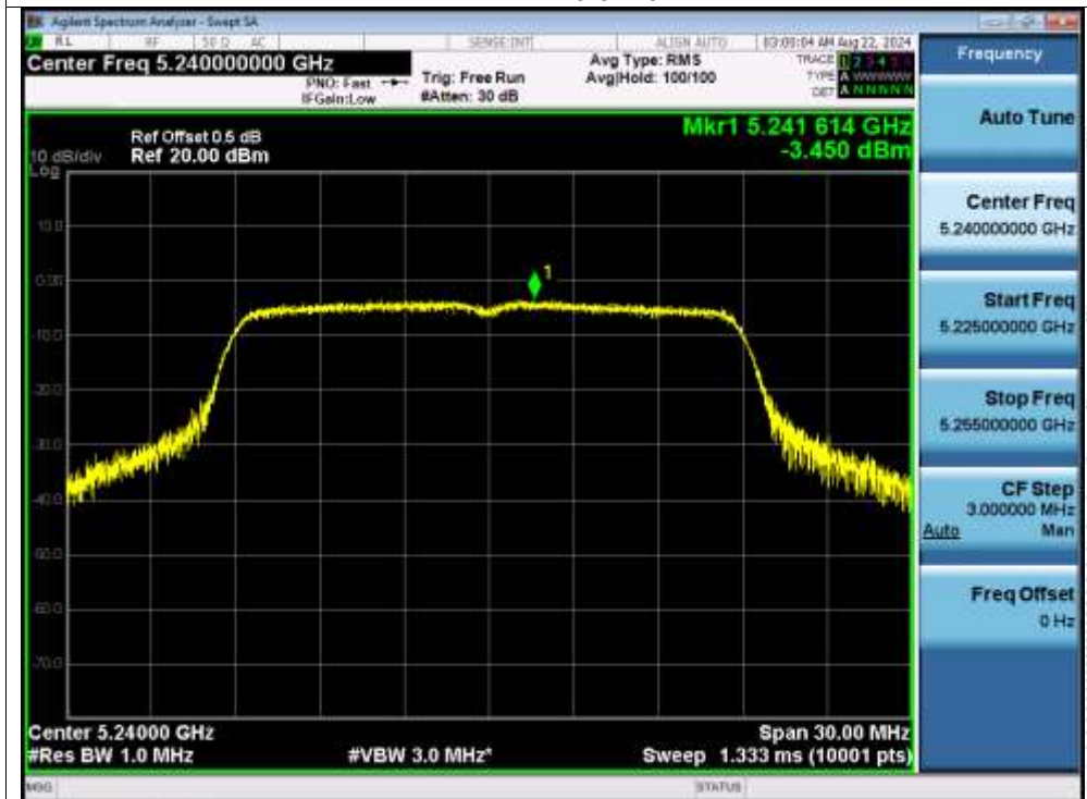
PSD NVNT n20 5240MHz
