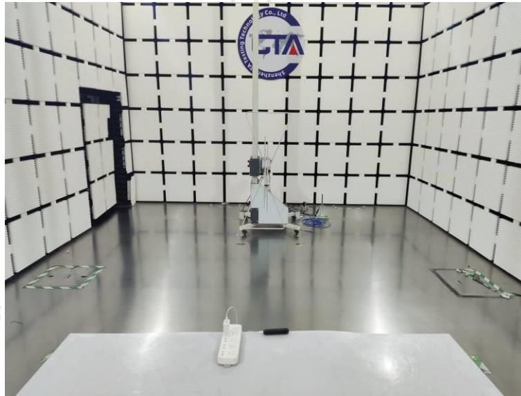
Conducted Disturbance
