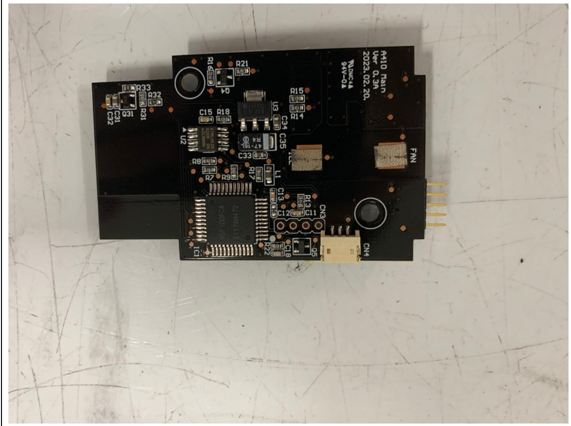
PCB_Rear
