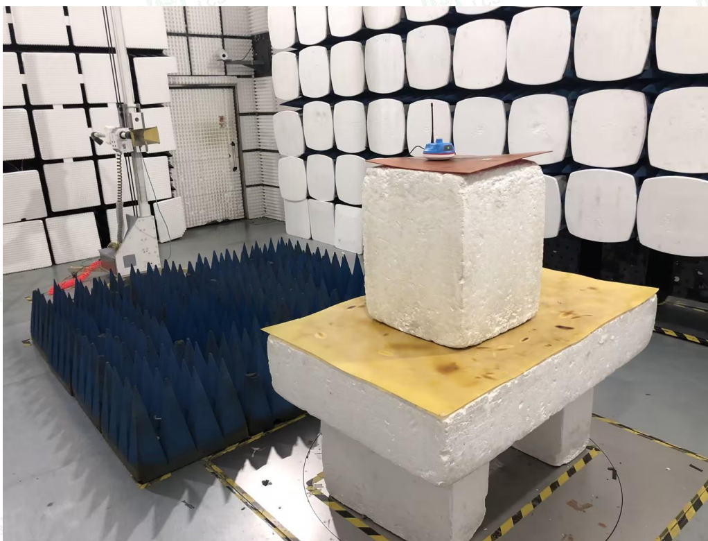
Fig.1 (below 1GHz)
