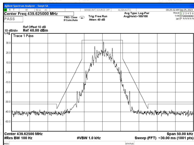
Channel 80 / 439.625 MHz
