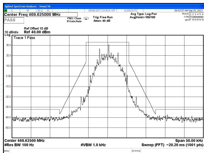
Channel 20 / 469.625 MHz
