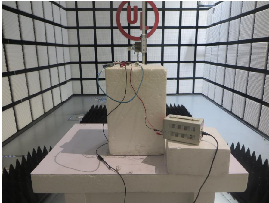
MEASUREMENT POSITION (X axis) - External antenna
