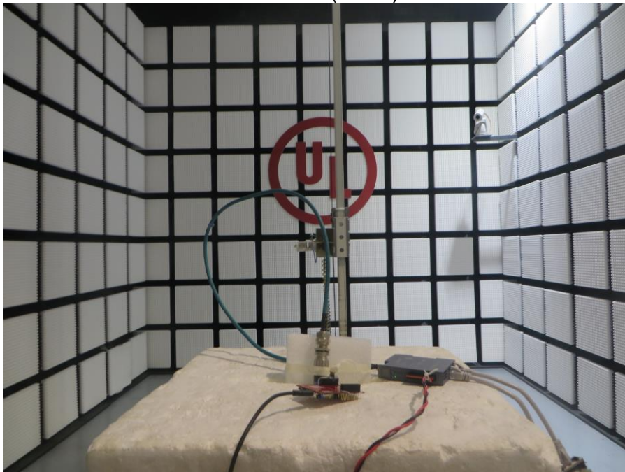
MEASUREMENT POSITION (Z axis) - External antenna
