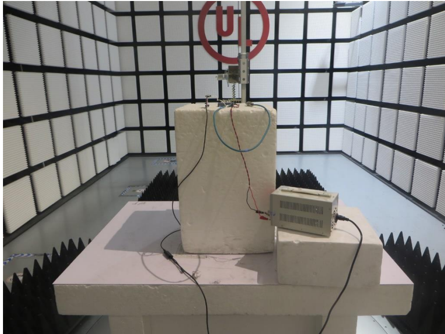
RADIATED RF MEASUREMENT SETUP (ABOVE 1 GHz) MEASUREMENT POSITION - Internal antenna
