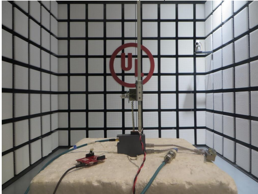
MEASUREMENT POSITION (Z axis) - Internal antenna
