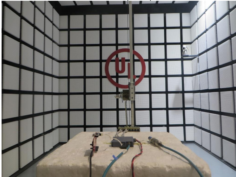
MEASUREMENT POSITION (X axis) - Internal antenna
