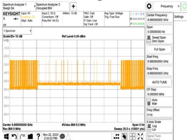
FMCW_150MHz_CF 6570MHz_Interference_6680MHz_ -67.87dBm_ON
