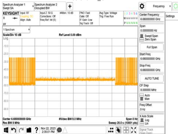
FMCW_150MHz_CF 6570MHz_Interference_6680MHz_ -66.87dBm_Minimal
