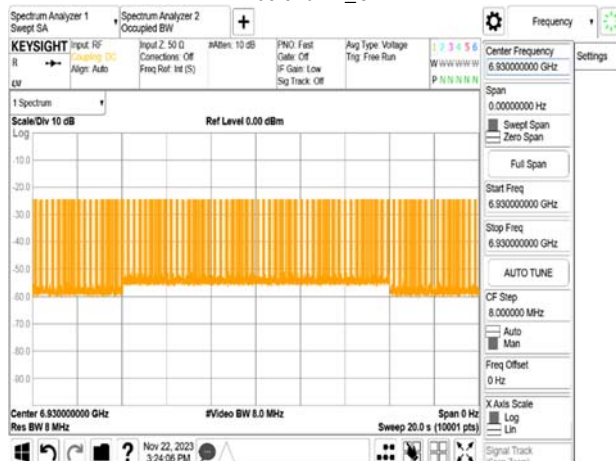
FMCW_150MHz_CF 7000MHz_Interference_6930MHz_ -68.37dBm_ON
