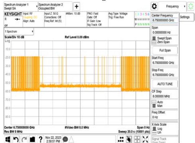
FMCW_150MHz_CF 6750MHz_Interference_6750MHz_ -68.82dBm_ON
