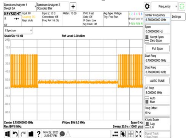
FMCW_150MHz_CF 6750MHz_Interference_6750MHz_ -67.82dBm_Minimal
