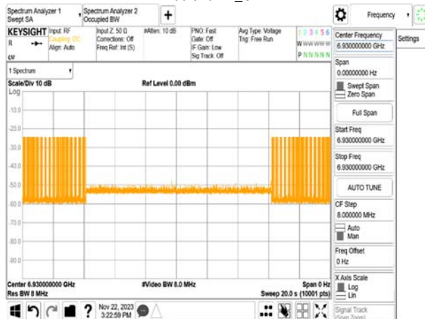
FMCW_150MHz_CF 7000MHz_Interference_6930MHz_ -67.37dBm_Minimal
