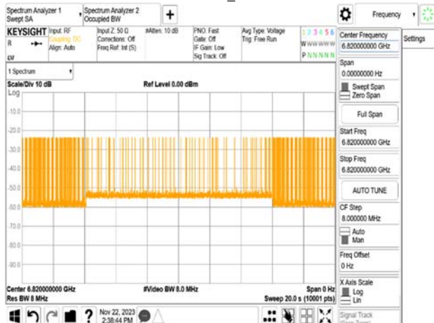
FMCW_150MHz_CF 6750MHz_Interference_6820MHz_ -68.81dBm_ON
