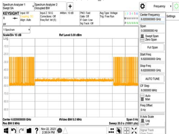
FMCW_150MHz_CF 6750MHz_Interference_6820MHz_ -67.81dBm_Minimal
