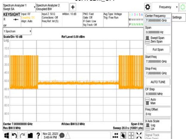
FMCW_150MHz_CF 7000MHz_Interference_7000MHz_ -67.47dBm_Minimal
