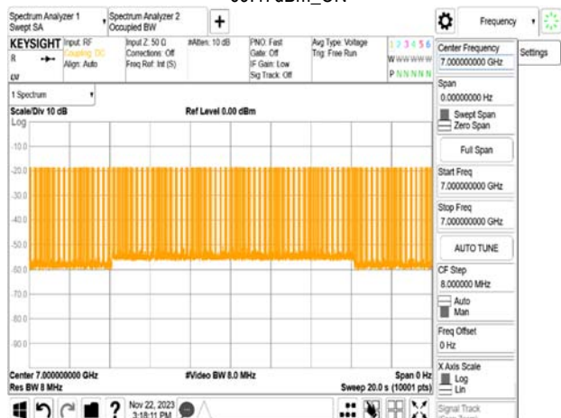
FMCW_150MHz_CF 7000MHz_Interference_7000MHz_ -69.47dBm_ON
