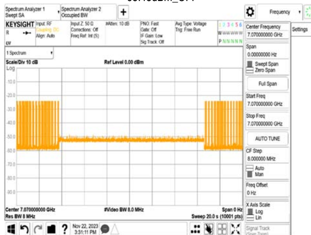
FMCW_150MHz_CF 7000MHz_Interference_7070MHz_ -66.43dBm_Minimal
