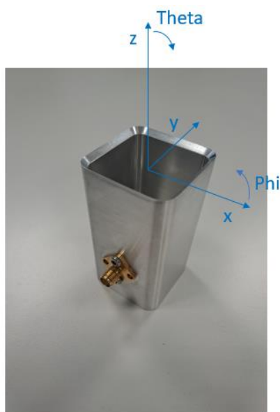
Fig. 1. Photo of measured antenna A-108-061 and coordinate system.
