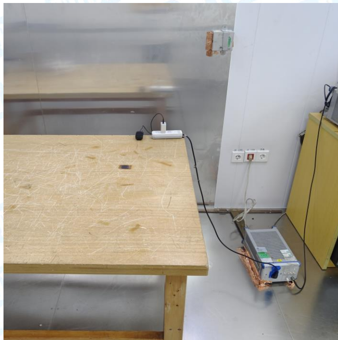
Photo of Setup for Conducted Emission
