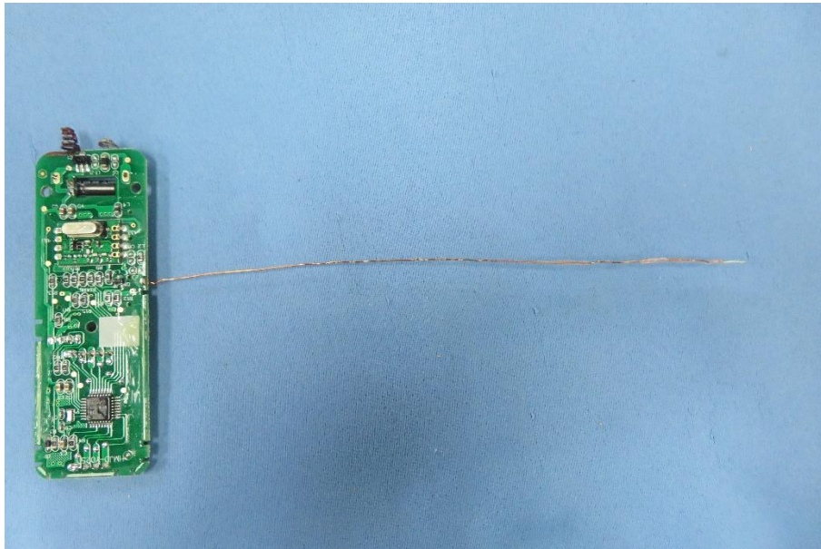
Antenna length:70mm
