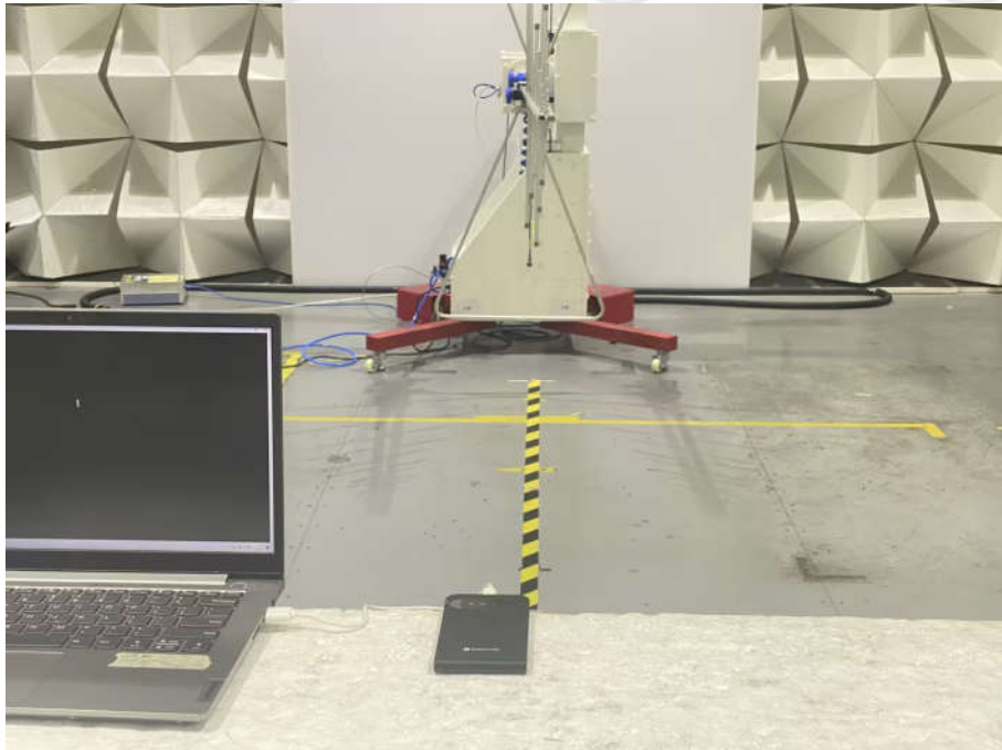
Radiated spurious emission Test Setup-1(Below 1GHz)close up
