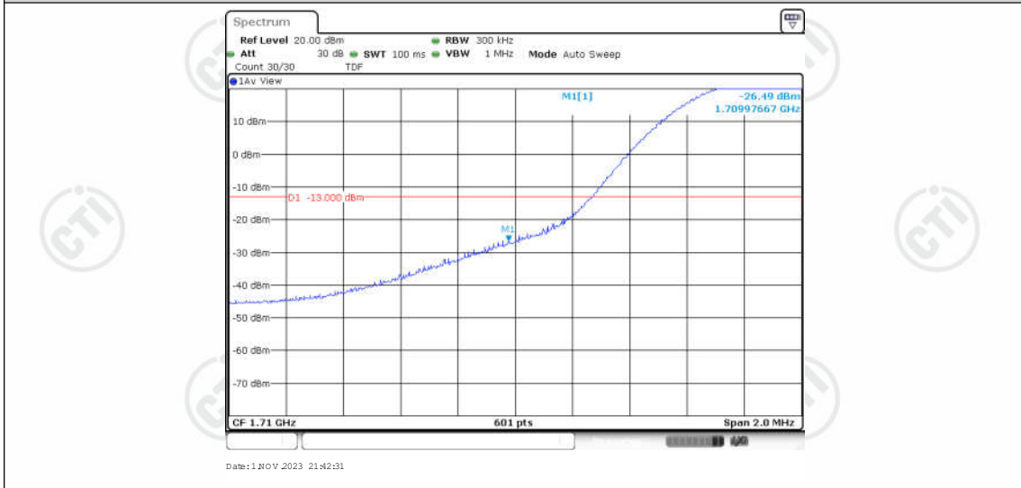
Band66-15MHz-16QAM-132047-1RB#74
