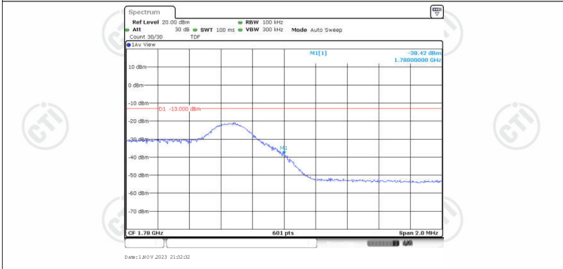
Band66-5MHz-16QAM-132647-1RB#24
