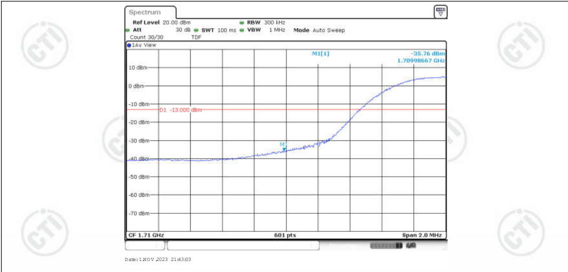
Band66-15MHz-QPSK-132597-1RB#0
