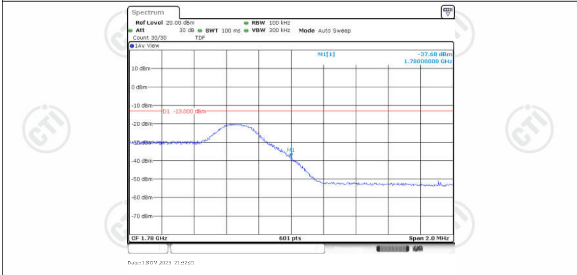
Band66-5MHz-QPSK-132647-1RB#24
