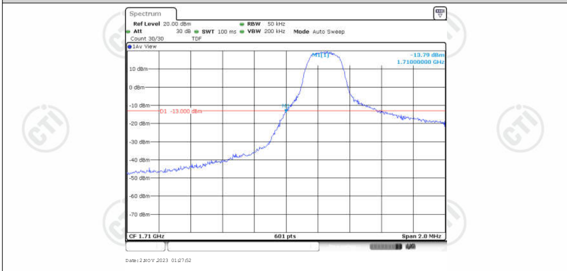
Band66-3MHz-QPSK-131987-1RB#14
