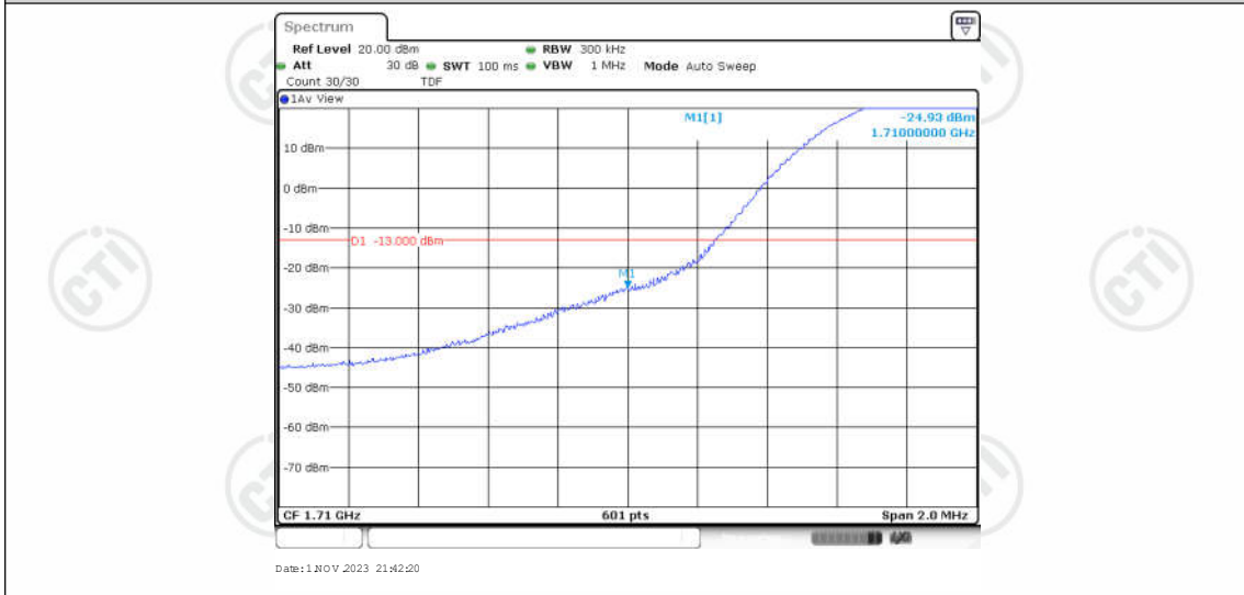
Band66-15MHz-QPSK-132047-1RB#74
