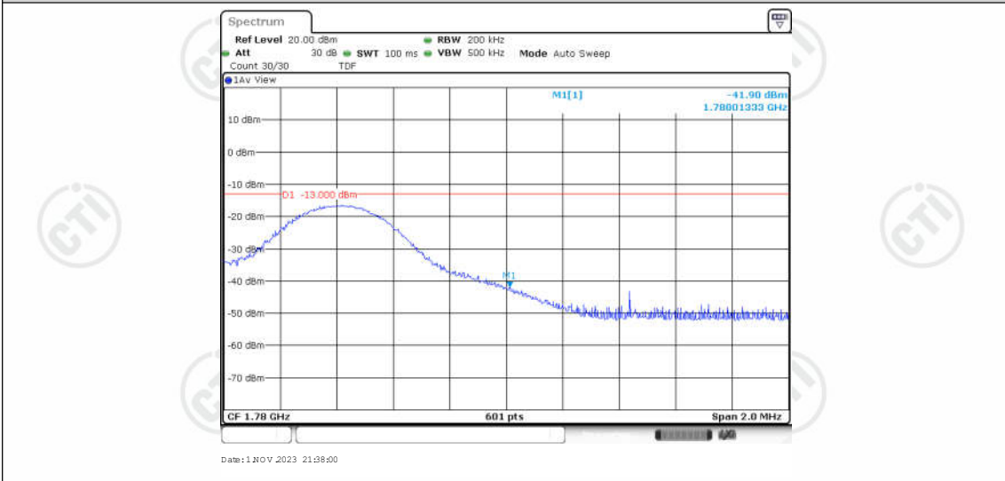
Band66-10MHz-QPSK-132622-1RB#49
