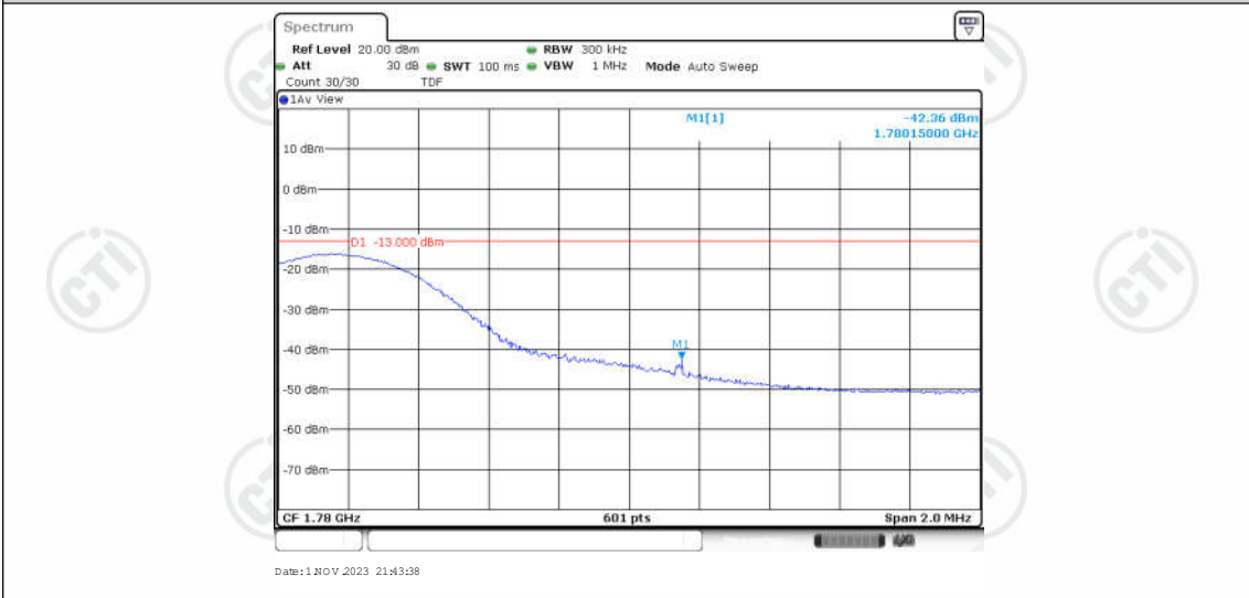
Band66-15MHz-QPSK-132597-1RB#74
