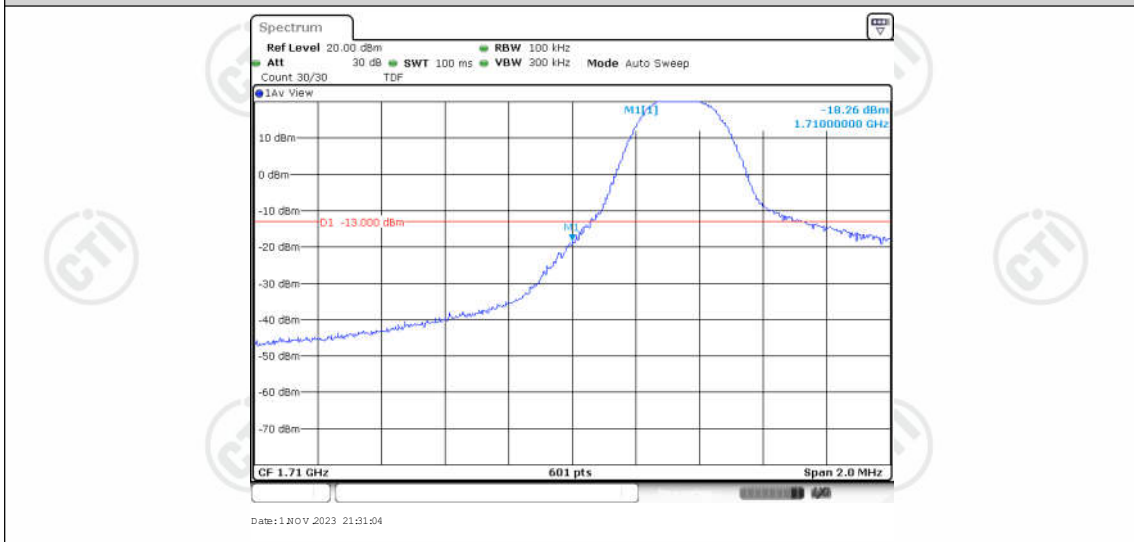
Band66-5MHz-QPSK-131997-1RB#24
