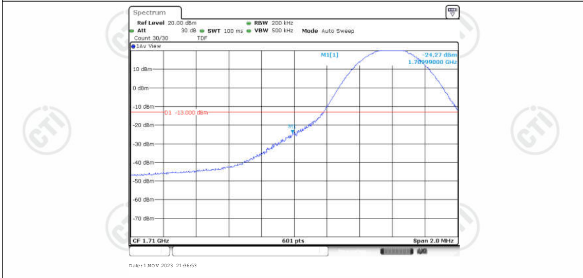
Band66-10MHz-16QAM-132022-1RB#49
