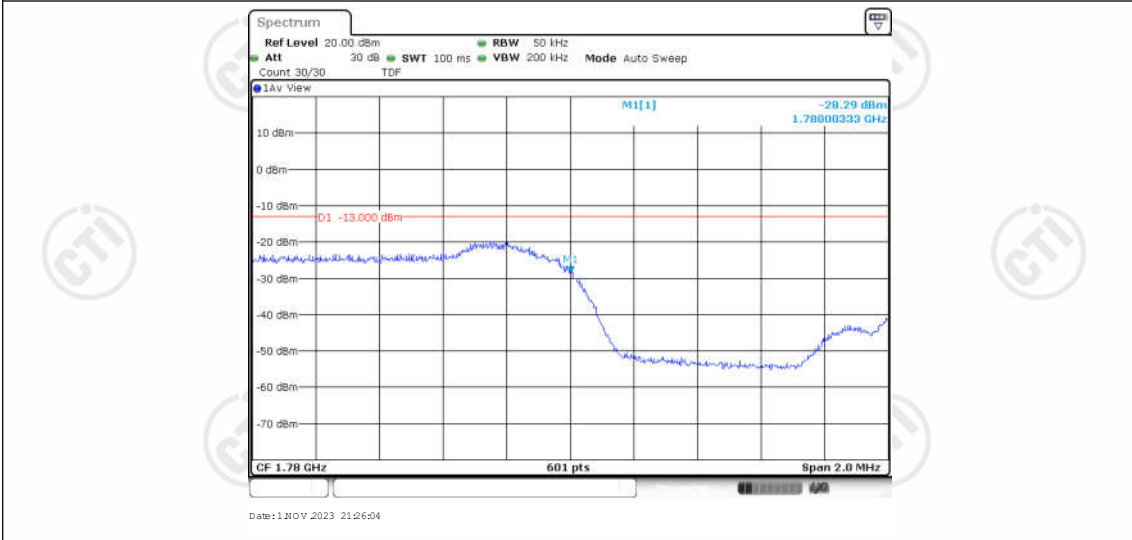
Band66-3MHz-QPSK-132657-1RB#14
