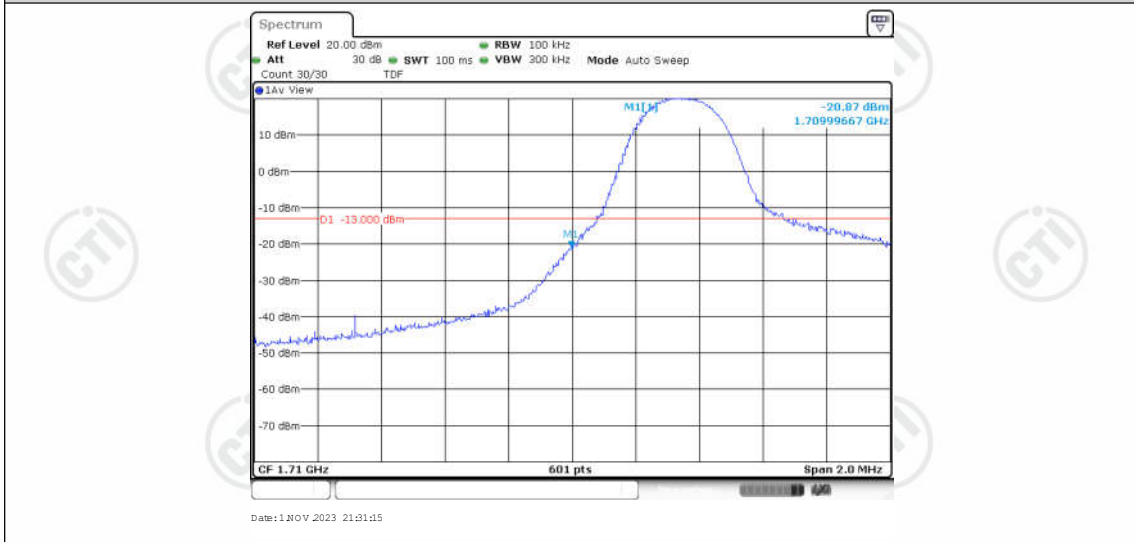
Band66-5MHz-16QAM-131997-1RB#24
