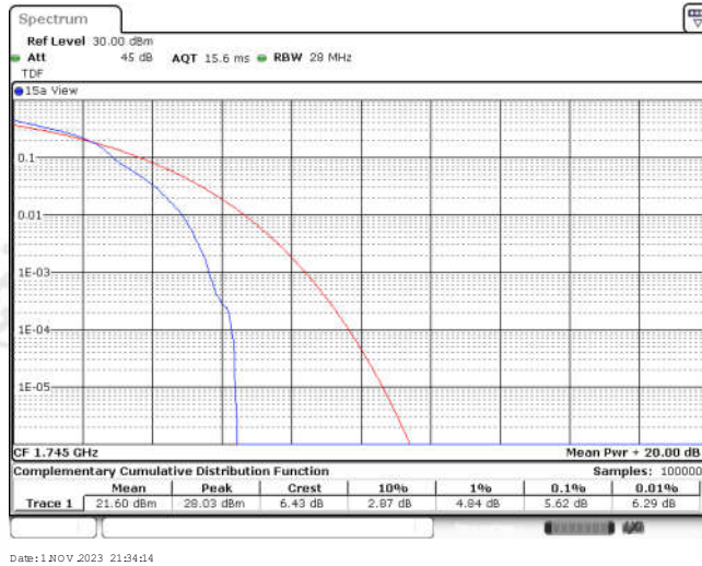
Band66-5MHz-16QAM-132322-25RB#0
