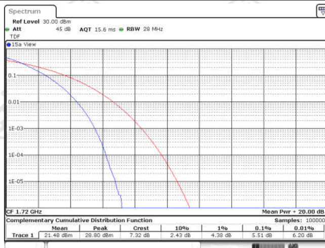
Band66-20MHz-QPSK-132072-100RB#0
