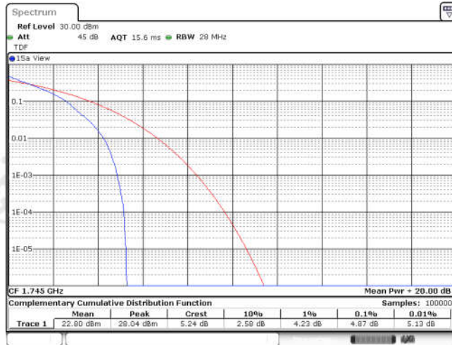
Band66-5MHz-QPSK-132322-25RB#0
