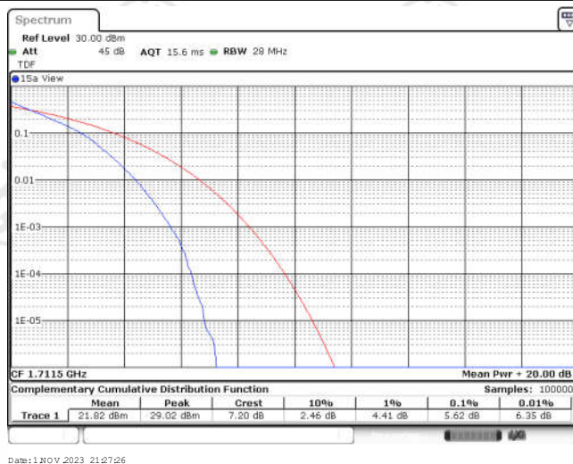
Band66-3MHz-QPSK-132322-1RB#0
