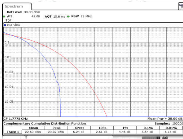
Band66-5MHz-QPSK-132647-1RB#0
