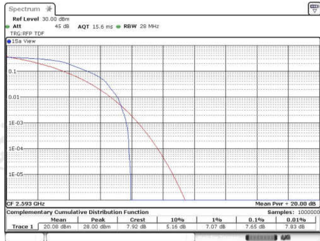
Band41-5MHz-16QAM-40620-25RB#0
