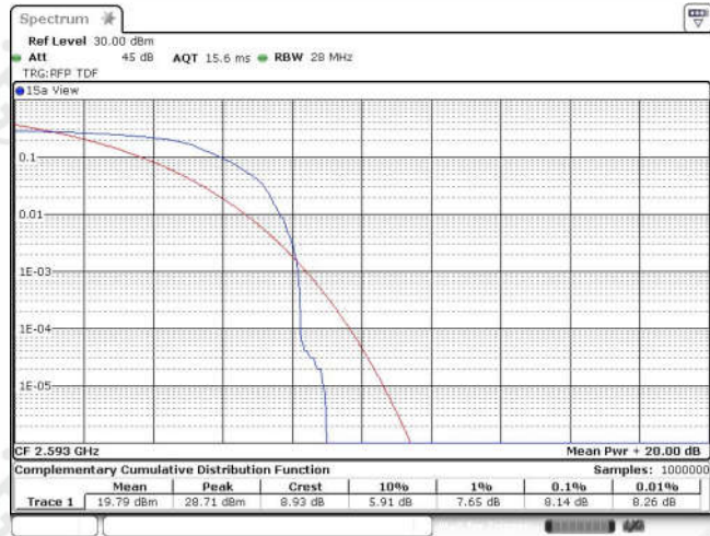
Band41-10MHz-16QAM-40620-50RB#0
