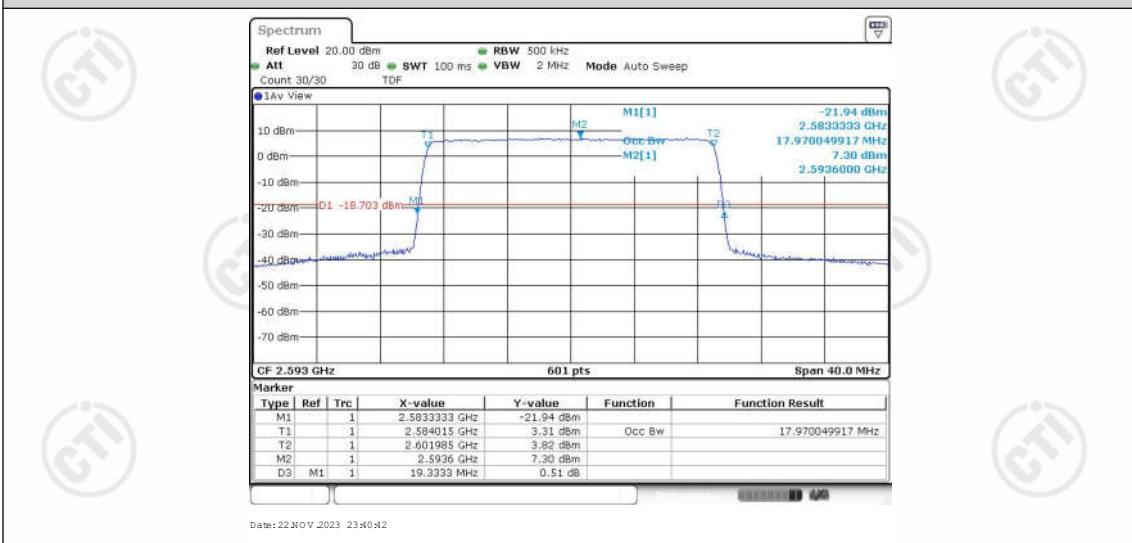
Band41-20MHz-16QAM-41490-100RB#0-17.97
