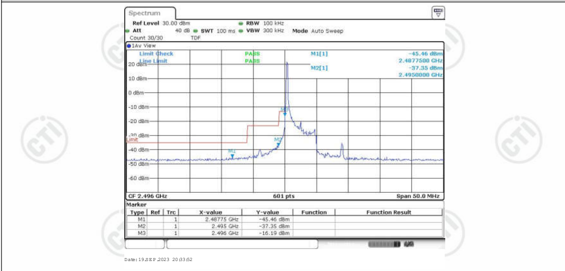
Band41-5MHz-16QAM-39675-1RB#24
