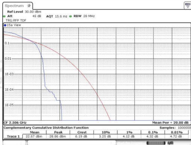
Band41-20MHz-16QAM-39750-100RB#0
