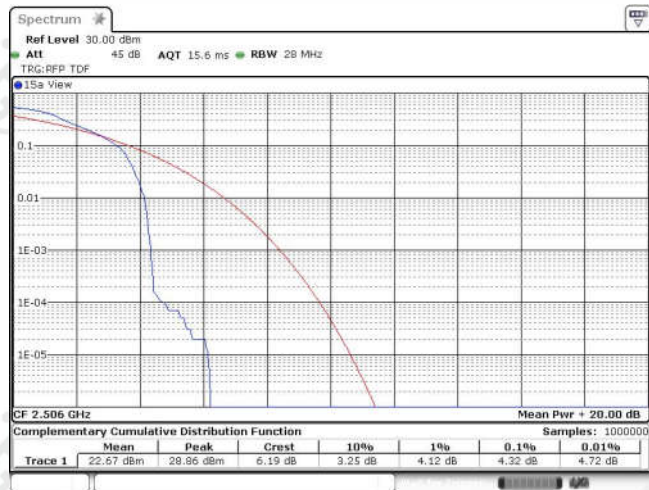
Band41-20MHz-QPSK-39750-1RB#0
