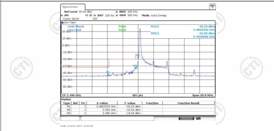
Band41-10MHz-16QAM-39700-1RB#49
