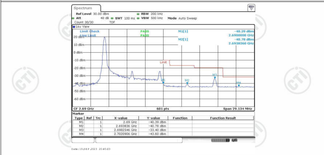
Band41-10MHz-QPSK-41540-1RB#49
