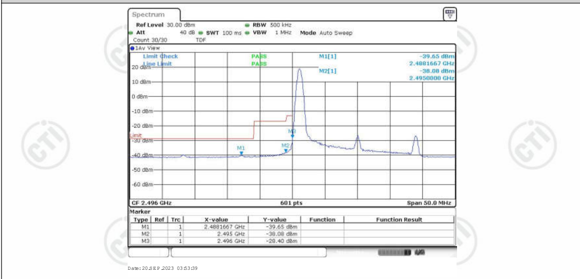
Band41-20MHz-16QAM-39750-1RB#99
