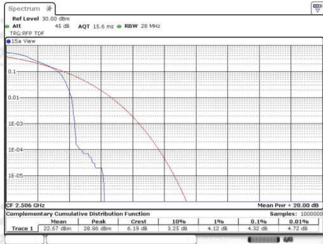
Band41-20MHz-16QAM-39750-1RB#0
