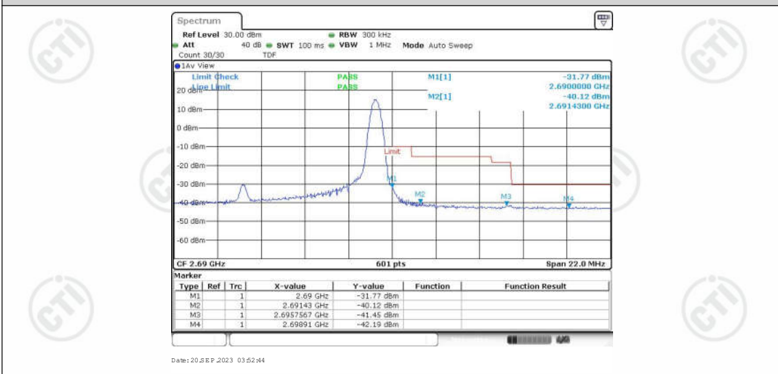
Band41-15MHz-16QAM-41515-75RB#0
