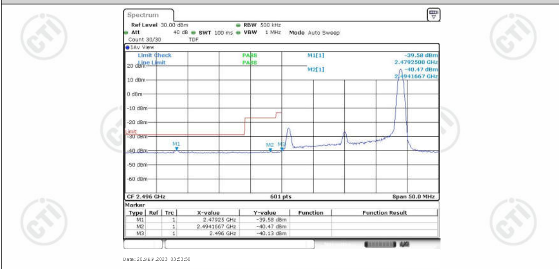
Band41-20MHz-QPSK-39750-100RB#0
