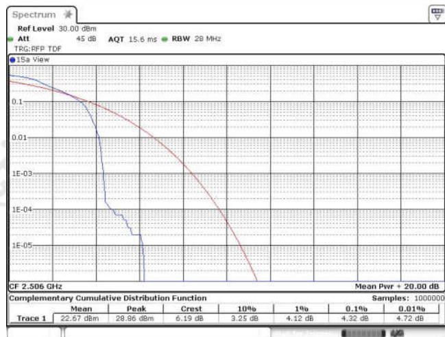
Band41-20MHz-QPSK-39750-100RB#0
