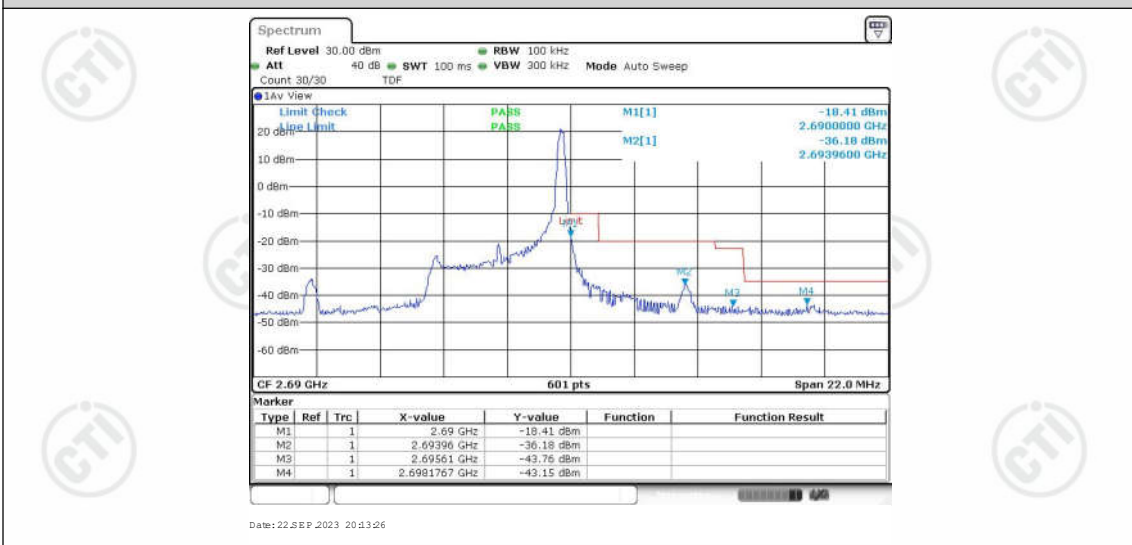
Band41-5MHz-QPSK-41565-25RB#0
