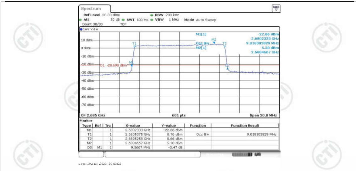
Band41-10MHz-16QAM-41540-50RB#0-9.018
