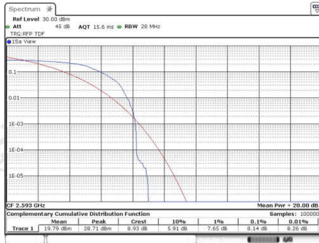
Band41-10MHz-QPSK-40620-50RB#0
