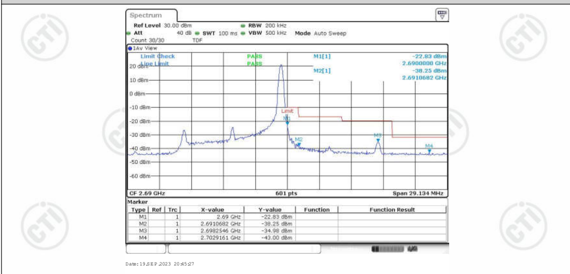
Band41-10MHz-QPSK-41540-50RB#0
