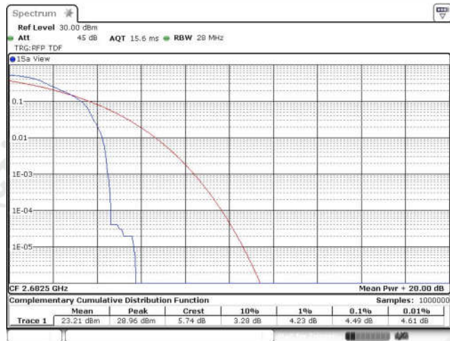
Band41-15MHz-QPSK-41515-1RB#0
