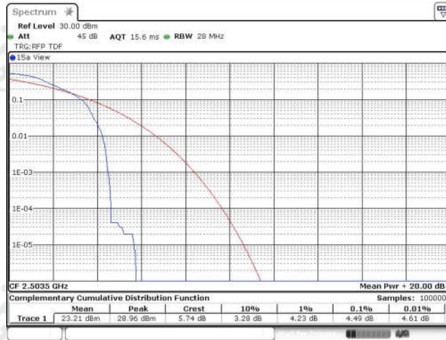
Band41-15MHz-QPSK-39725-1RB#0
