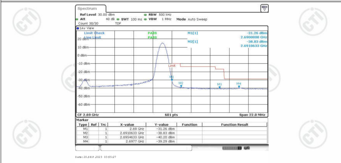
Band41-20MHz-16QAM-41490-100RB#0
