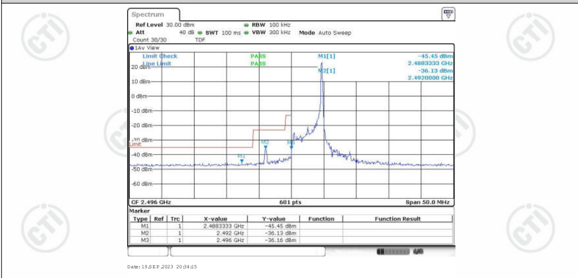
Band41-5MHz-16QAM-39675-25RB#0
