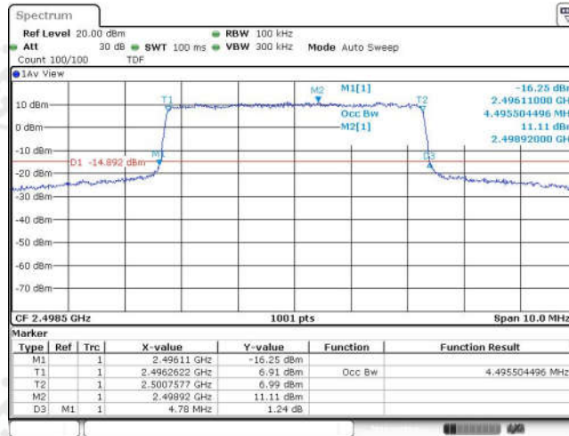
Band41-5MHz-QPSK-39675-25RB#0-4.496
