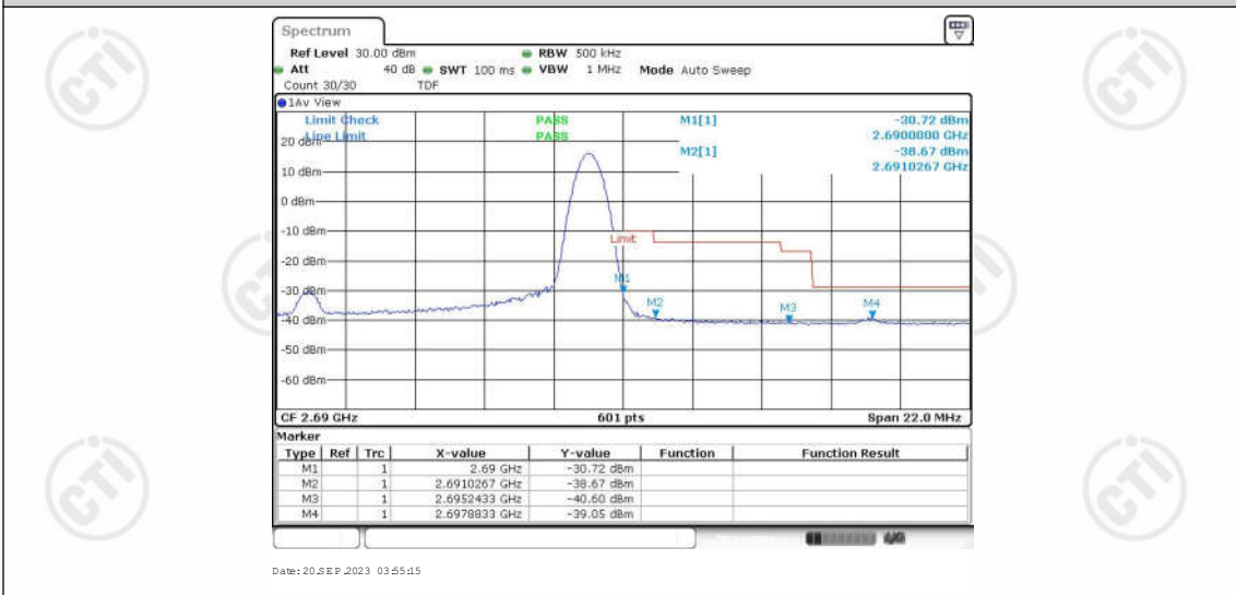
Band41-20MHz-QPSK-41490-100RB#0
