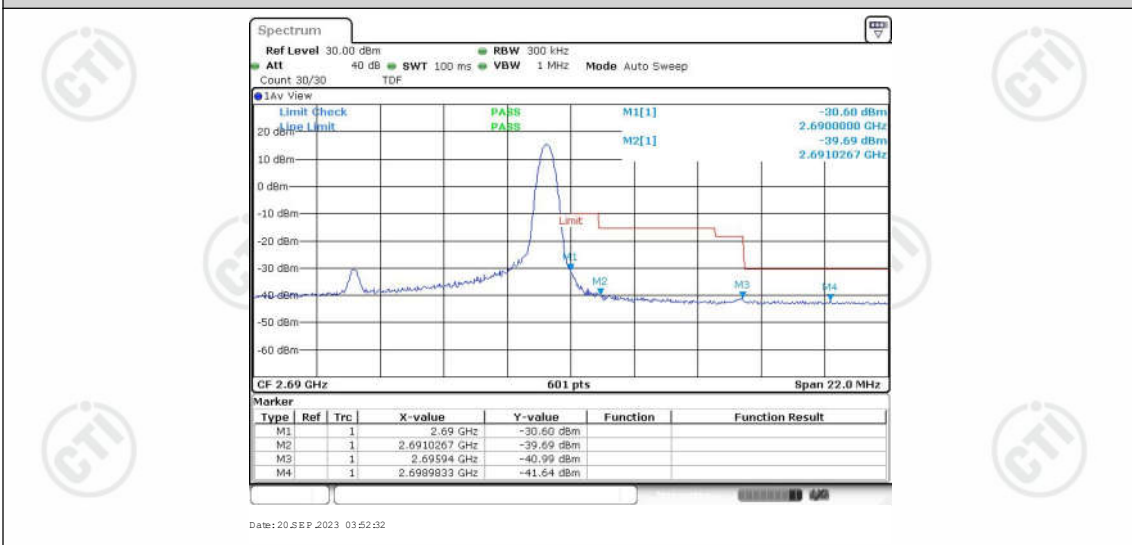
Band41-15MHz-QPSK-41515-75RB#0
