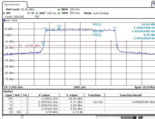
Band41-5MHz-QPSK-40620-25RB#0-4.496
