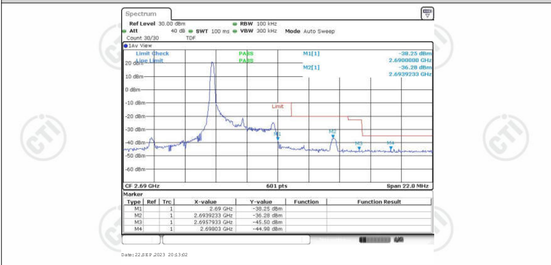
Band41-5MHz-QPSK-41565-1RB#24
