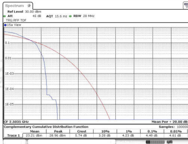
Band41-15MHz-QPSK-39725-75RB#0
