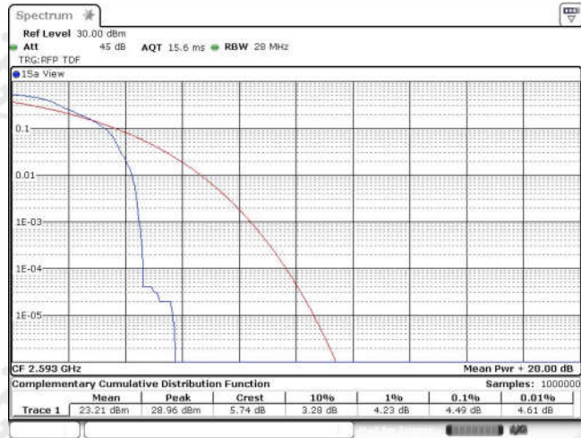
Band41-15MHz-QPSK-40620-75RB#0
