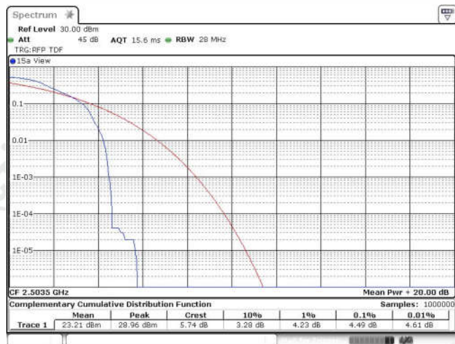
Band41-15MHz-16QAM-39725-75RB#0
