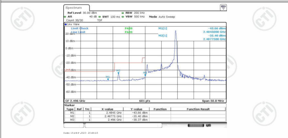
Band41-10MHz-16QAM-39700-50RB#0
