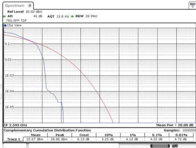
Band41-20MHz-16QAM-40620-100RB#0
