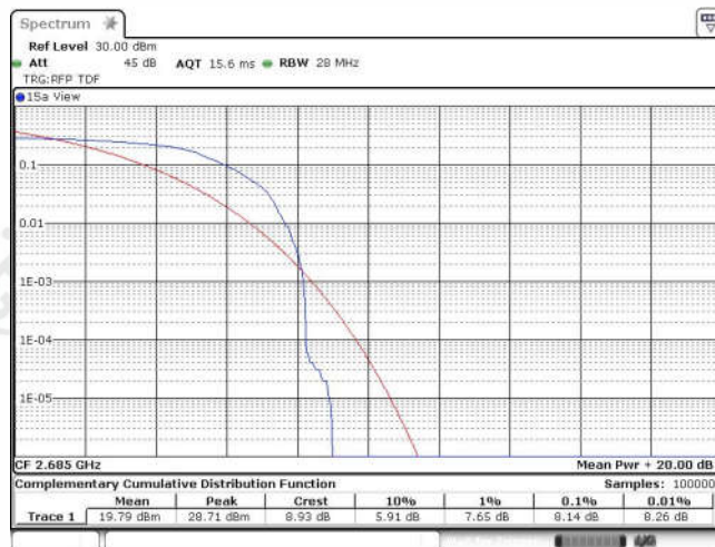
Band41-10MHz-QPSK-41540-1RB#0
