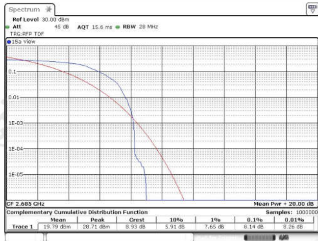
Band41-10MHz-16QAM-41540-1RB#0
