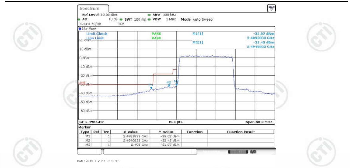
Band41-15MHz-16QAM-41515-1RB#0
