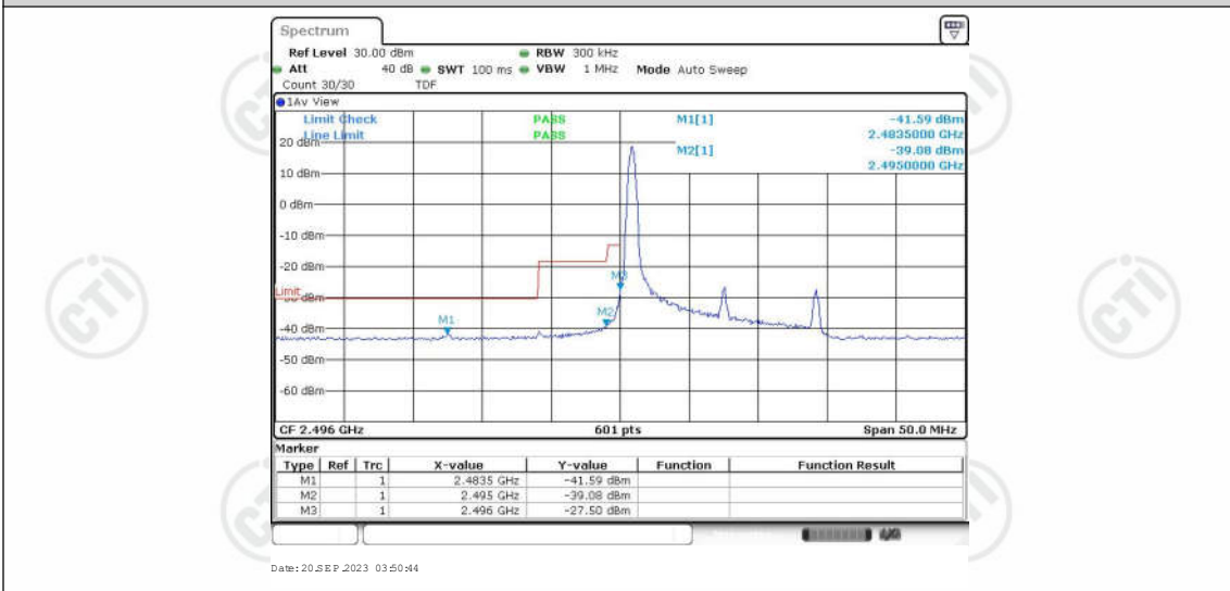
Band41-15MHz-QPSK-39725-1RB#74
