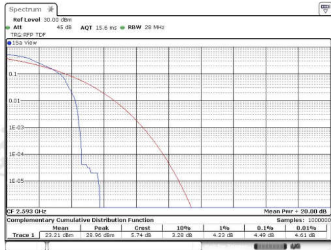
Band41-15MHz-16QAM-40620-75RB#0
