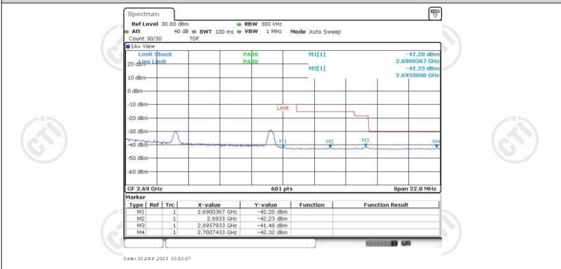
Band41-15MHz-QPSK-41515-1RB#74
