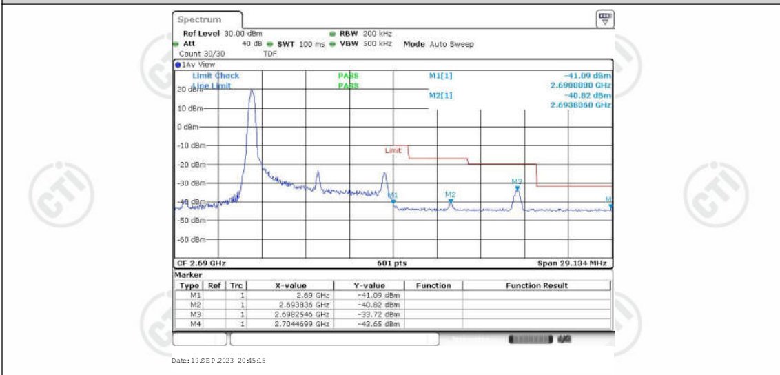
Band41-10MHz-16QAM-41540-1RB#49
