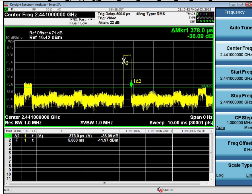
Dwell_Time_(Hopping)_NVNT_ANT1_1-DH1_2441_One_Burst_Time
